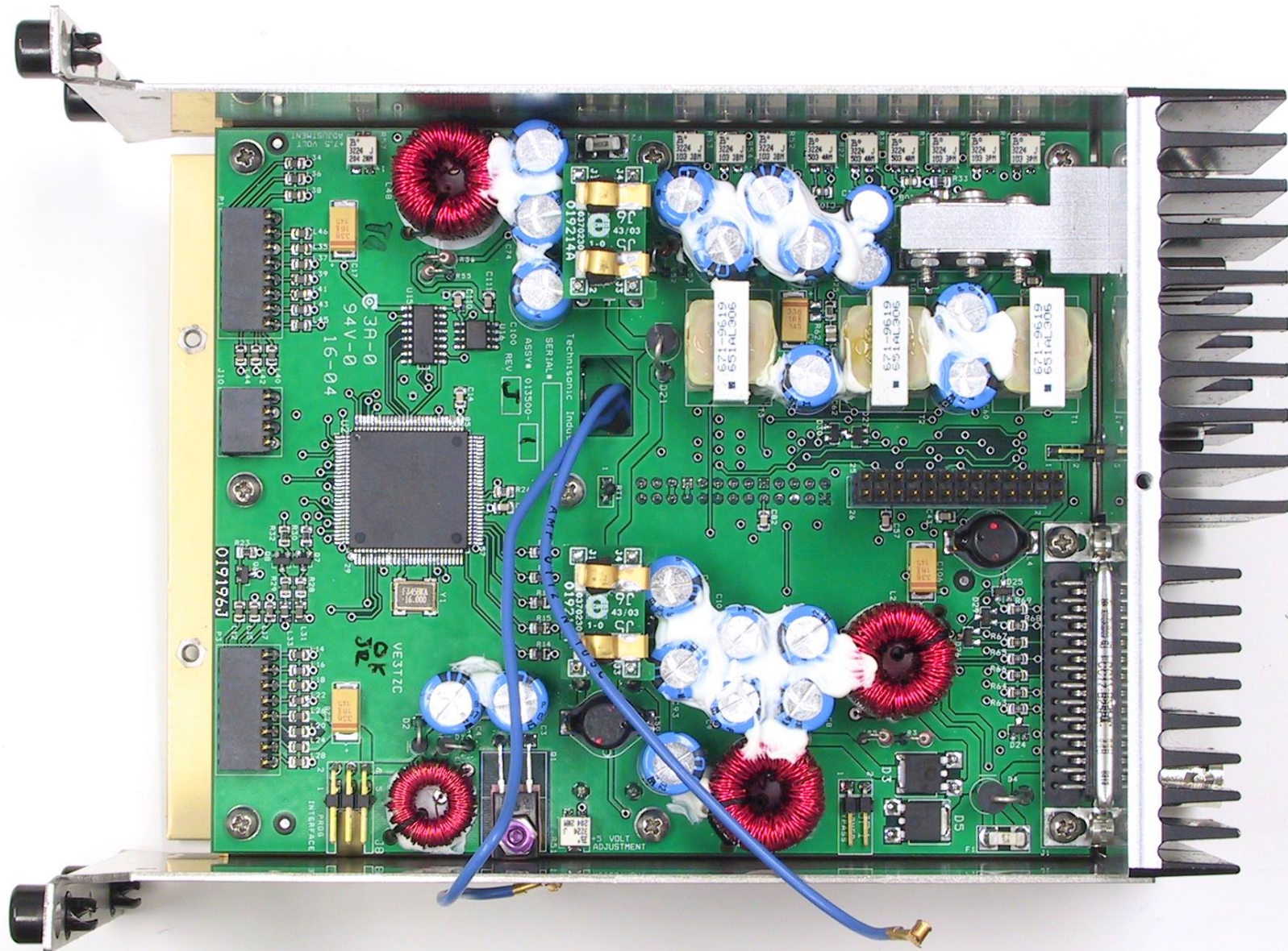
Annex 3 – Internal Photographs of EUT VHF P25 Airborne Transceiver, Model No.: TDFM-636
