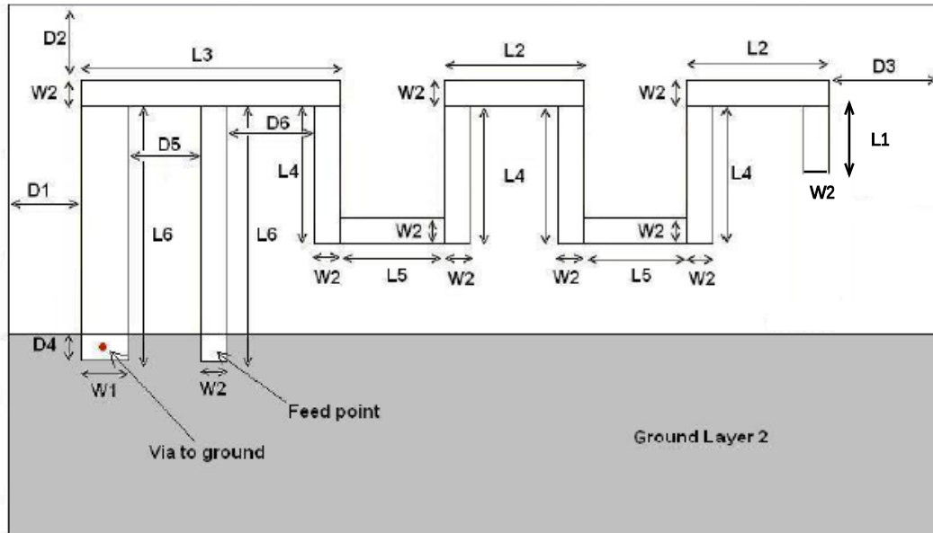
Figure 3: Antenna Dimensions
