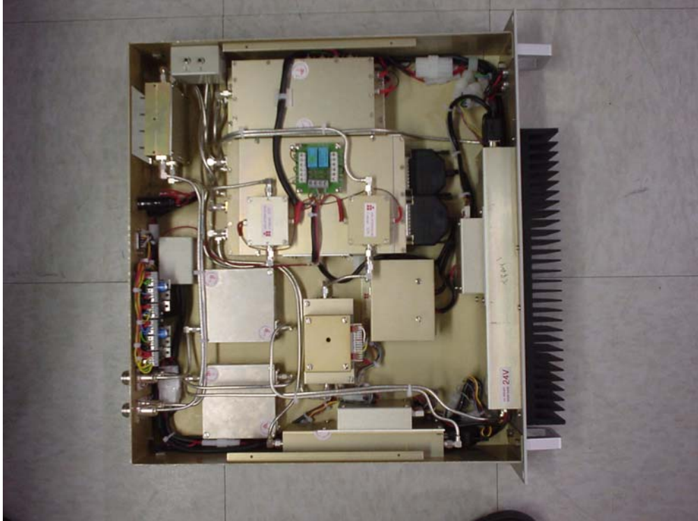
VHF Channelized Module (Simplex)
