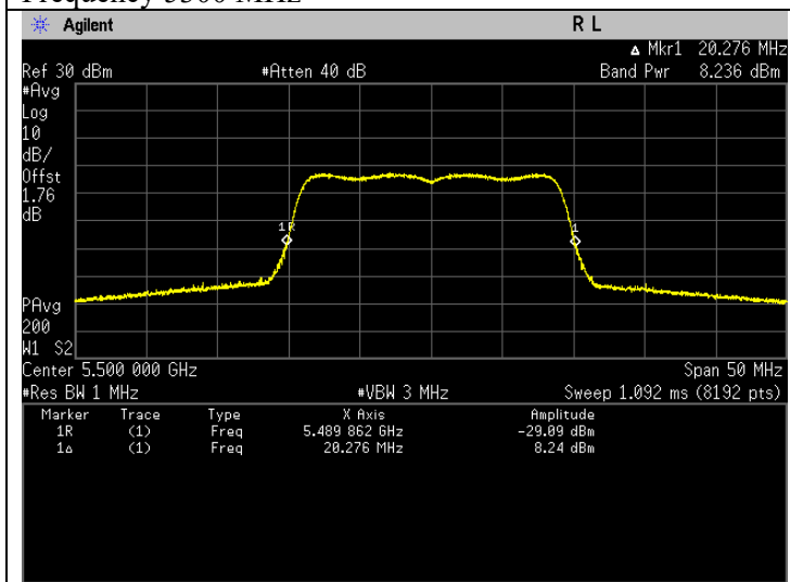
Frequency 5500 MHz
