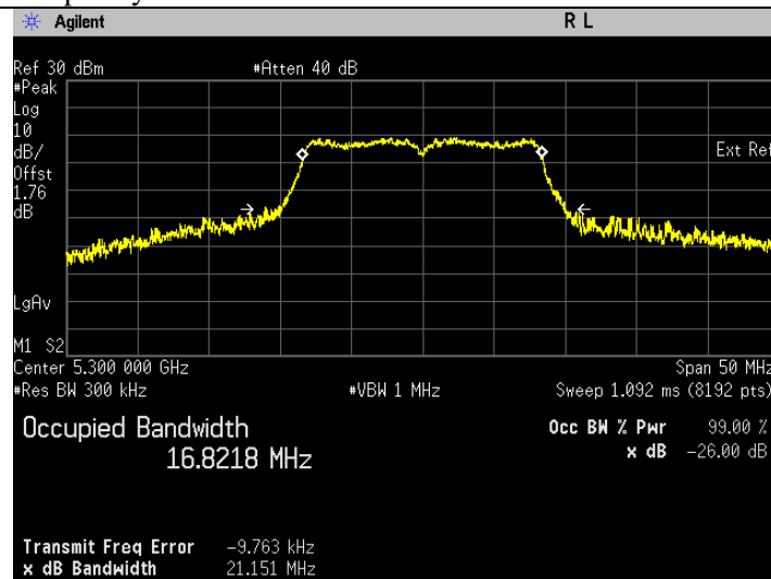
Frequency 5300 MHz
