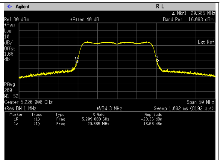
Frequency 5220 MHz
