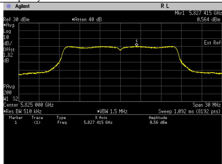
Frequency 5825 MHz
