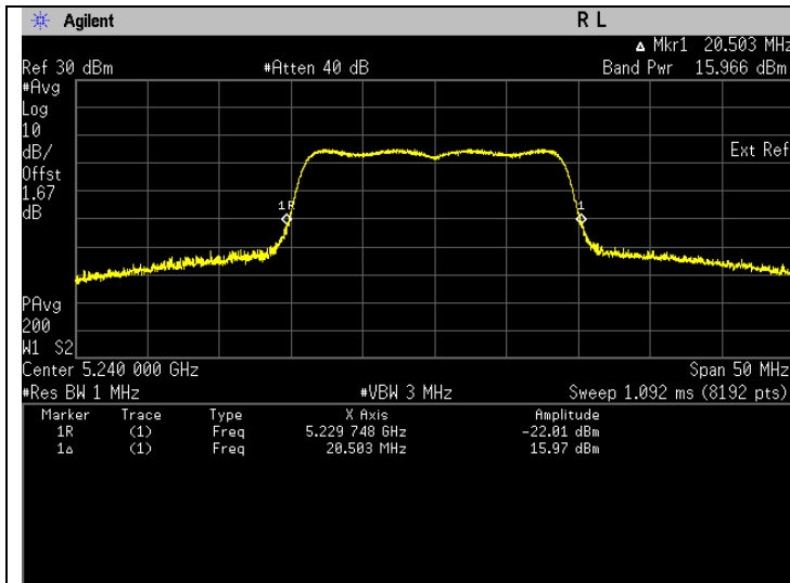
Frequency 5240 MHz
