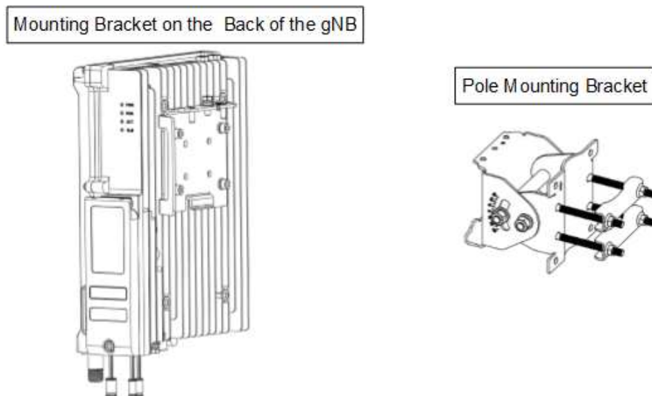
Figure 2-1 Pre-assembled Device
