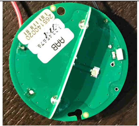
Antenna PCB shown with battery and battery clips removed (Power cables for bench testing only)
