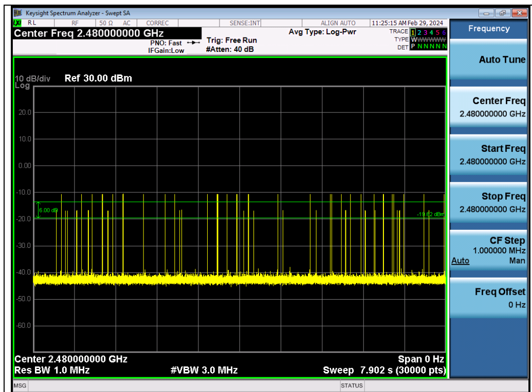
Test Graph EDR HOP ANT1 NA 2Mbps 2480 Number of Busrt
