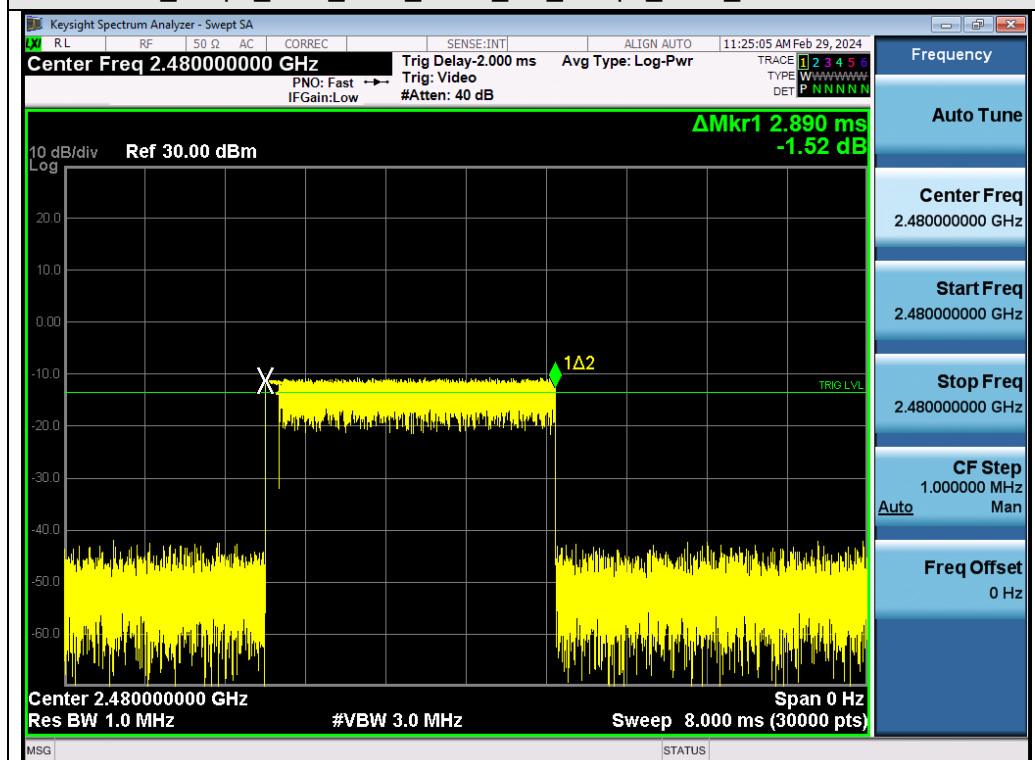
Test Graph EDR HOP ANT1 NA 2Mbps 2480 Time per Burst
