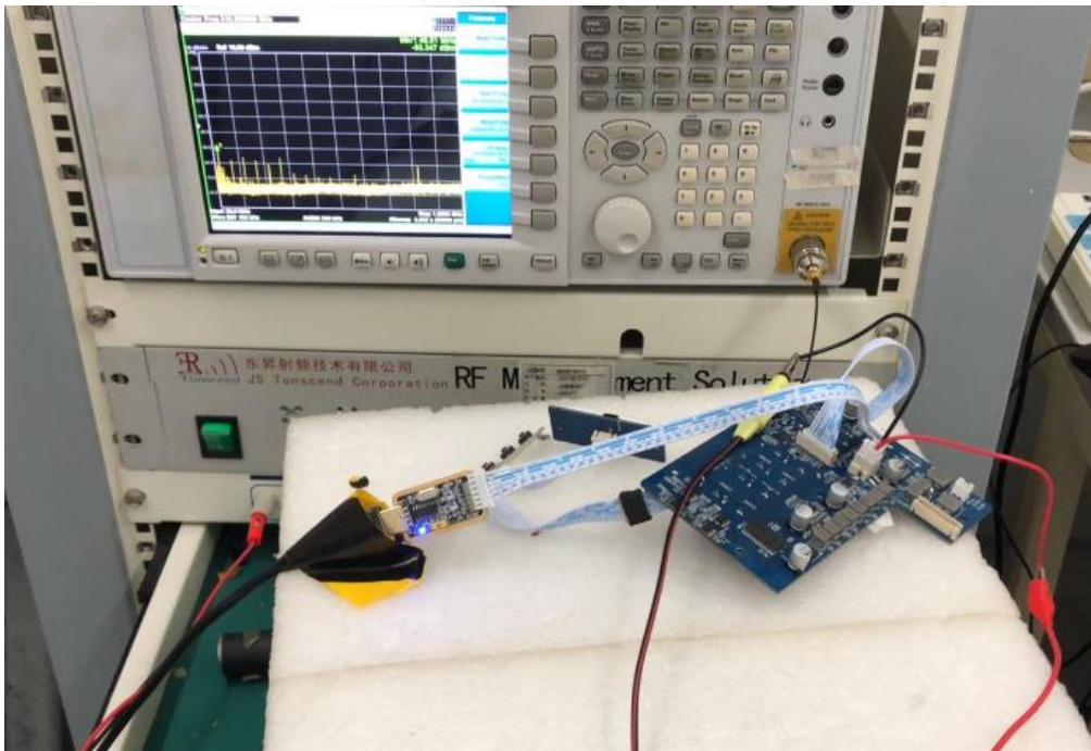
CONDUCTED TEST SETUP
