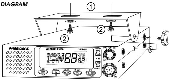
MOUNTING DIAGRAM
