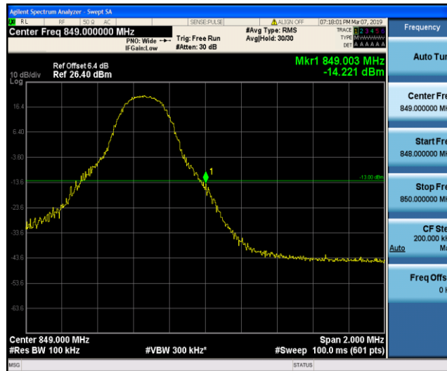
Band5_5MHz_QPSK_20625_1RB#24
