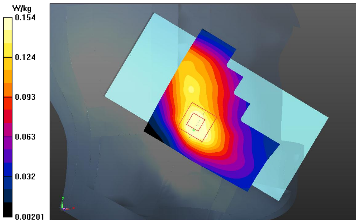
Fig.3 GSM 1900 Head
