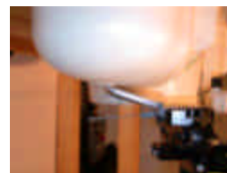
Figure 14.10 Right Head SAR Test Setup -- Ear / Tilt Position --
