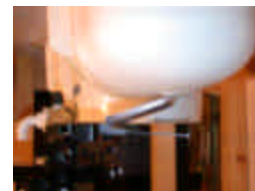
Figure 14.12 Left Head SAR Test Setup -- Ear / Tilt Position --
