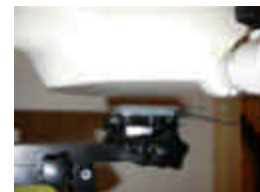
Figure 14.15 Body SAR Test Setup -- w/o Belt-clip --
