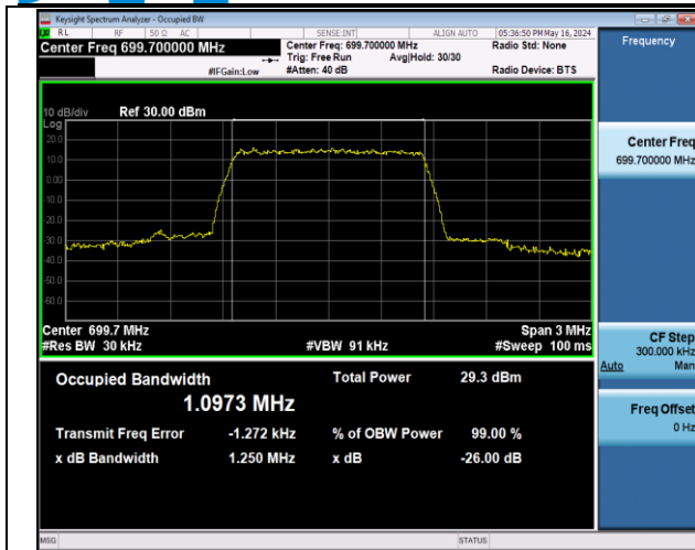
Band12-1.4MHz-QPSK-23017-6RB#0-PASS
