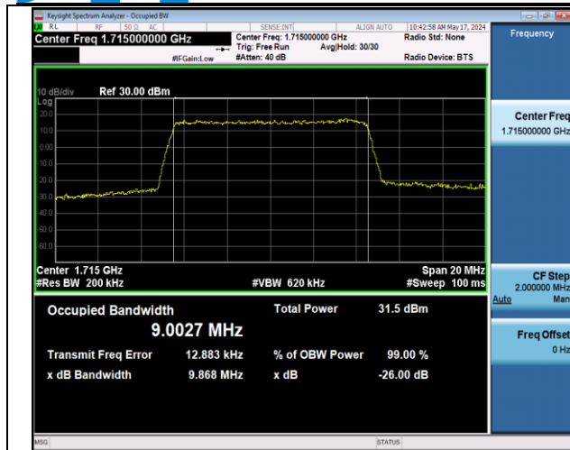
Band66-10MHz-QPSK-132022-50RB#0-PASS
