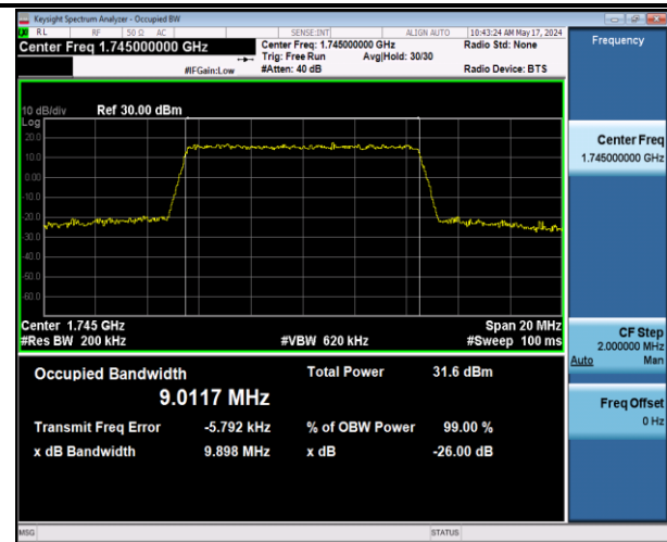
Band66-10MHz-QPSK-132322-50RB#0-PASS
