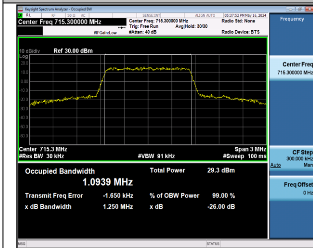
Band12-1.4MHz-QPSK-23173-6RB#0-PASS
