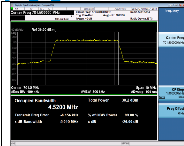
Band12-5MHz-QPSK-23035-25RB#0-PASS
