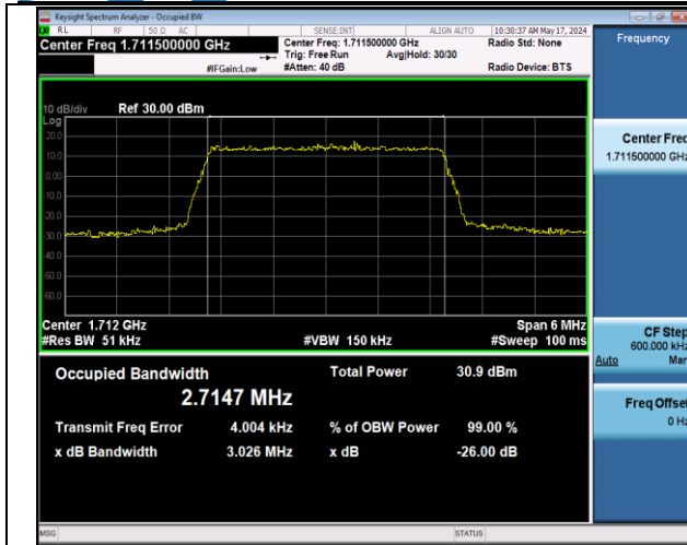
Band66-3MHz-QPSK-131987-15RB#0-PASS
