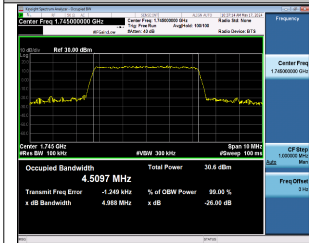
Band66-5MHz-16QAM-132322-25RB#0-PASS
