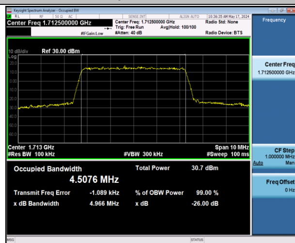
Band66-5MHz-16QAM-131997-25RB#0-PASS
