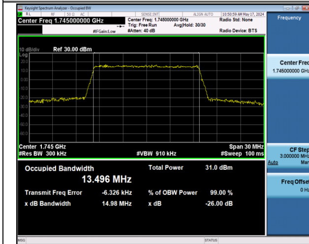
Band66-15MHz-16QAM-132322-75RB#0-PASS
