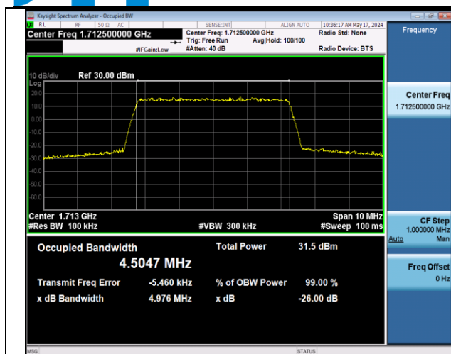
Band66-5MHz-QPSK-131997-25RB#0-PASS
