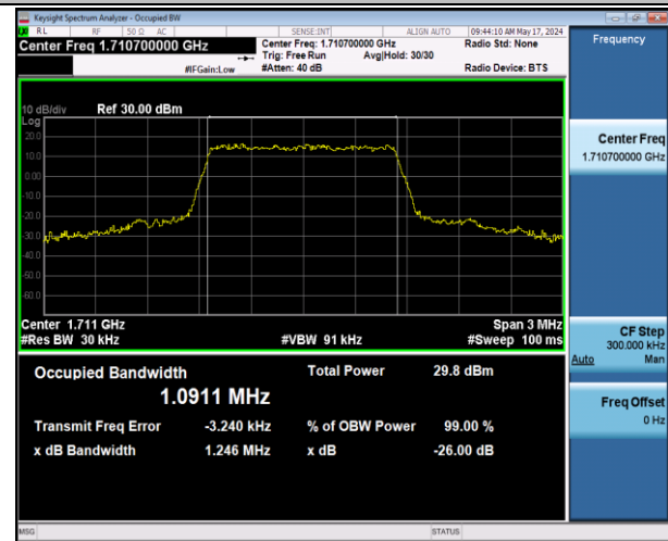
Band66-1.4MHz-16QAM-131979-6RB#0-PASS
