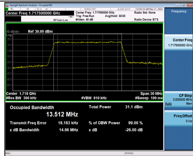
Band66-15MHz-16QAM-132047-75RB#0-PASS
