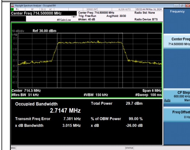
Band12-3MHz-QPSK-23165-15RB#0-PASS
