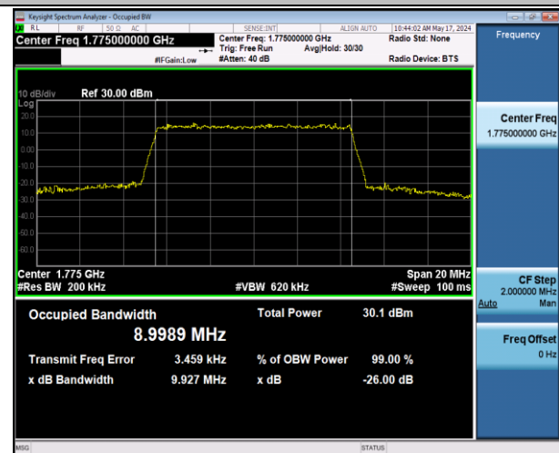
Band66-10MHz-16QAM-132622-50RB#0-PASS
