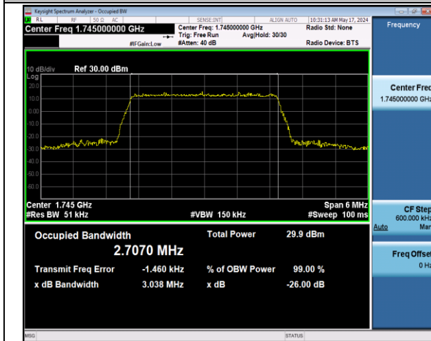
Band66-3MHz-16QAM-132322-15RB#0-PASS
