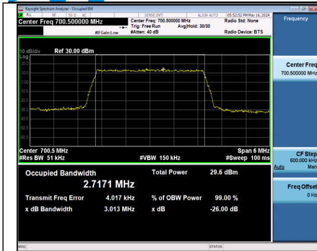
Band12-3MHz-QPSK-23025-15RB#0-PASS
