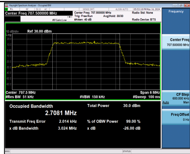
Band12-3MHz-QPSK-23095-15RB#0-PASS
