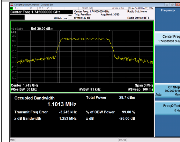
Band66-1.4MHz-16QAM-132322-6RB#0-PASS
