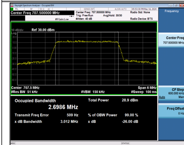
Band12-3MHz-16QAM-23095-15RB#0-PASS
