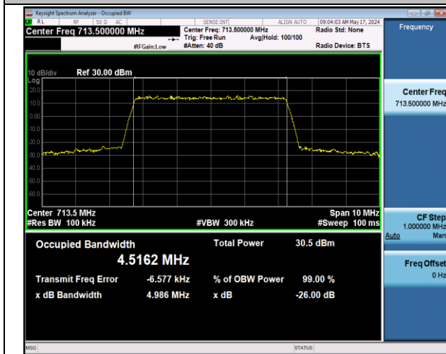
Band12-5MHz-QPSK-23155-25RB#0-PASS
