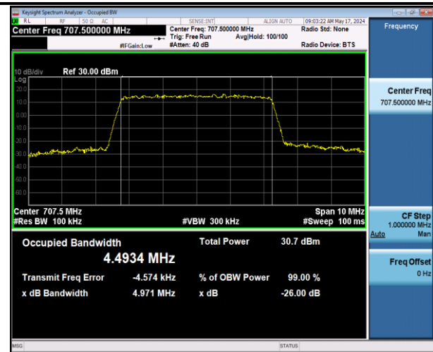
Band12-5MHz-QPSK-23095-25RB#0-PASS
