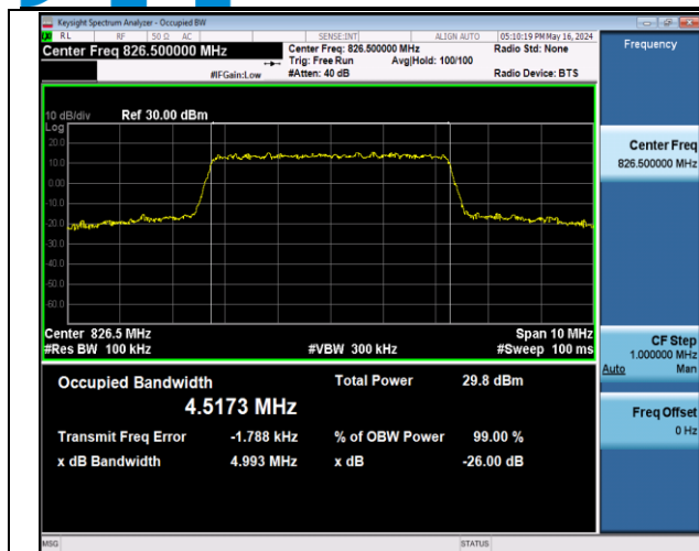
Band5-5MHz-QPSK-20425-25RB#0-PASS
