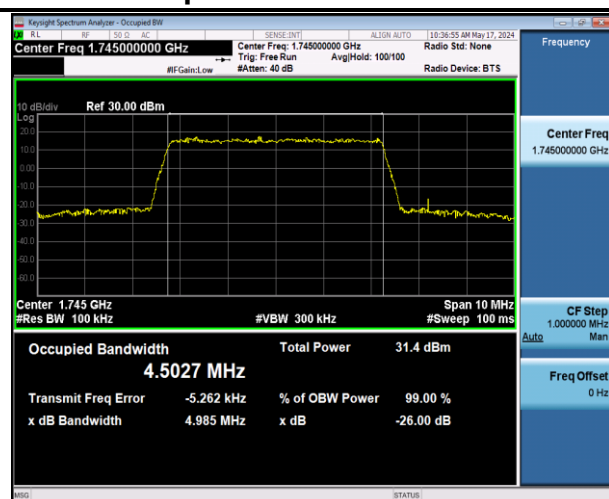
Band66-5MHz-QPSK-132322-25RB#0-PASS
