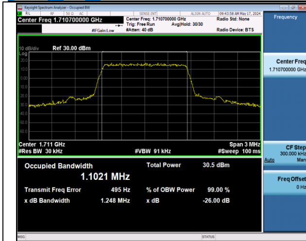
Band66-1.4MHz-QPSK-131979-6RB#0-PASS
