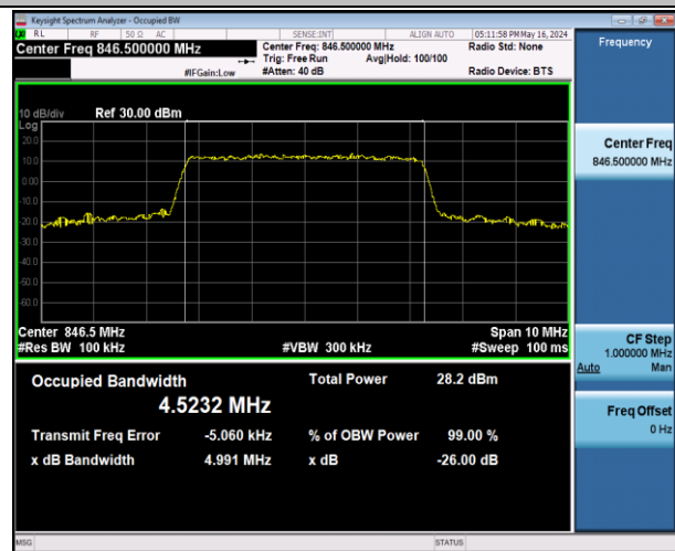
Band5-5MHz-16QAM-20625-25RB#0-PASS
