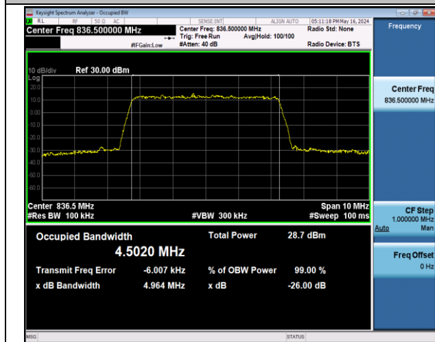
Band5-5MHz-16QAM-20525-25RB#0-PASS
