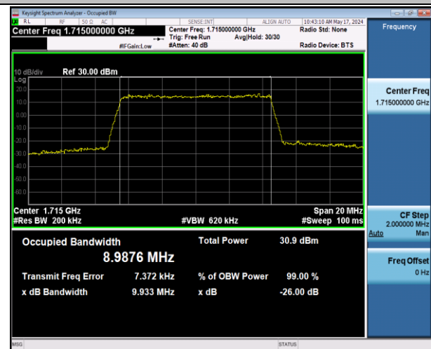
Band66-10MHz-16QAM-132022-50RB#0-PASS
