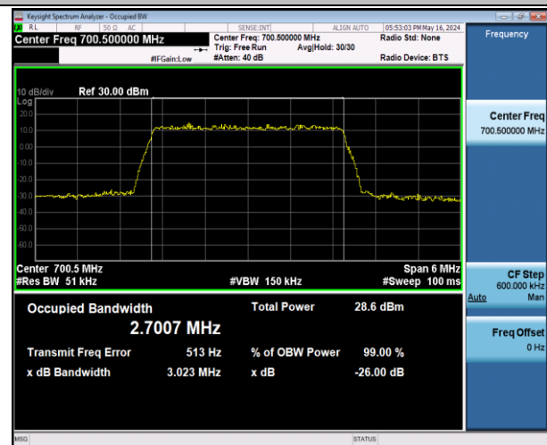
Band12-3MHz-16QAM-23025-15RB#0-PASS
