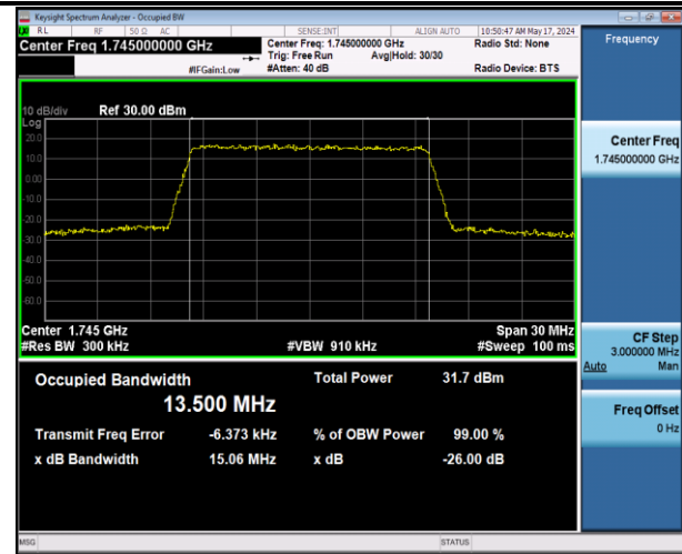
Band66-15MHz-QPSK-132322-75RB#0-PASS
