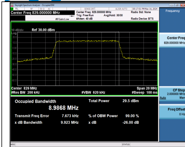
Band5-10MHz-QPSK-20450-50RB#0-PASS
