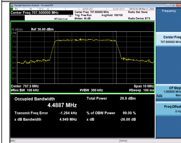
Band12-5MHz-16QAM-23095-25RB#0-PASS
