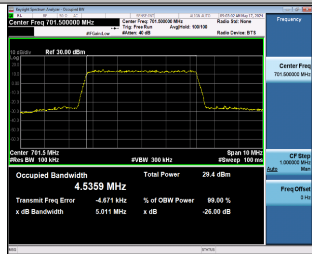
Band12-5MHz-16QAM-23035-25RB#0-PASS
