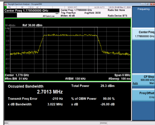
Band66-3MHz-16QAM-132657-15RB#0-PASS
