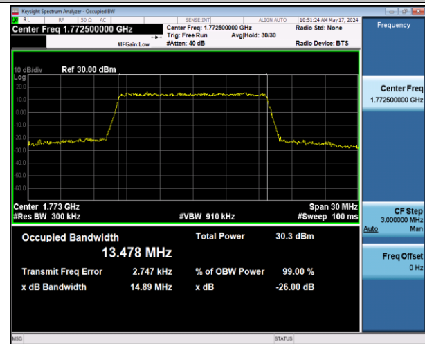
Band66-15MHz-16QAM-132597-75RB#0-PASS
