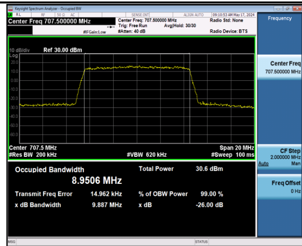
Band12-10MHz-QPSK-23095-50RB#0-PASS
