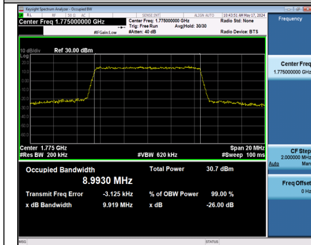
Band66-10MHz-QPSK-132622-50RB#0-PASS
