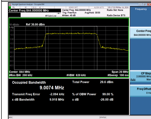
Band5-10MHz-QPSK-20600-50RB#0-PASS
