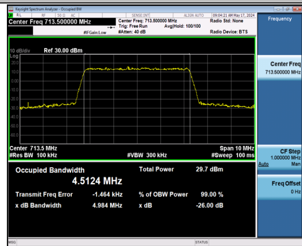
Band12-5MHz-16QAM-23155-25RB#0-PASS
