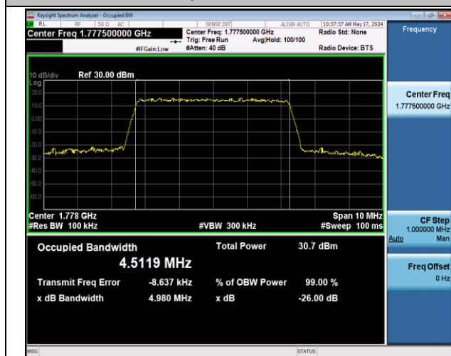
Band66-5MHz-QPSK-132647-25RB#0-PASS
