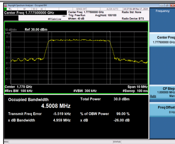
Band66-5MHz-16QAM-132647-25RB#0-PASS
