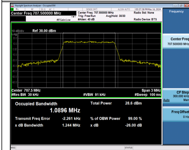
Band12-1.4MHz-16QAM-23095-6RB#0-PASS
