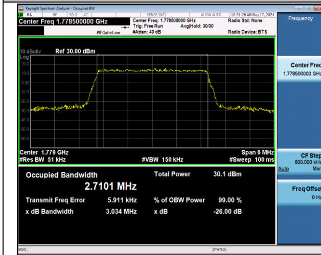
Band66-3MHz-QPSK-132657-15RB#0-PASS
