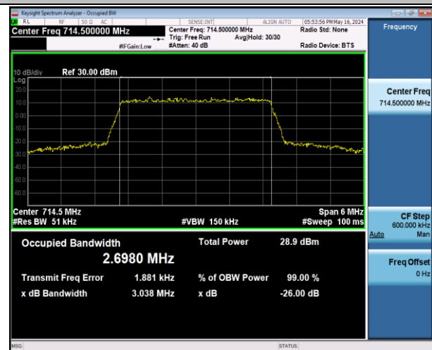
Band12-3MHz-16QAM-23165-15RB#0-PASS
