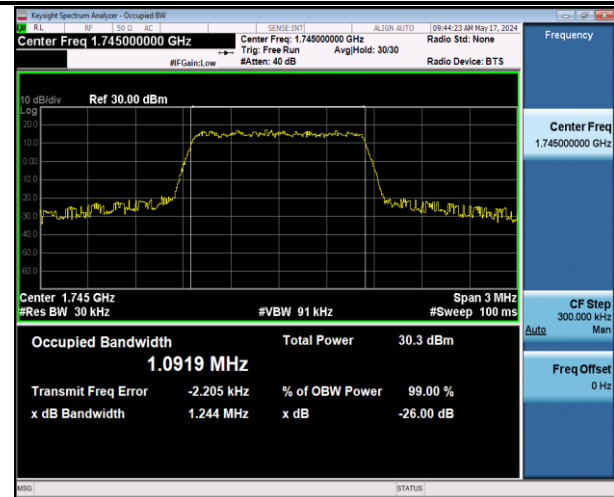
Band66-1.4MHz-QPSK-132322-6RB#0-PASS
