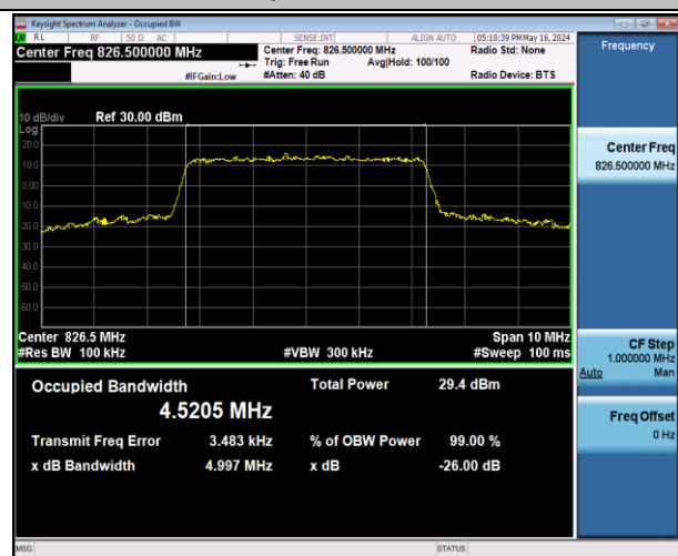
Band5-5MHz-16QAM-20425-25RB#0-PASS
