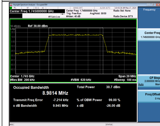
Band66-10MHz-16QAM-132322-50RB#0-PASS
