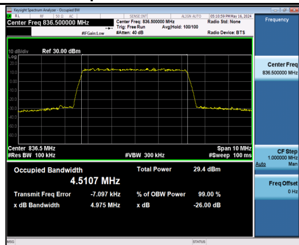
Band5-5MHz-QPSK-20525-25RB#0-PASS
