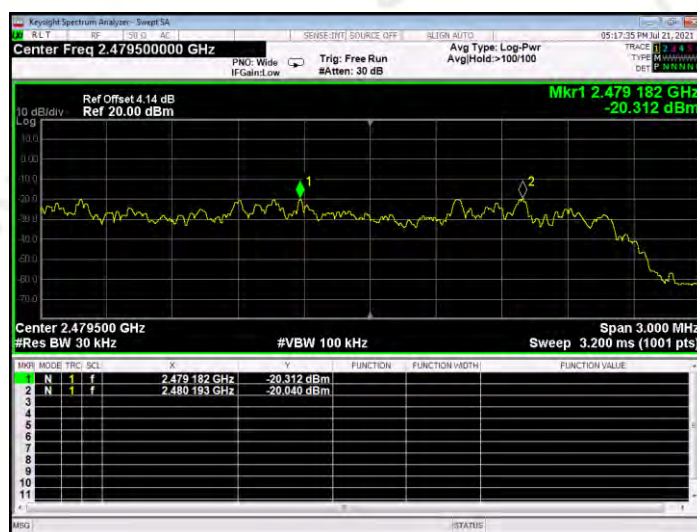
\pi/4 -DQPSK Highest Channel
