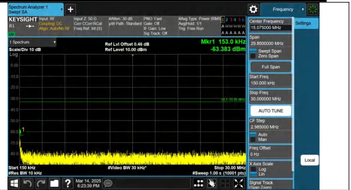
Band2-20MHz-QPSK-18900-1RB#0-0.15~30-PASS
