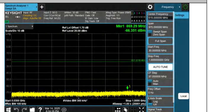
Band2-20MHz-QPSK-18900-1RB#99-30~1000-PASS
