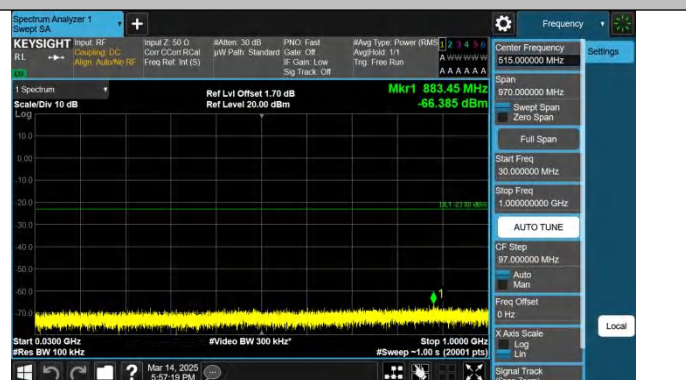
Band2-5MHz-QPSK-19175-1RB#24-30~1000-PASS
