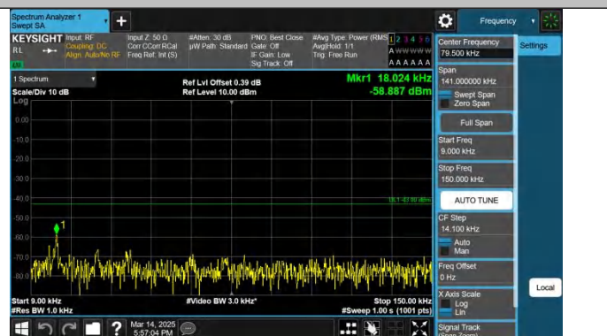
Band2-5MHz-QPSK-19175-1RB#24-0.009~0.15-PASS
