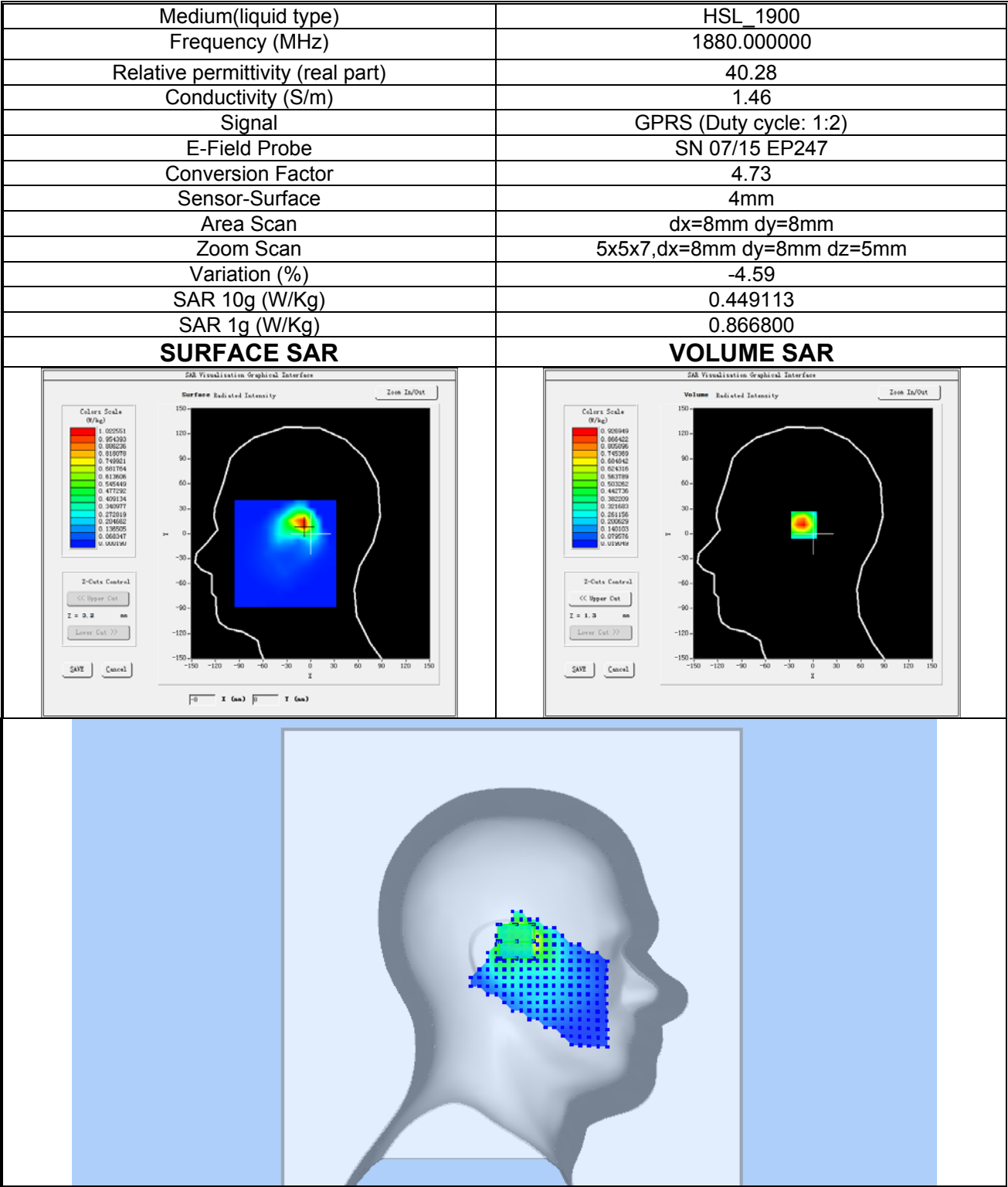
Plot 3: GPRS1900, Mid channel (Left Head Cheek) Product Description: Mobile Phone Test Date: 2020-04-30
