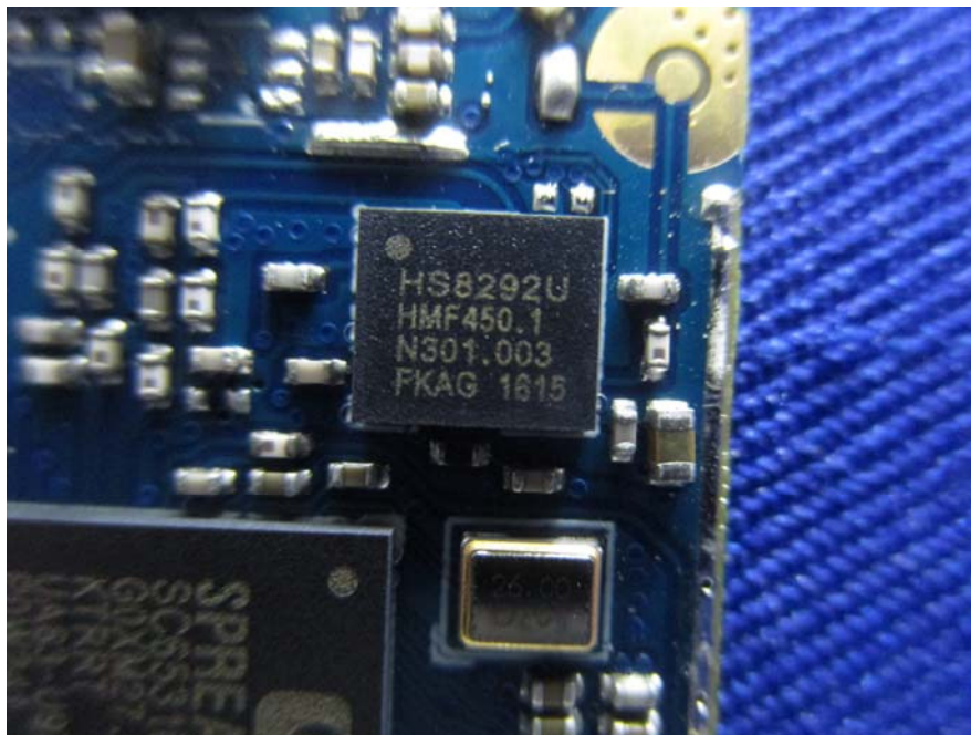
EUT – RF Switch View
