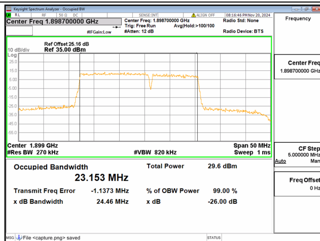
2C / 15+10MHz / 16QAM/ High CH
