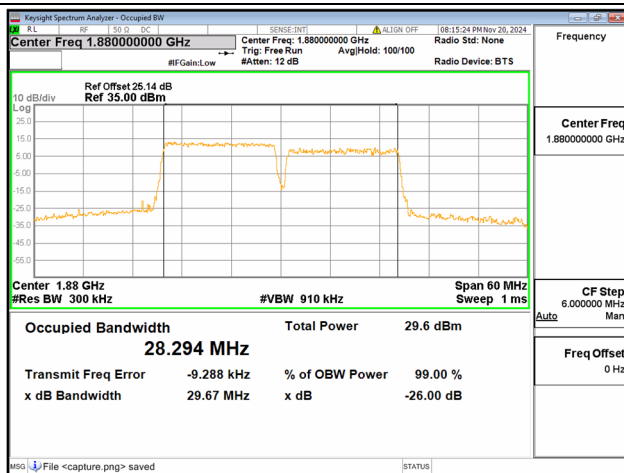
2C / 15+15MHz / 16QAM/ Mid CH
