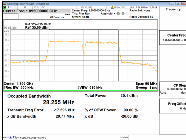
2C / 15+15MHz / 64QAM/ High CH
