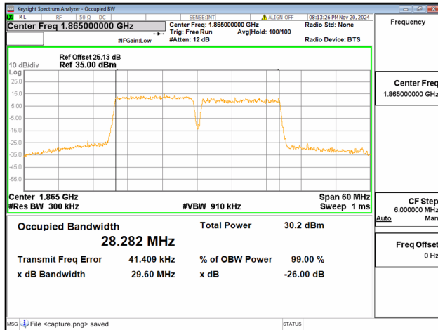
2C / 15+15MHz / 64QAM/ Low CH
