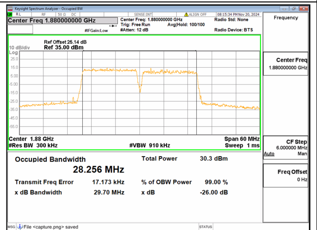
2C / 15+15MHz / 64QAM/ Mid CH
