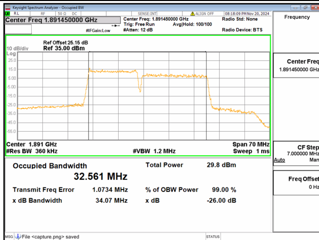
2C / 15+20MHz / 16QAM/ High CH
