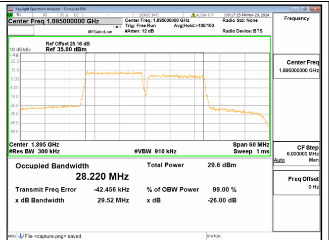
2C / 15+15MHz / 16QAM/ High CH
