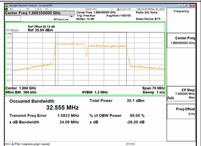
2C / 15+20MHz / 64QAM/ Low CH
