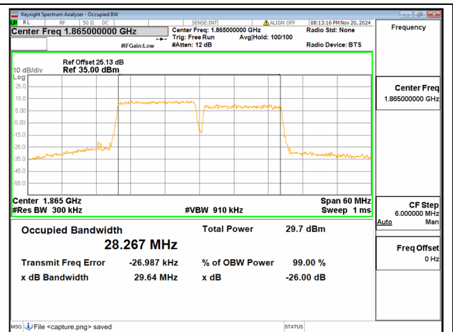
2C / 15+15MHz / 16QAM/ Low CH
