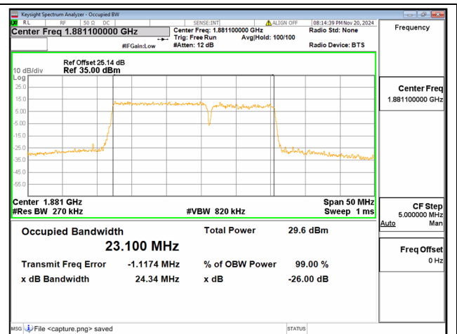
2C / 15+10MHz / 16QAM/ Mid CH
