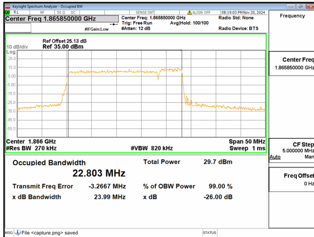
2C / 20+5MHz / 64QAM/ Low CH
