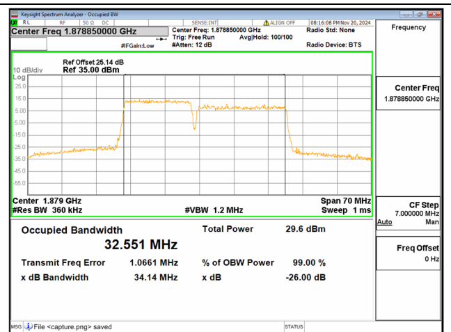
2C / 15+20MHz / 16QAM/ Mid CH
