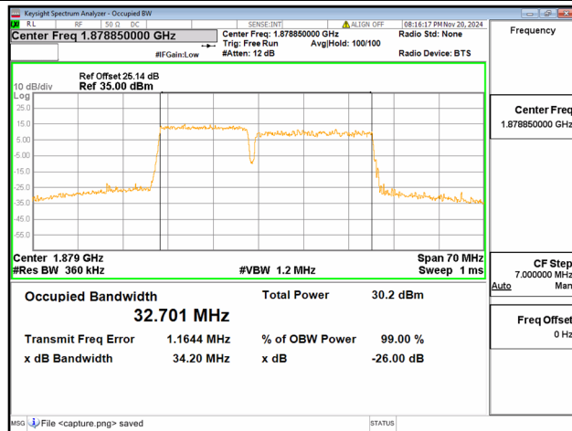
2C / 15+20MHz / 64QAM/ Mid CH
