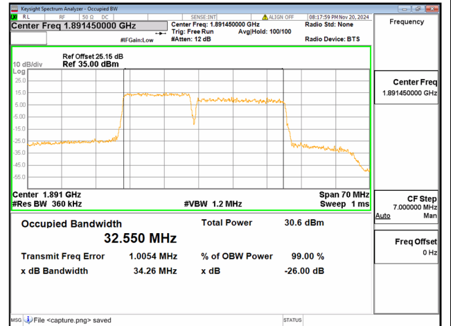
2C / 15+20MHz / QPSK/ High CH
