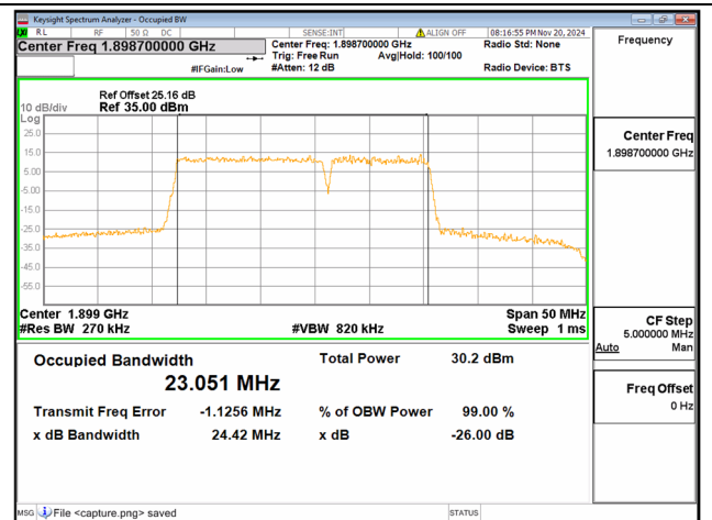
2C / 15+10MHz / 64QAM/ High CH
