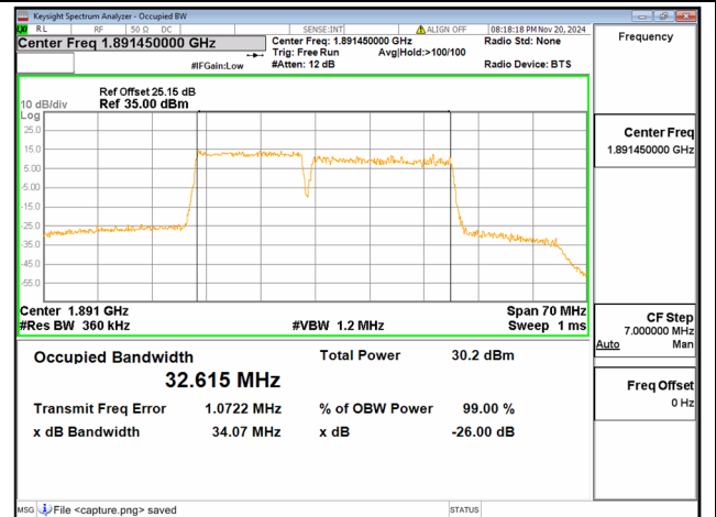
2C / 15+20MHz / 64QAM/ High CH
