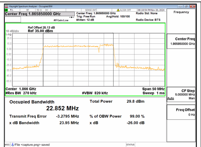
2C / 20+5MHz / 16QAM/ Low CH
