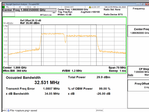
2C / 15+20MHz / 16QAM/ Low CH
