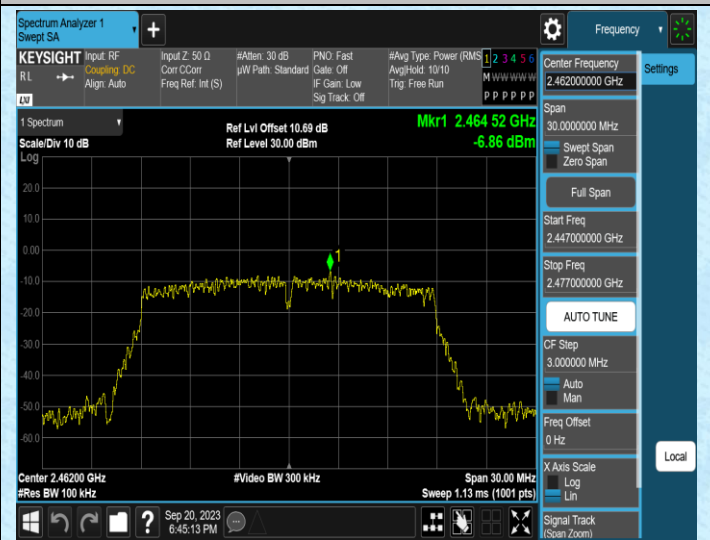
11N20SISO-Ant1-2462-0~Reference
