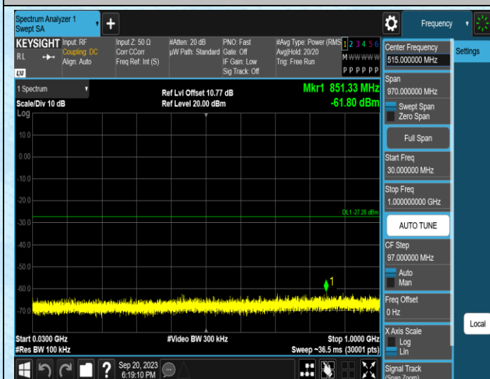
11N20SISO-Ant0-2437-30~1000
