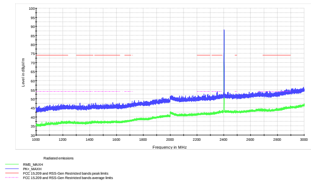
Figure 8.6-31: Radiated spurious emissions within 1–3 GHz, low channel
