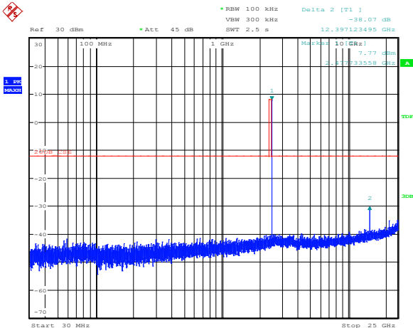
Figure 8.6-24: Conducted spurious emissions for BLE at low channel
