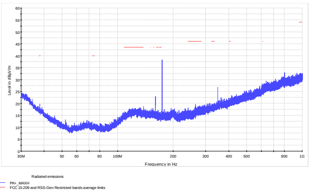
Figure 8.6-30: Radiated spurious emissions below 1 GHz, VHF radio on
