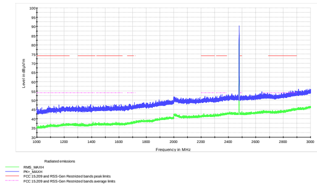
Figure 8.6-33: Radiated spurious emissions within 1–3 GHz, low channel
