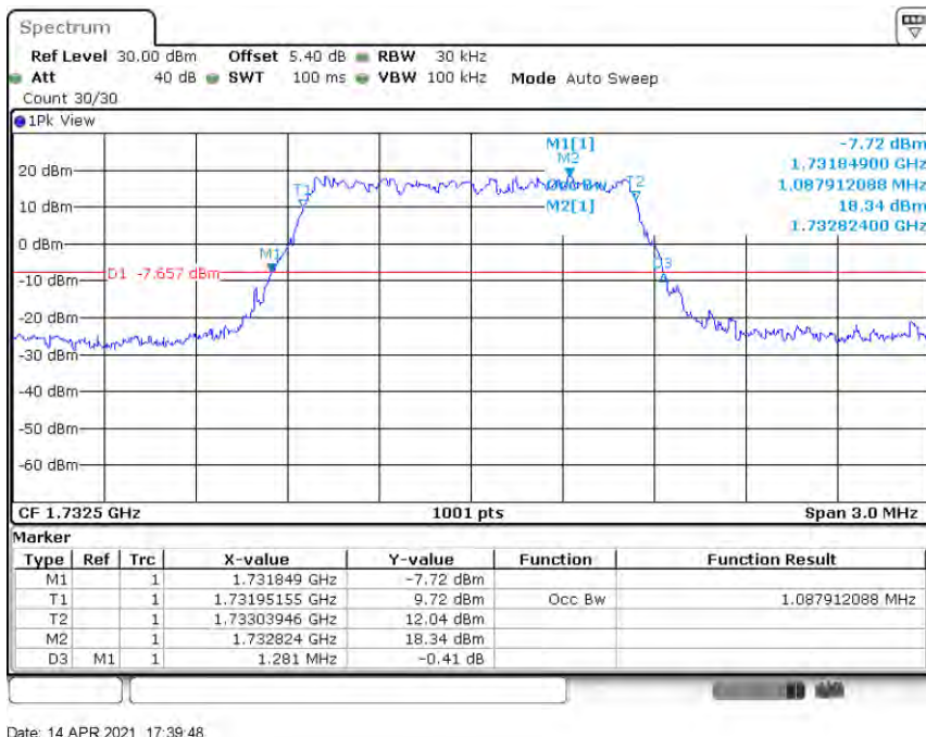
Band4-1.4MHz-QPSK-20175-6RB#0-1.088
