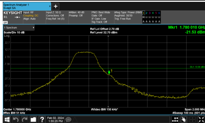
Band66-3MHz-QPSK-132657-15RB#0
