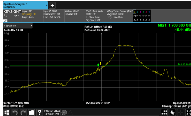
Band66-1.4MHz-QPSK-131979-1RB#5
