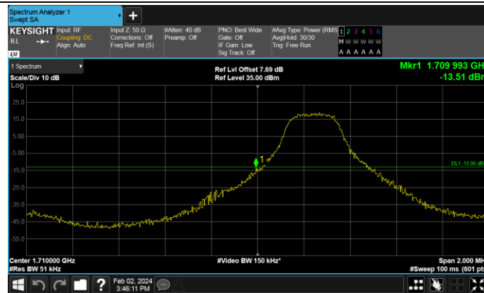
Band66-3MHz-16QAM-131987-1RB#14
