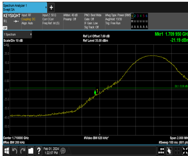
Band66-10MHz-QPSK-132022-1RB#49
