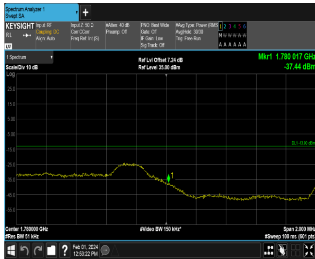
Band66-3MHz-QPSK-132657-1RB#14
