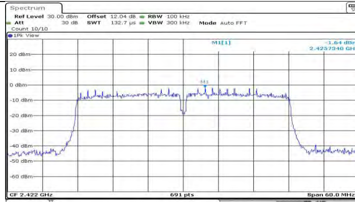
11N40SISO_Ant1_2422_0~Reference
