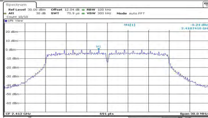
11N20SISO_Ant1_2412_0~Reference
