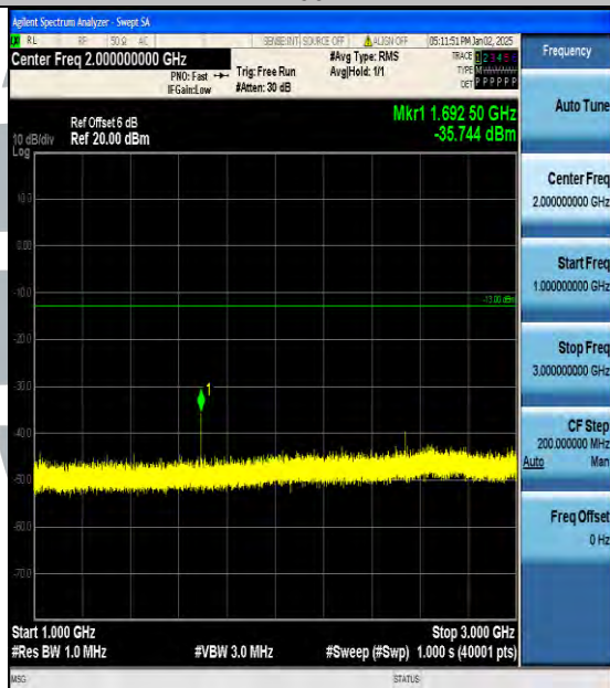
Band5_3MHz_16QAM_20635_1RB#0_1000~3000_1000~3000
