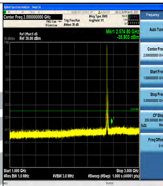
Band7_15MHz_16QAM_20825_1RB#0_1000~3000_1000~3000
