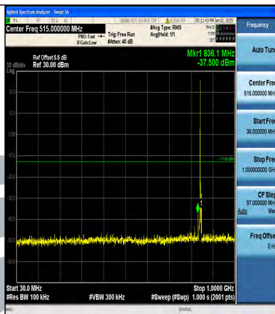
Band5_3MHz_16QAM_20635_1RB#0_30~1000_30~1000
