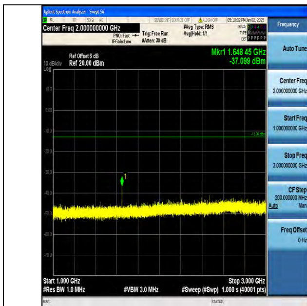
Band5_3MHz_16QAM_20415_1RB#0_1000~3000_1000~3000
