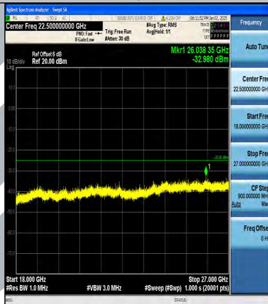
Band7_15MHz_16QAM_20825_1RB#0_18000~27000_18000~27000
