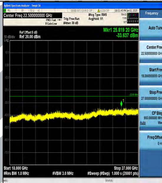
Band7_10MHz_QPSK_21100_1RB#0_18000~27000_18000~27000
