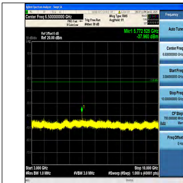
Band5_10MHz_QPSK_20450_1RB#0_3000~10000_3000~10000
