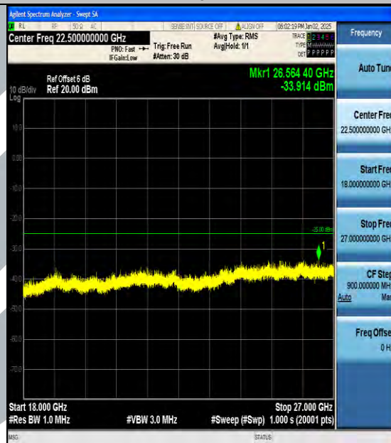
Band7_10MHz_16QAM_21100_1RB#0_18000~27000_18000~27000
