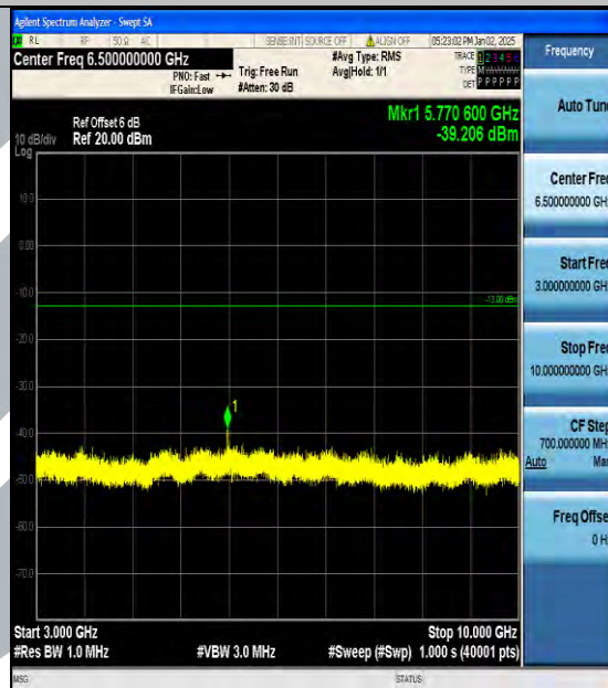
Band5_5MHz_16QAM_20425_1RB#0_3000~10000_3000~10000
