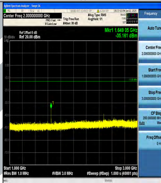
Band5_10MHz_QPSK_20450_1RB#0_1000~3000_1000~3000
