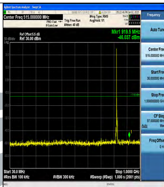
Band5_5MHz_16QAM_20425_1RB#0_30~1000_30~1000
