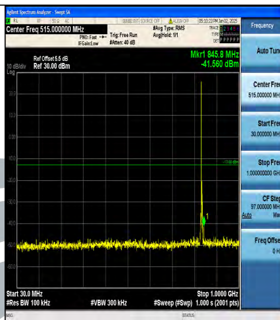
Band5_3MHz_QPSK_20525_1RB#0_30~1000_30~1000
