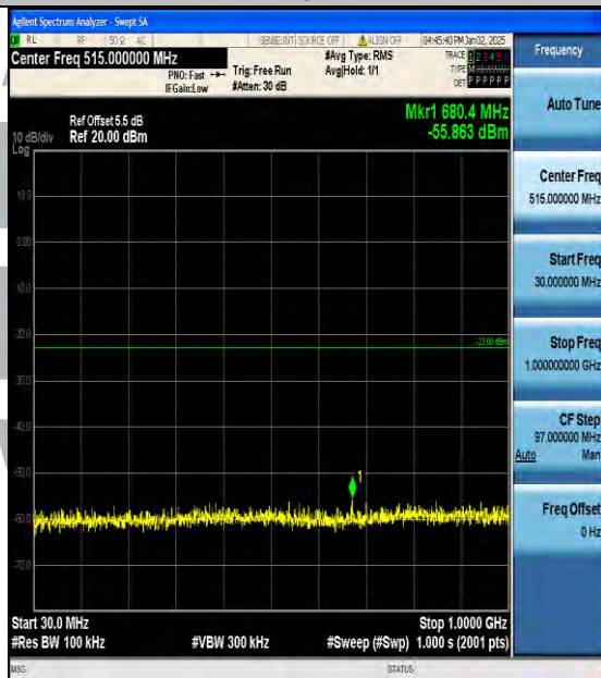
Band4_20MHz_16QAM_20175_1RB#0_30~1000_30~1000
