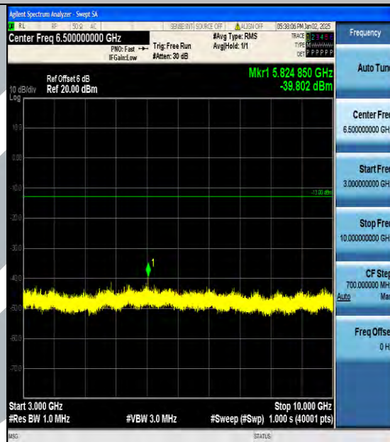
Band5_10MHz_QPSK_20525_1RB#0_3000~10000_3000~10000
