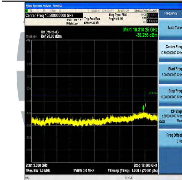
Band7_10MHz_16QAM_21400_1RB#0_3000~18000_3000~18000
