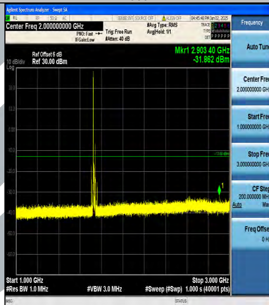
Band4_20MHz_16QAM_20175_1RB#0_1000~3000_1000~3000
