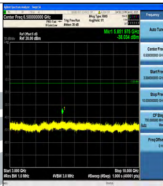
Band5_1.4MHz_QPSK_20525_1RB#0_3000~10000_3000~10000
