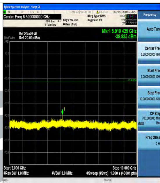
Band5_5MHz_16QAM_20625_1RB#0_3000~10000_3000~10000
