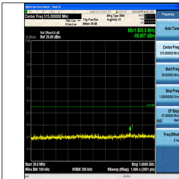
Band7_10MHz_16QAM_21100_1RB#0_30~1000_30~1000
