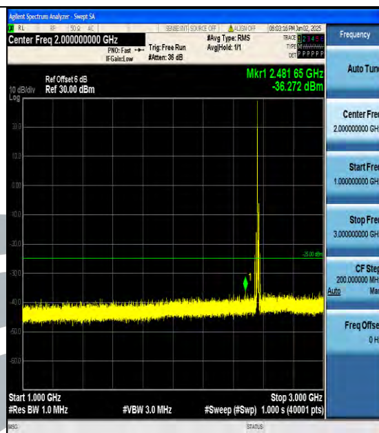
Band7_10MHz_16QAM_21400_1RB#0_1000~3000_1000~3000
