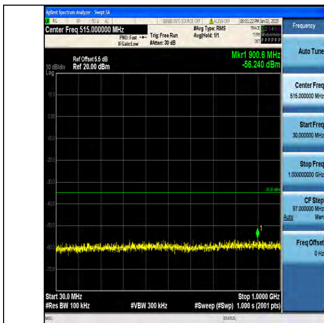
Band7_10MHz_QPSK_21100_1RB#0_30~1000_30~1000
