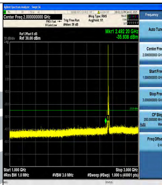
Band7_10MHz_QPSK_21100_1RB#0_1000~3000_1000~3000
