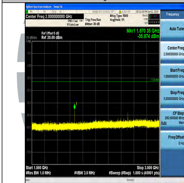
Band5_3MHz_QPSK_20525_1RB#0_1000~3000_1000~3000
