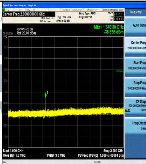
Band5_1.4MHz_16QAM_20407_1RB#0_1000~3000_1000~3000
