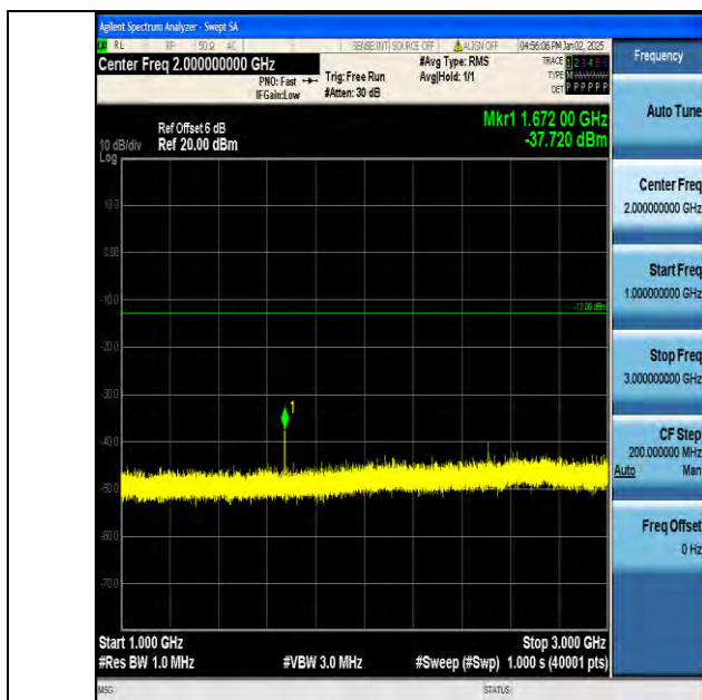
Band5_1.4MHz_QPSK_20525_1RB#0_1000~3000_1000~3000
