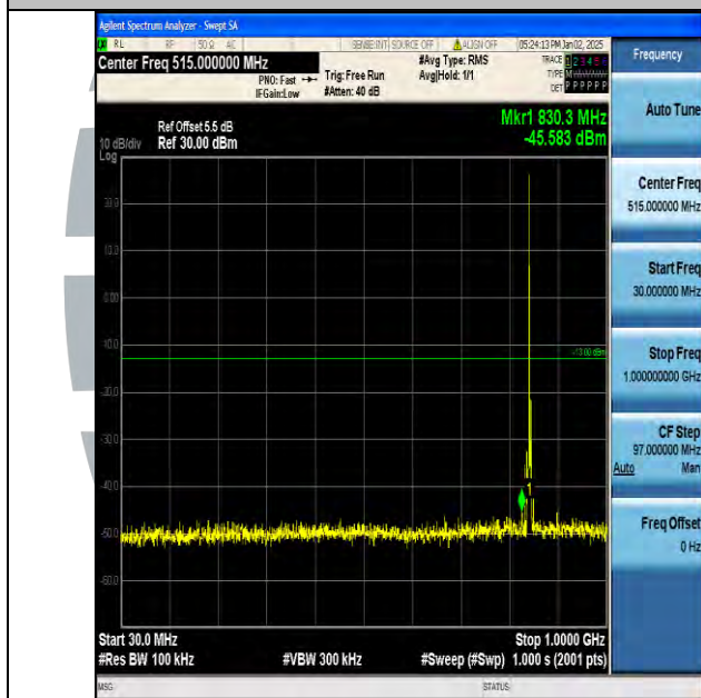
Band5_5MHz_QPSK_20625_1RB#0_30~1000_30~1000
