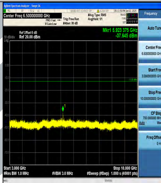
Band5_3MHz_16QAM_20635_1RB#0_3000~10000_3000~10000
