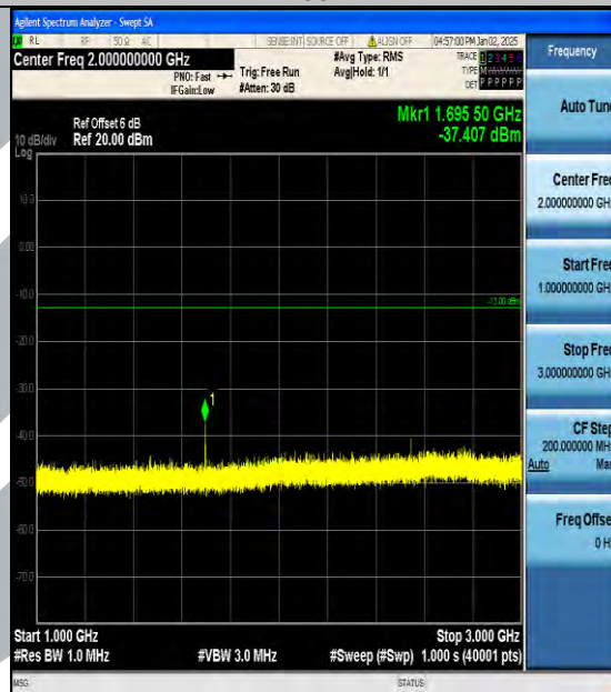
Band5_1.4MHz_QPSK_20643_1RB#0_1000~3000_1000~3000
