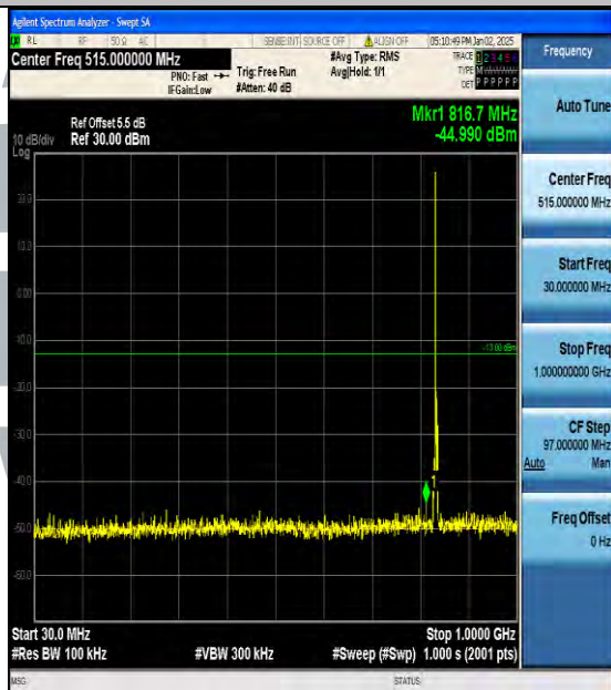
Band5 3MHz 16QAM 20525 1RB#0 30~1000 30~1000
