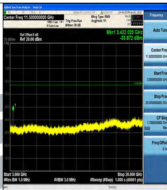
Band4_20MHz_16QAM_20050_1RB#0_3000~20000_3000~20000
