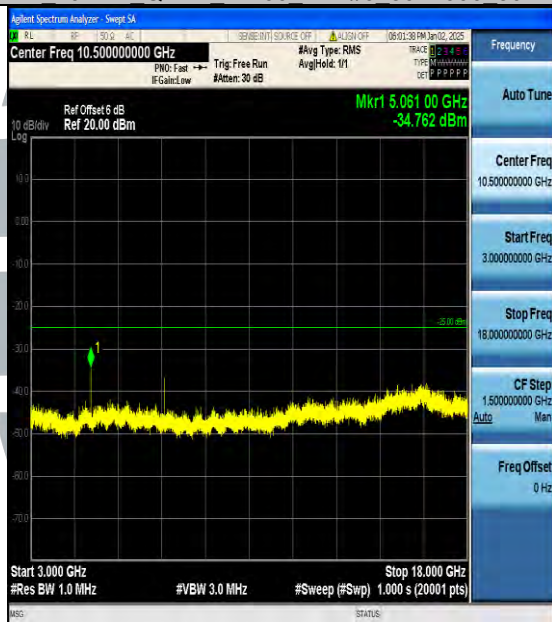
Band7_10MHz_QPSK_21100_1RB#0_3000~18000_3000~18000
