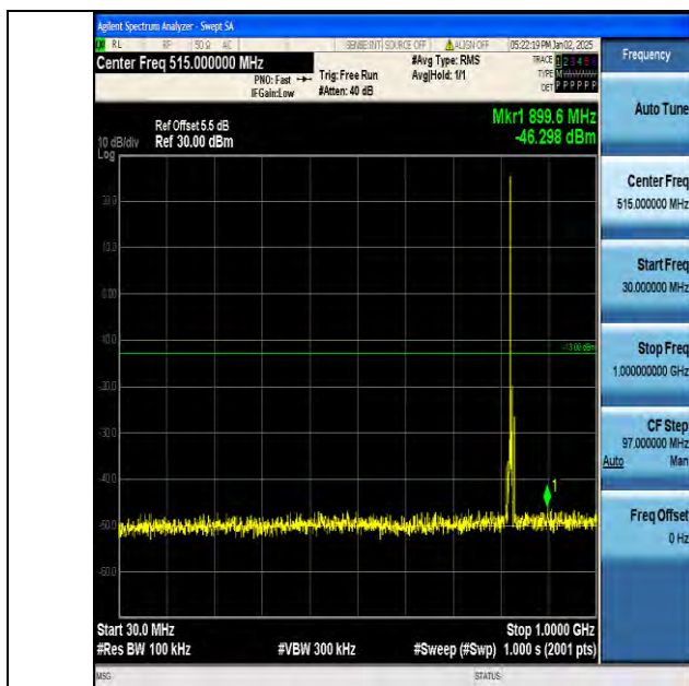
Band5_5MHz_QPSK_20425_1RB#0_30~1000_30~1000
