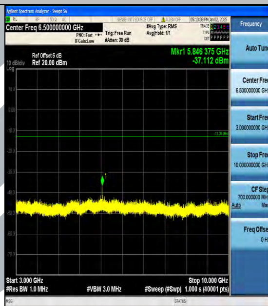
Band5_3MHz_QPSK_20525_1RB#0_3000~10000_3000~1000 0
