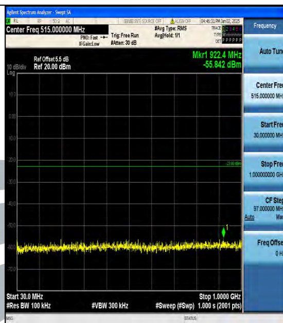
Band4_20MHz_16QAM_20300_1RB#0_30~1000_30~1000
