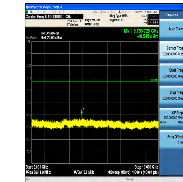
Band5_3MHz_QPSK_20415_1RB#0_3000~10000_3000~1000 0
