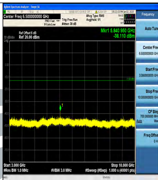
Band5_5MHz_QPSK_20525_1RB#0_3000~10000_3000~10000
