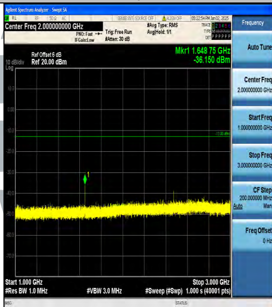
Band5_5MHz_16QAM_20425_1RB#0_1000~3000_1000~3000
