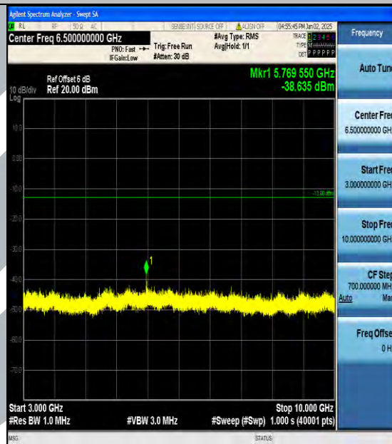
Band5_1.4MHz_16QAM_20407_1RB#0_3000~10000_3000~10000
