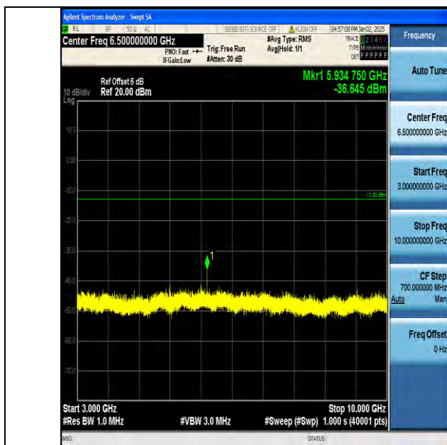
Band5_1.4MHz_QPSK_20643_1RB#0_3000~10000_3000~10000
