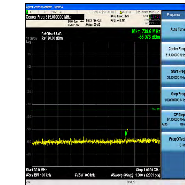
Band7_10MHz_16QAM_21400_1RB#0_30~1000_30~1000
