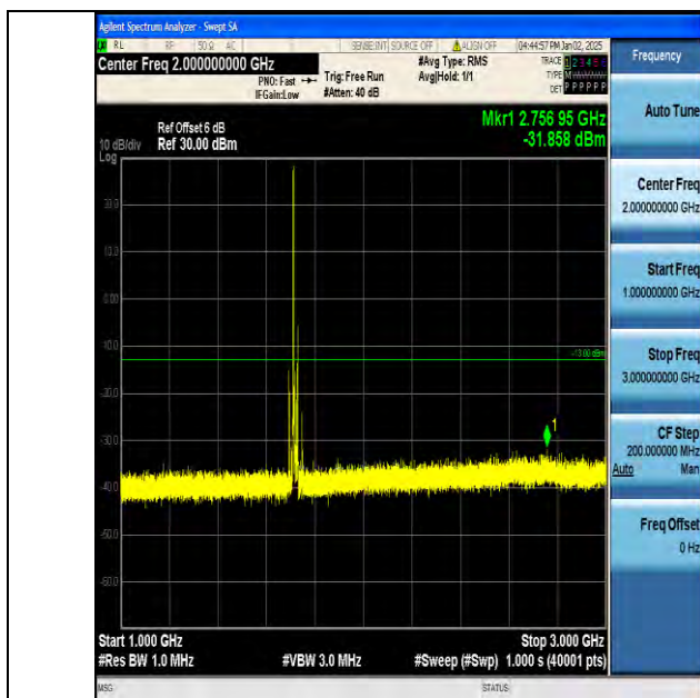
Band4_20MHz_16QAM_20050_1RB#0_1000~3000_1000~3000
