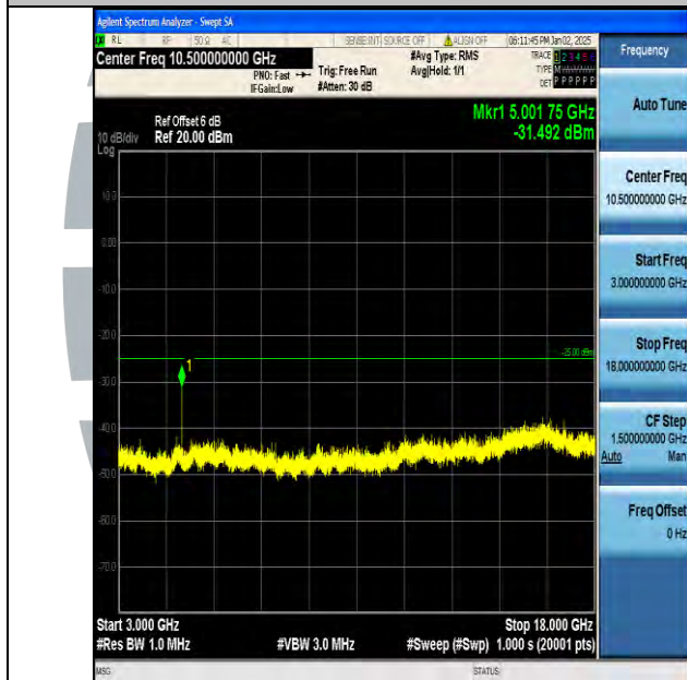
Band7_15MHz_16QAM_20825_1RB#0_3000~18000_3000~18000
