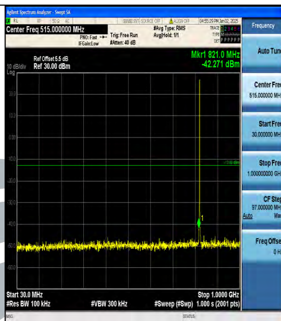
Band5_1.4MHz_16QAM_20407_1RB#0_30~1000_30~1000
