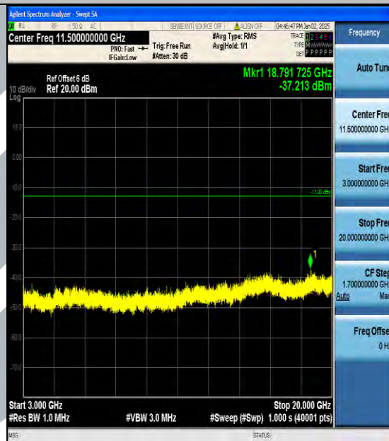
Band4_20MHz_16QAM_20300_1RB#0_3000~20000_3000~20000
