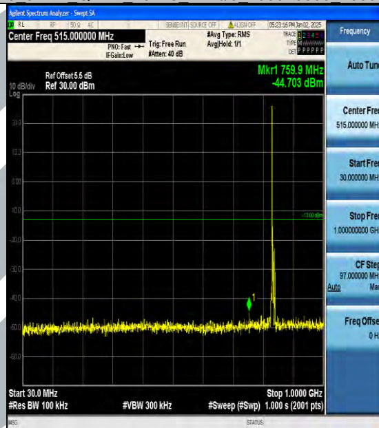
Band5_5MHz_QPSK_20525_1RB#0_30~1000_30~1000
