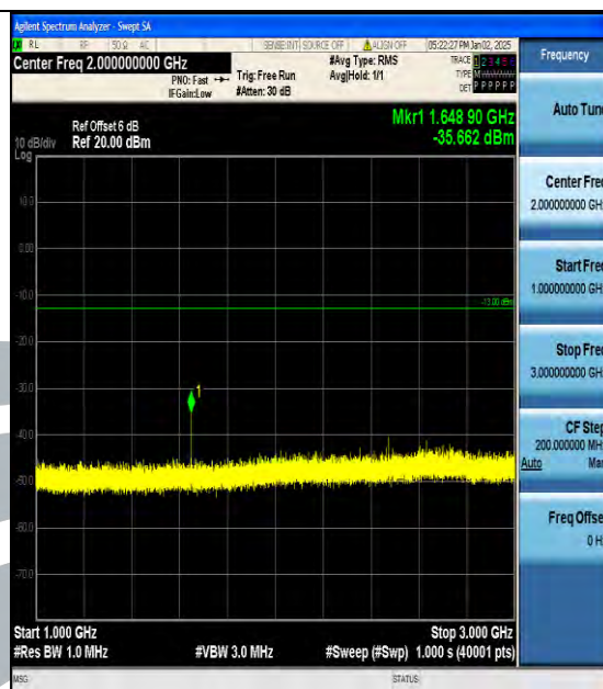
Band5_5MHz_QPSK_20425_1RB#0_1000~3000_1000~3000
