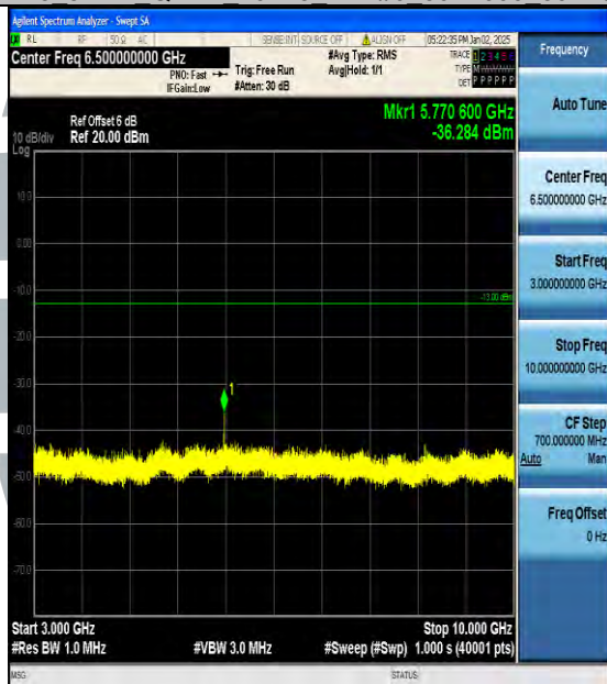
Band5_5MHz_QPSK_20425_1RB#0_3000~10000_3000~10000
