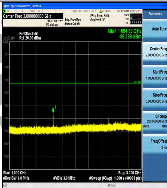
Band5_10MHz_QPSK_20525_1RB#0_1000~3000_1000~3000
