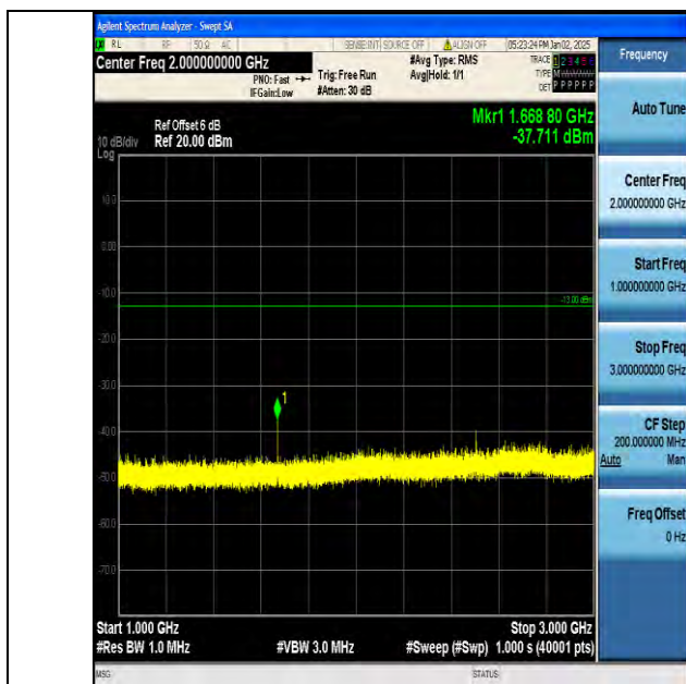
Band5_5MHz_QPSK_20525_1RB#0_1000~3000_1000~3000
