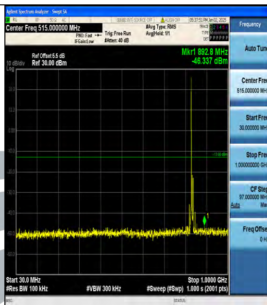
Band5_10MHz_QPSK_20525_1RB#0_30~1000_30~1000
