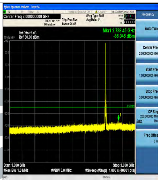
Band7_10MHz_16QAM_21100_1RB#0_1000~3000_1000~3000
