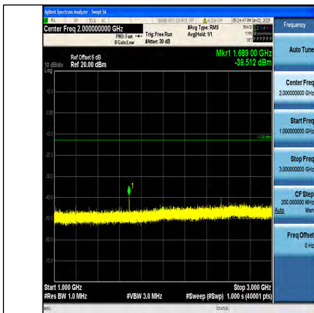
Band5_5MHz_16QAM_20625_1RB#0_1000~3000_1000~3000
