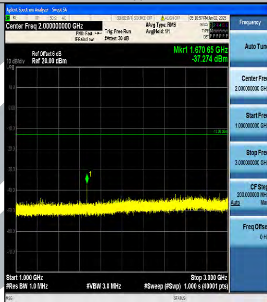
Band5 3MHz 16QAM 20525 1RB#0 1000~3000 1000~3000
