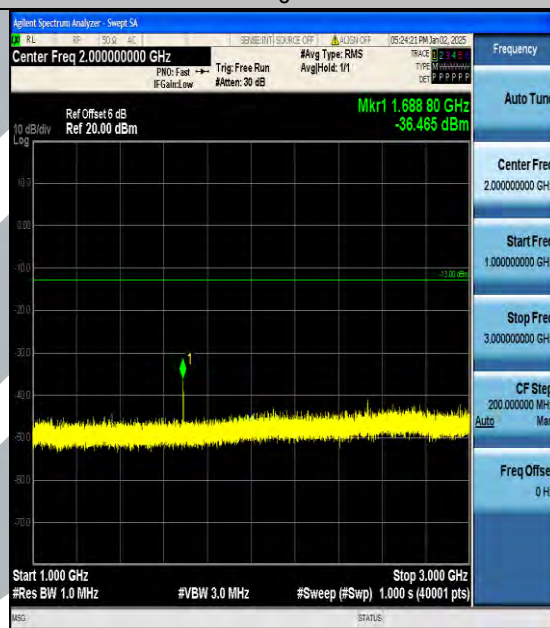
Band5_5MHz_QPSK_20625_1RB#0_1000~3000_1000~3000
