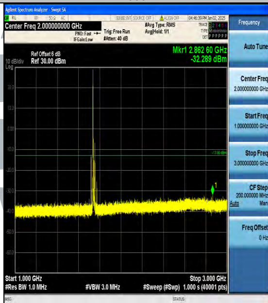
Band4_20MHz_16QAM_20300_1RB#0_1000~3000_1000~3000
