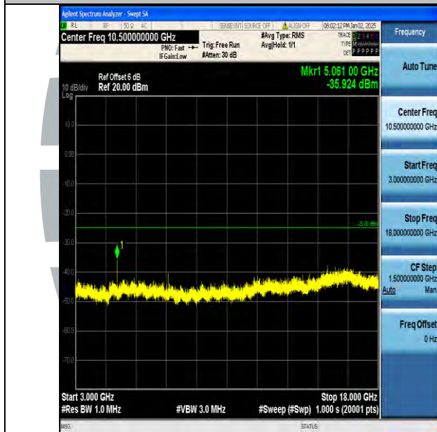
Band7_10MHz_16QAM_21100_1RB#0_3000~18000_3000~18000
