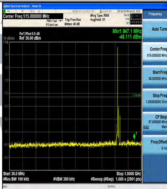
Band5_10MHz_QPSK_20450_1RB#0_30~1000_30~1000
