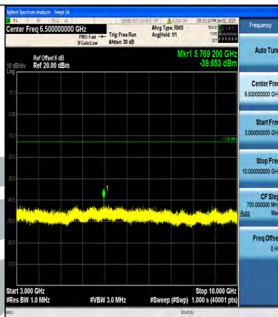
Band5_3MHz_16QAM_20415_1RB#0_3000~10000_3000~10000
