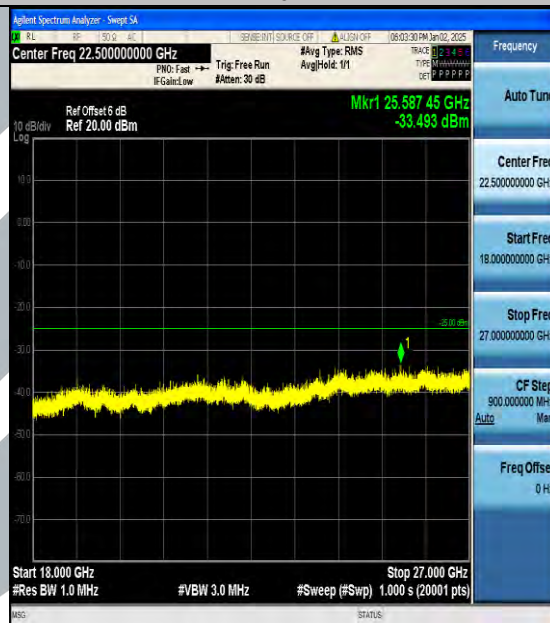
Band7_10MHz_16QAM_21400_1RB#0_18000~27000_18000~27000
