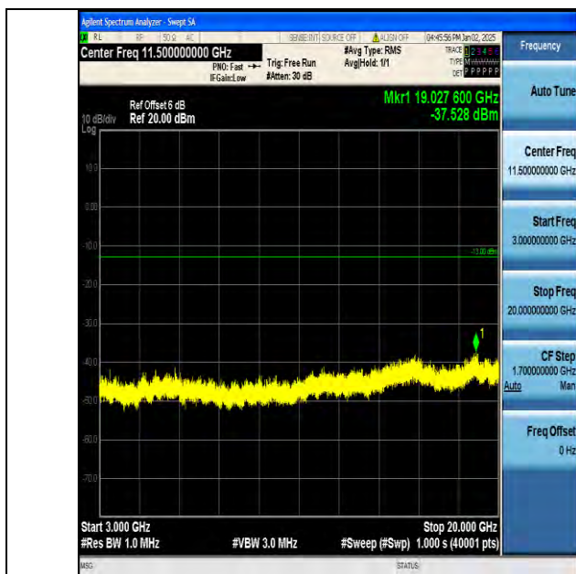
Band4_20MHz_16QAM_20175_1RB#0_3000~20000_3000~20000
