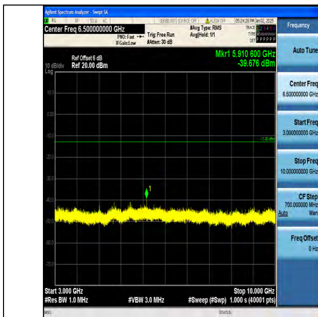
Band5_5MHz_QPSK_20625_1RB#0_3000~10000_3000~10000
