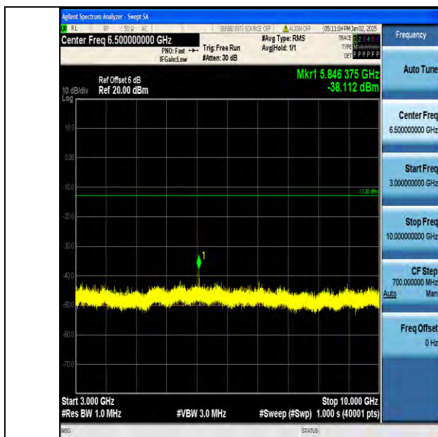
Band5_3MHz_16QAM_20525_1RB#0_3000~10000_3000~10000
