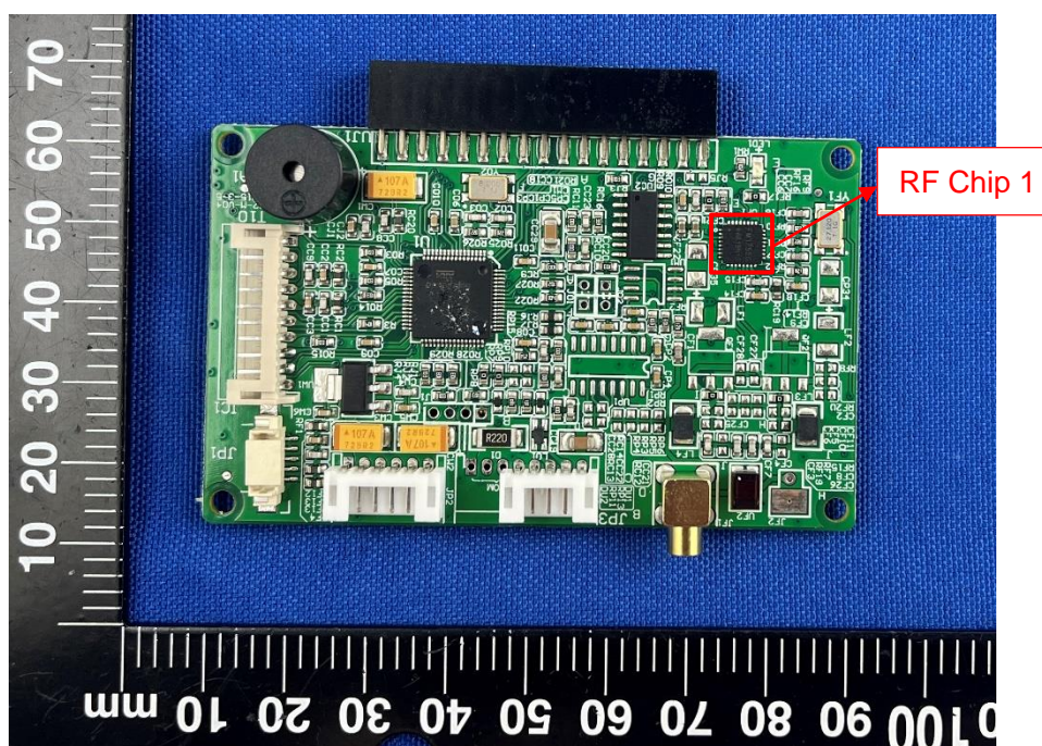
SECONDARY BOARD 1 TOP VIEW (RFID-1)
