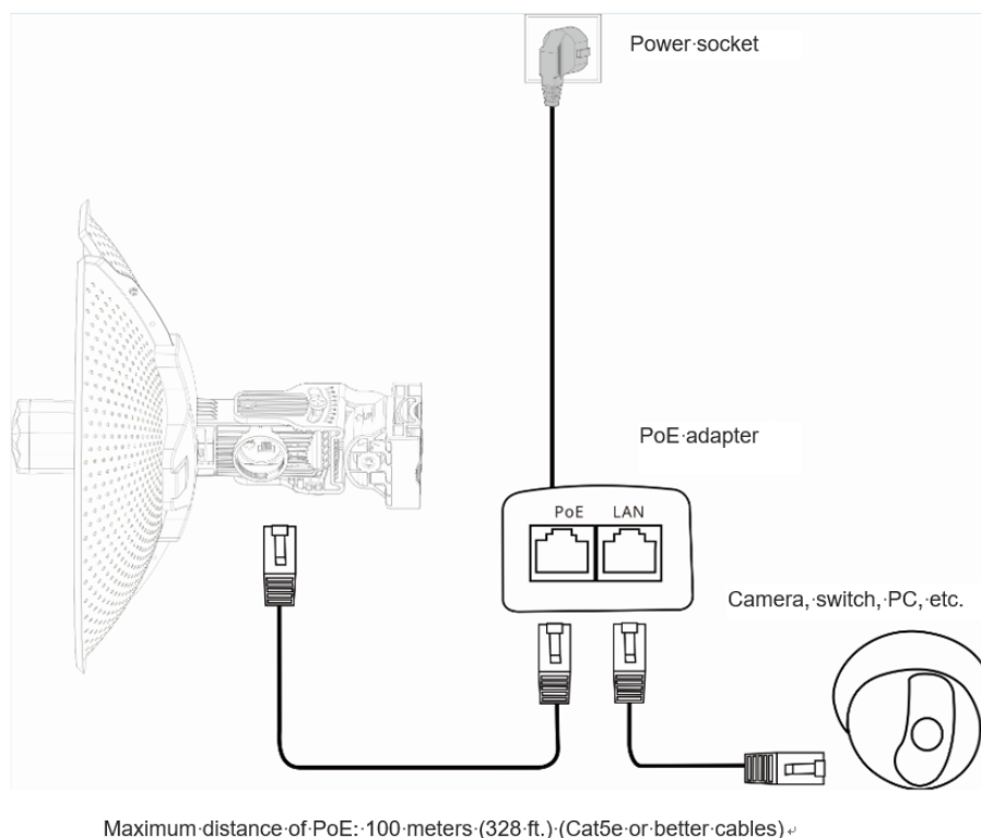
Figure 3-1 Cable Connection
