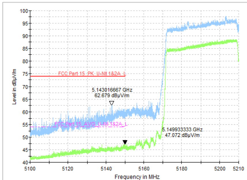
Fig. 27 Band Edges (802.11ac-VHT80, CH42 5210MHz)
