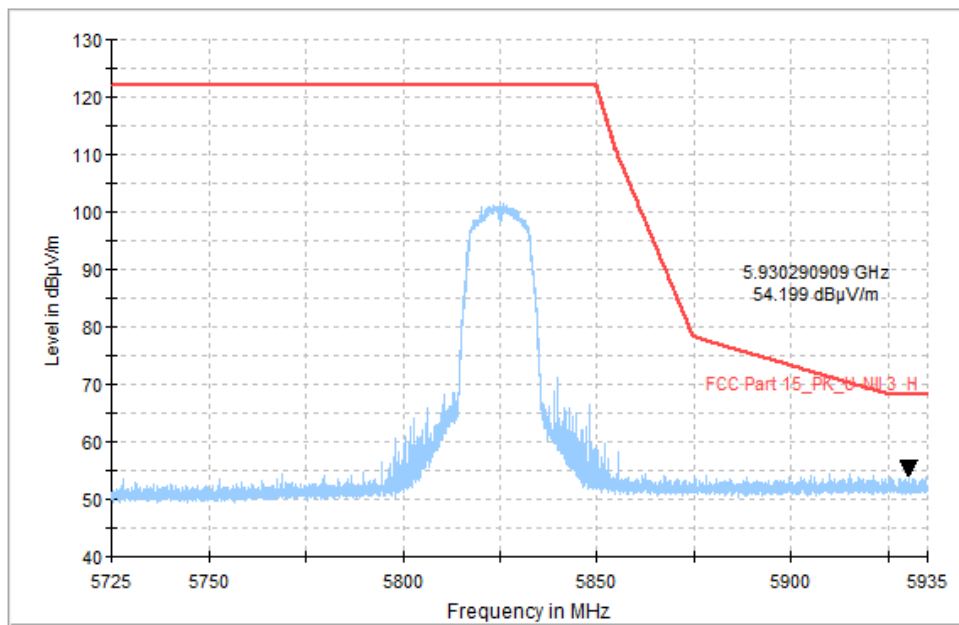
Fig. 22 Band Edges (802.11a, CH165 5825MHz)
