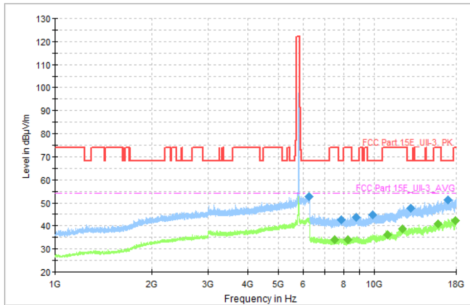
Fig. 44 Transmitter Spurious Emission (802.11n-HT40, CH159 5795MHz)
