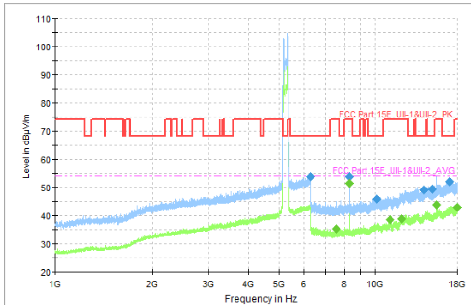
Fig. 30 Transmitter Spurious Emission (802.11a, CH36 5180MHz)
