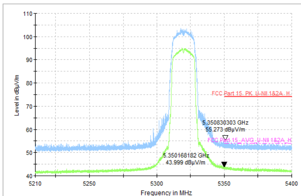
Fig. 20 Band Edges (802.11a, CH64 5320MHz)
