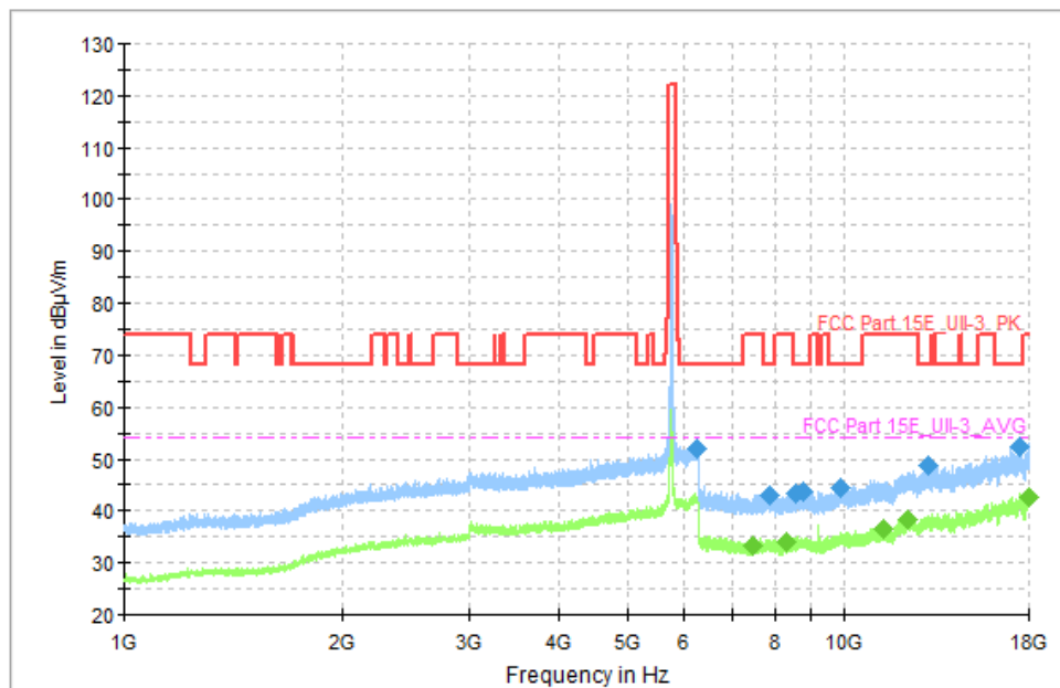
Fig. 43 Transmitter Spurious Emission (802. 11n-HT40, CH151 5755MHz)
