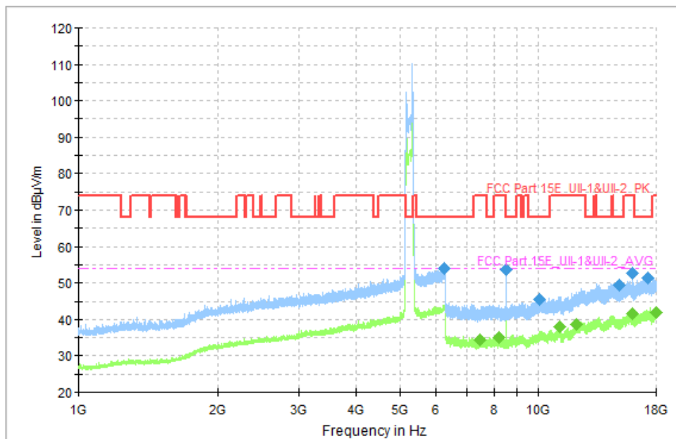
Fig. 35 Transmitter Spurious Emission (802.11a, CH64 5320MHz)
