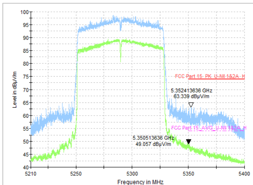
Fig. 28 Band Edges (802.11ac-VHT80, CH58 5290MHz)
