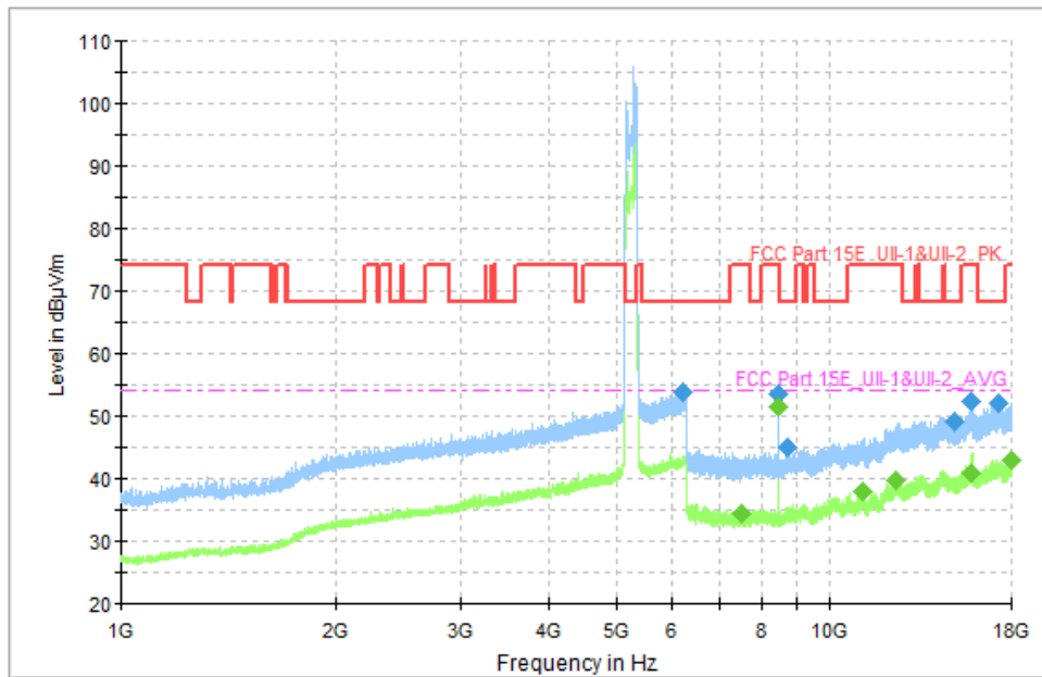
Fig. 34 Transmitter Spurious Emission (802.11a, CH56 5280MHz)
