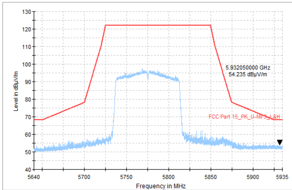
Fig. 29 Band Edges (802.11ac-VHT80, CH155 5775MHz)
