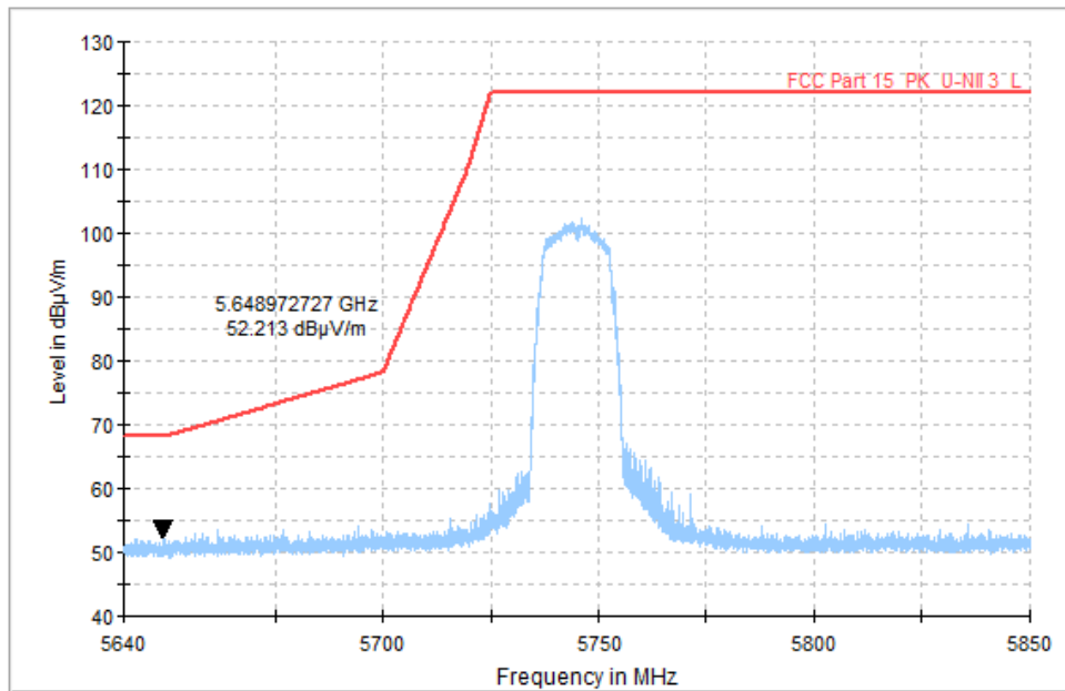
Fig. 21 Band Edges (802.11a, CH149 5745MHz)
