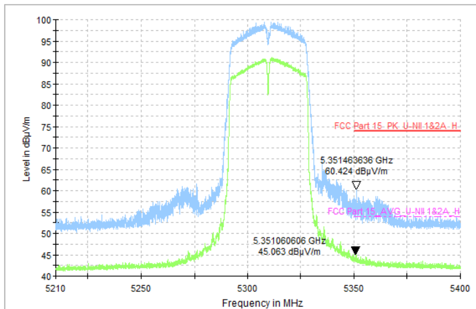
Fig. 24 Band Edges (802.11n-HT40, CH62 5310MHz)
