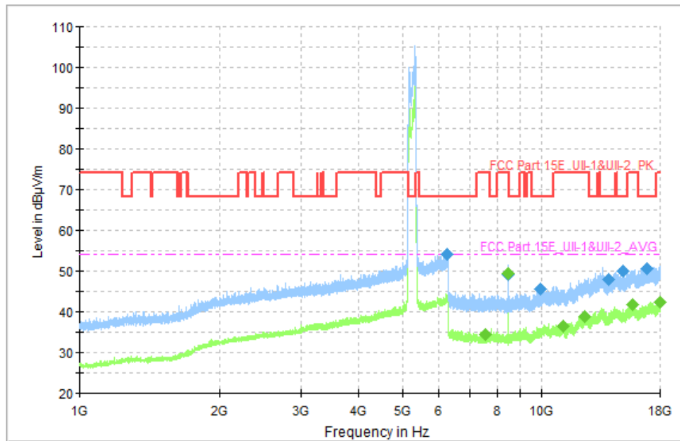
Fig. 46 Transmitter Spurious Emission (802.11ac-VHT80, CH58 5290MHz)
