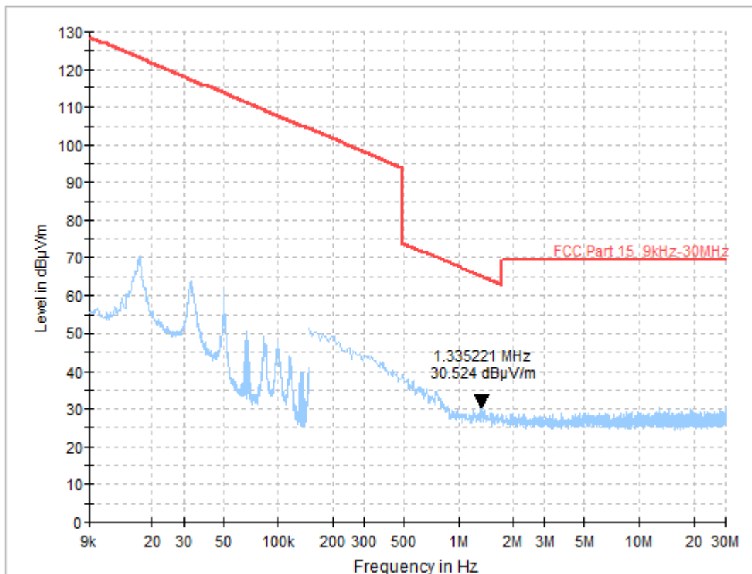
Fig. 51 Radiated Spurious Emission (All Channel, 9 kHz ~30 MHz)
