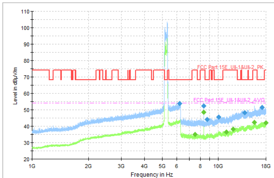
Fig. 45 Transmitter Spurious Emission (802.11ac-VHT80, CH42 5210MHz)
