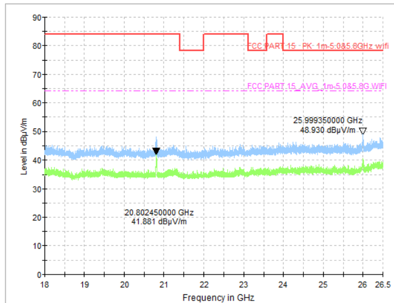
Fig. 49 Transmitter Spurious Emission (All channel, 18GHz~26.5GHz)
