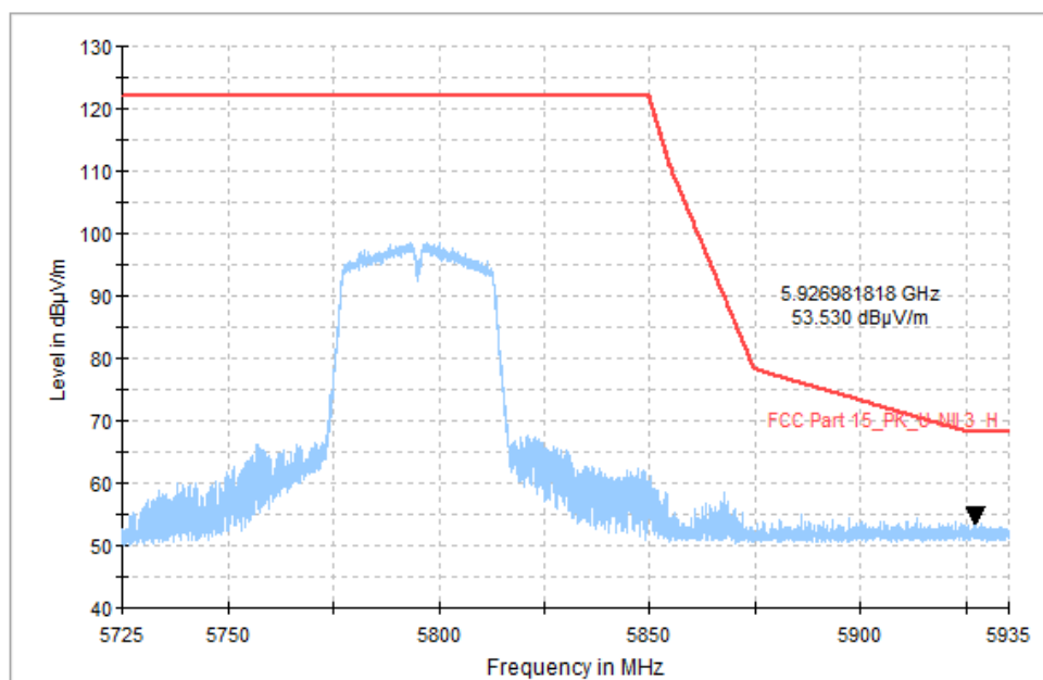
Fig. 26 Band Edges (802.11n-HT40, CH159 5795MHz)
