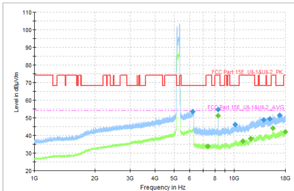
Fig. 39 Transmitter Spurious Emission (802.11n-HT40, CH38 5190MHz)
