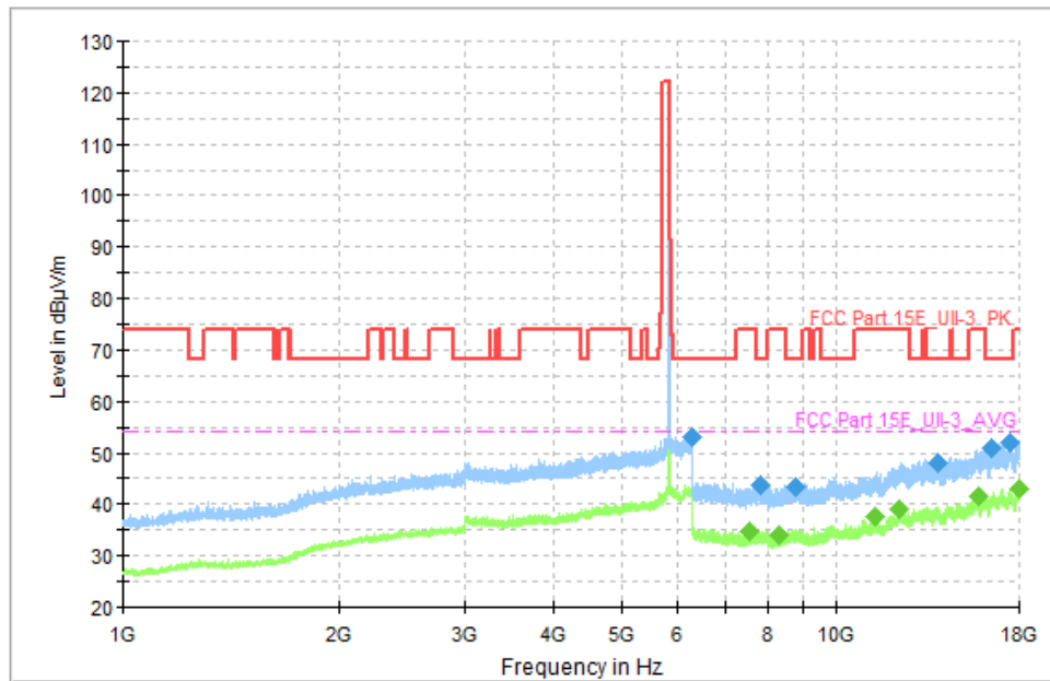
Fig. 38 Transmitter Spurious Emission (802. 11a, CH165 5825MHz)
