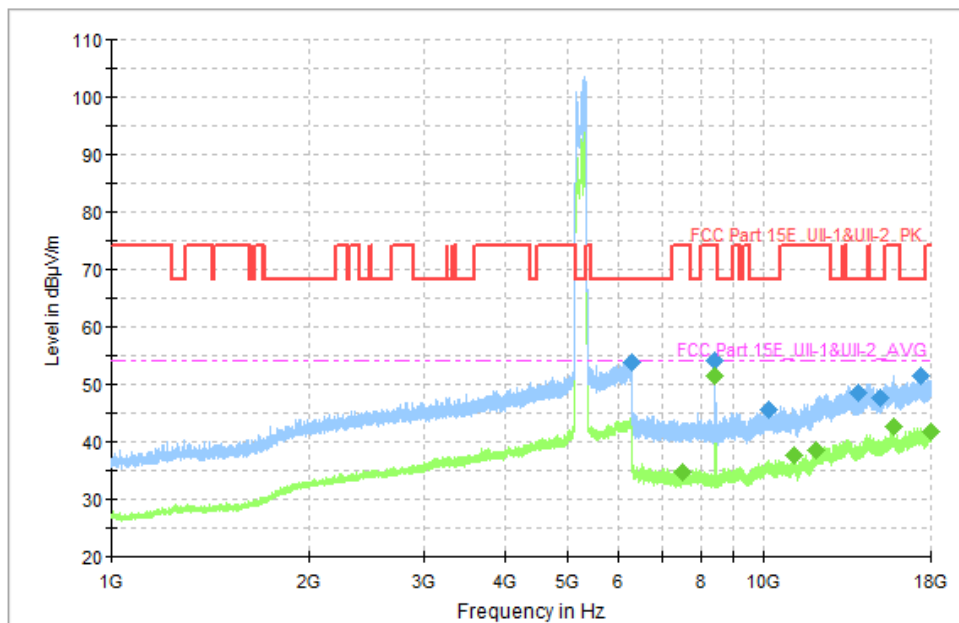
Fig. 41 Transmitter Spurious Emission (802.11n-HT40, CH54 5270MHz)
