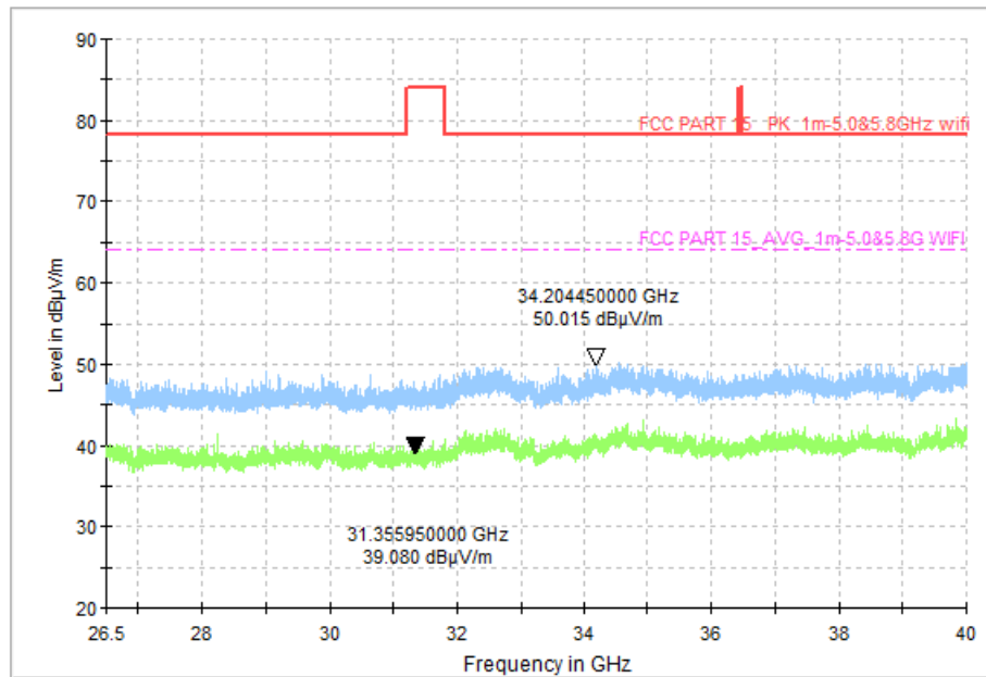
Fig. 50 Transmitter Spurious Emission (All channel, 26.5GHz~40GHz)
