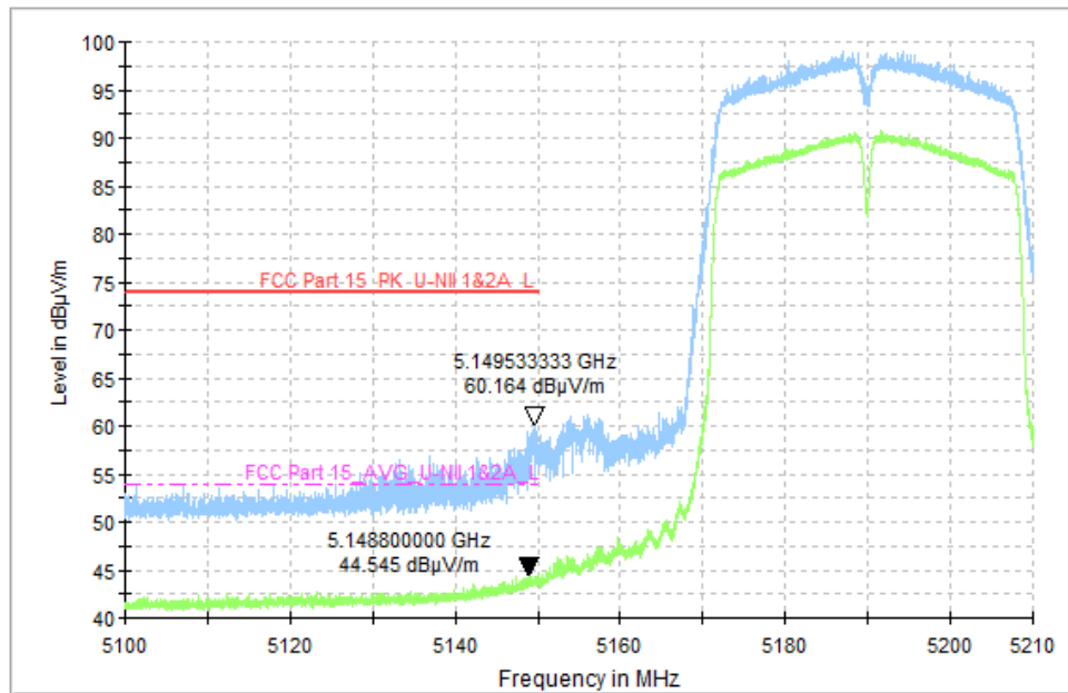
Fig. 23 Band Edges (802.11n-HT40, CH38 5190MHz)
