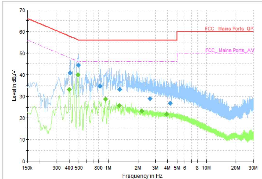
Fig. 52 AC Power line Conducted Emission (Traffic)
