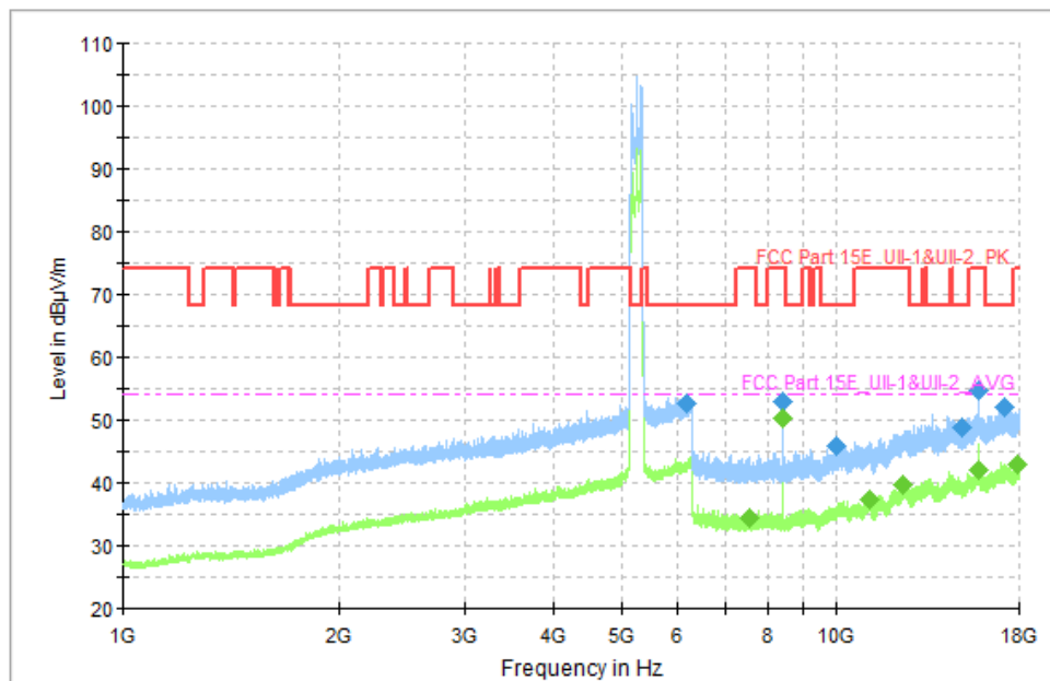
Fig. 33 Transmitter Spurious Emission (802.11a, CH52 5260MHz)
