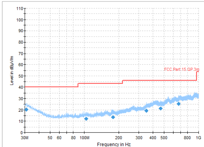
Fig. 48 Transmitter Spurious Emission (All channel, 30MHz~1GHz)
