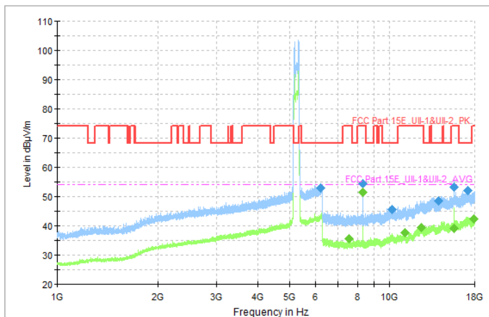
Fig. 31 Transmitter Spurious Emission (802.11a, CH40 5200MHz)
