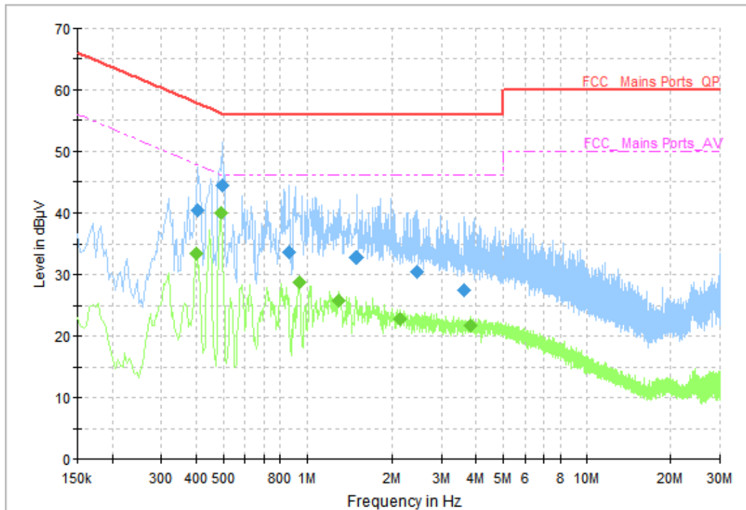
Fig. 53 AC Power line Conducted Emission (Idle)
