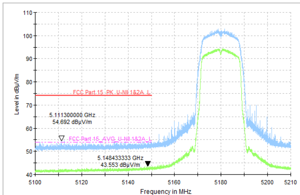
Fig. 19 Band Edges (802.11a, CH36 5180MHz)
