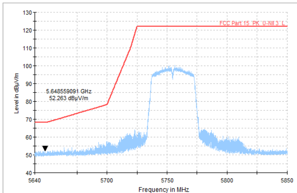
Fig. 25 Band Edges (802.11n-HT40, CH151 5755MHz)
