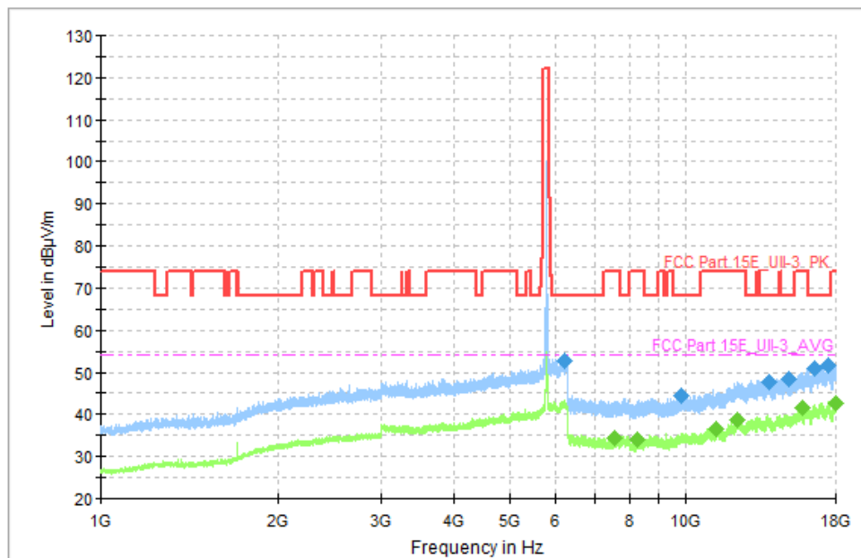
Fig. 37 Transmitter Spurious Emission (802. 11a, CH157 5785MHz)
