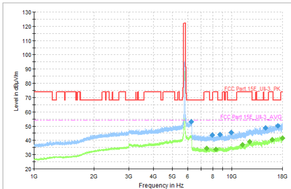
Fig. 47 Transmitter Spurious Emission (802.11ac-VHT80, CH155 5775MHz)
