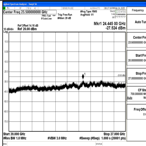
Band7_20MHz_QPSK_21100_1RB#0_20000~27000_20000~27000
