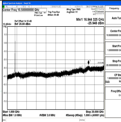
Band7_20MHz_QPSK_21100_1RB#0_1000~20000_1000~20000
