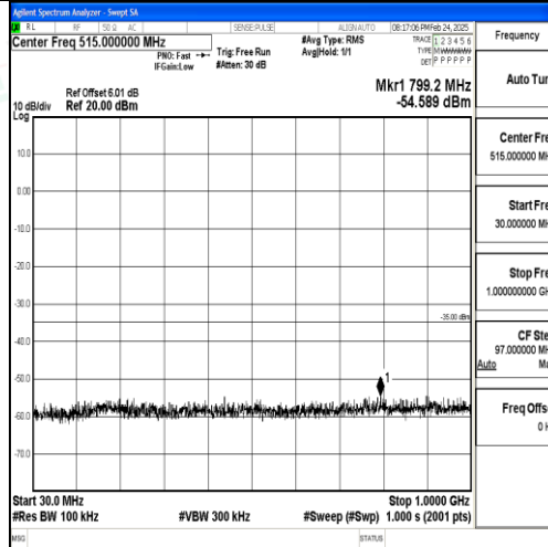
Band7_20MHz_QPSK_21100_1RB#0_30~1000_30~1000
