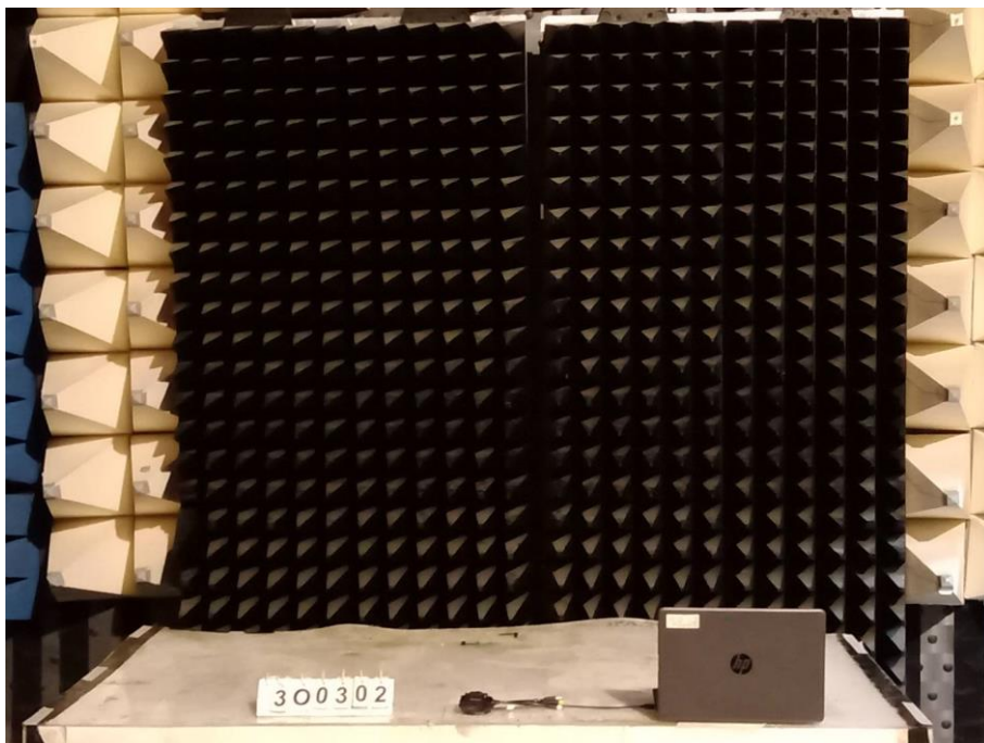
02. RE Rear View(Below 1GHz)
