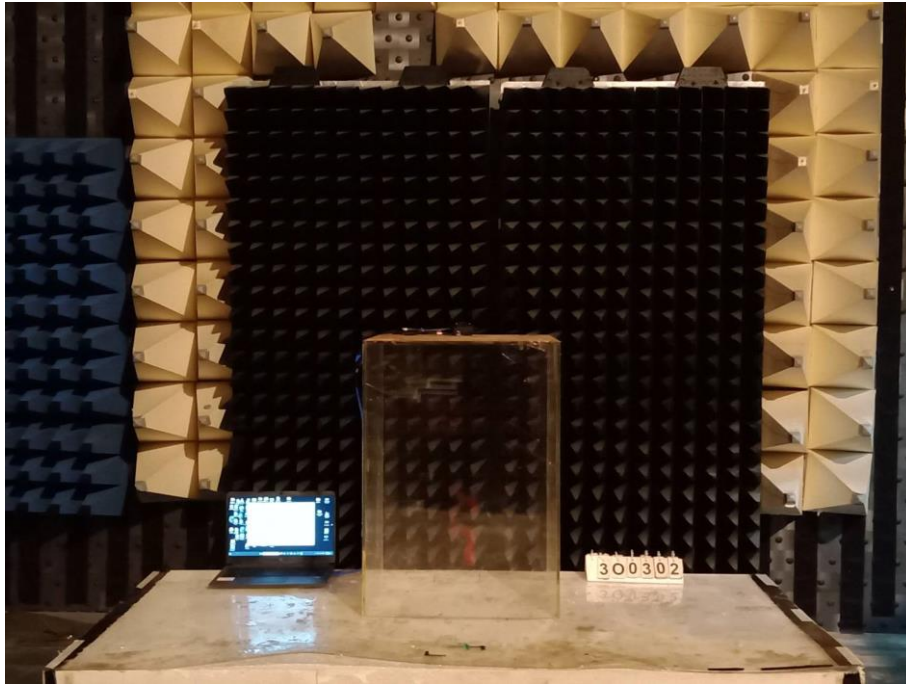
03. RE Front View(Above 1GHz)
