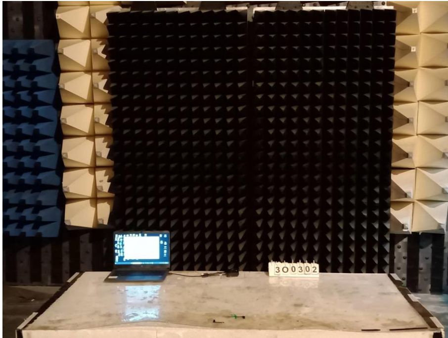
01. RE Front View(Below 1GHz)
