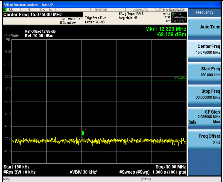
Band26_15MHz_16QAM_26865_1RB#74_0.15~30_0.15~30
