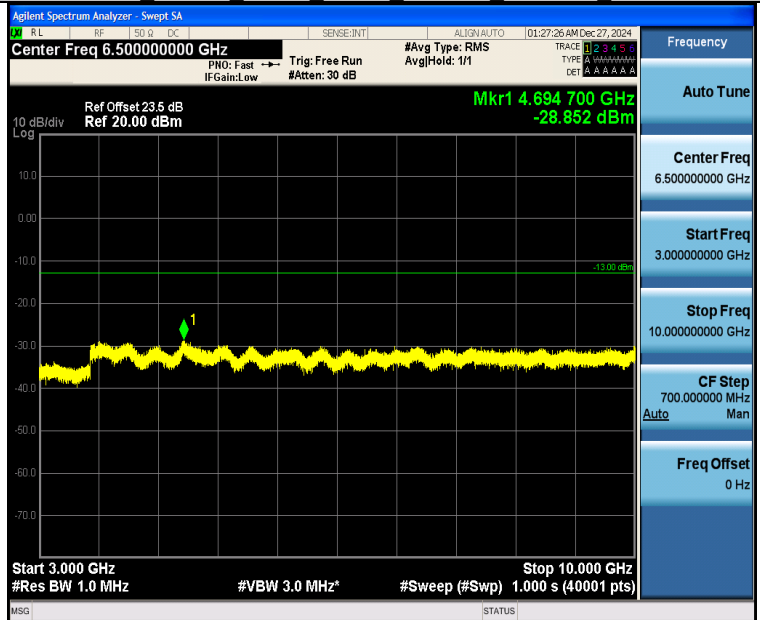
Band26_15MHz_QPSK_26865_1RB#74_3000~10000_3000~10000
