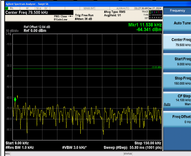
Band26_15MHz_16QAM_26865_1RB#74_0.009~0.15_0.009~0.15
