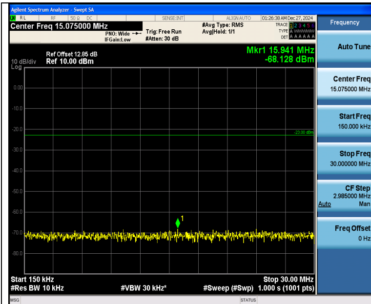
Band26_15MHz_QPSK_26865_1RB#74_0.15~30_0.15~30
