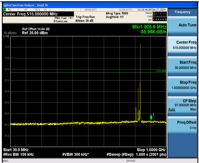
Band26_15MHz_QPSK_26865_1RB#74_30~1000_30~1000
