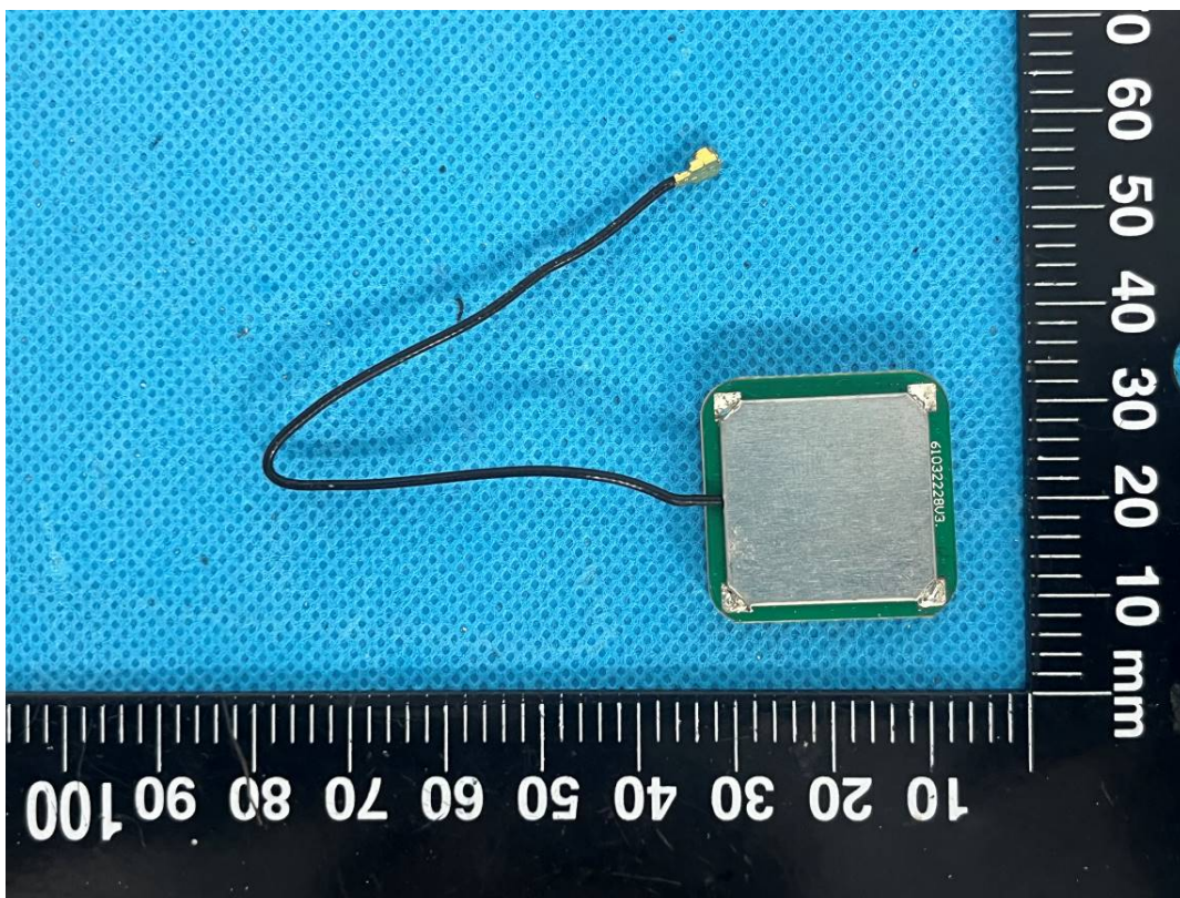
GPSAntenna
