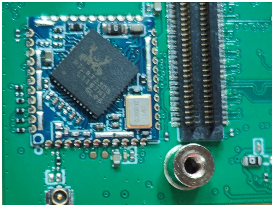
WIFI/BT chip
