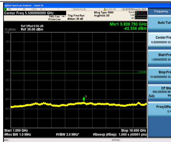
Band17_10MHz_16QAM_23780_1RB#0_1000~10000_1000~10000
