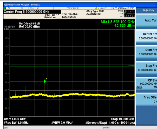
Band17_10MHz_QPSK_23790_1RB#0_1000~10000_1000~10000
