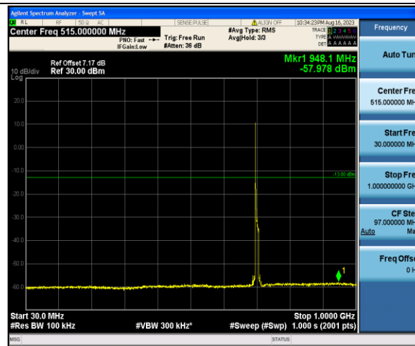
Band17_10MHz_QPSK_23780_1RB#0_30~1000_30~1000
