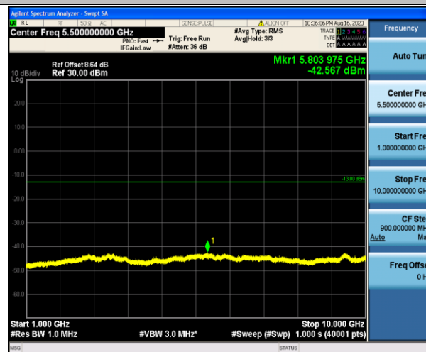
Band17_10MHz_16QAM_23790_1RB#0_1000~10000_1000~10000
