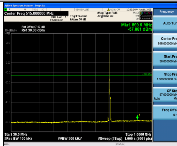
Band17_10MHz_QPSK_23790_1RB#0_30~1000_30~1000
