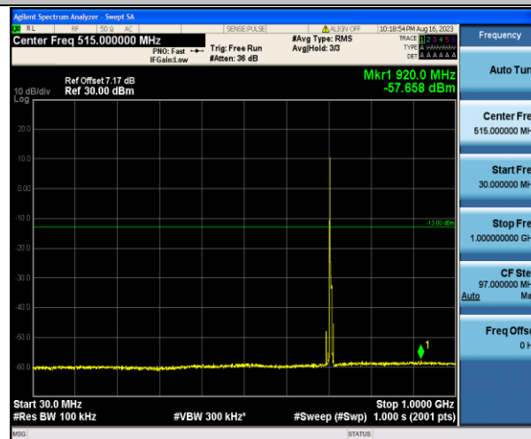
Band17_5MHz_16QAM_23825_1RB#0_30~1000_30~1000
