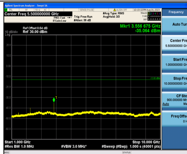
Band17_5MHz_16QAM_23825_1RB#0_1000~10000_1000~10000
