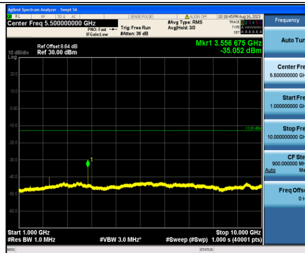
Band17_5MHz_QPSK_23825_1RB#0_1000~10000_1000~10000
