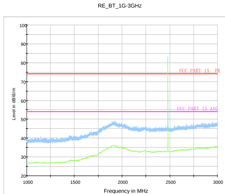
Fig.23. Radiated emission: GFSK, 2480MHz, 1 GHz - 3 GHz
