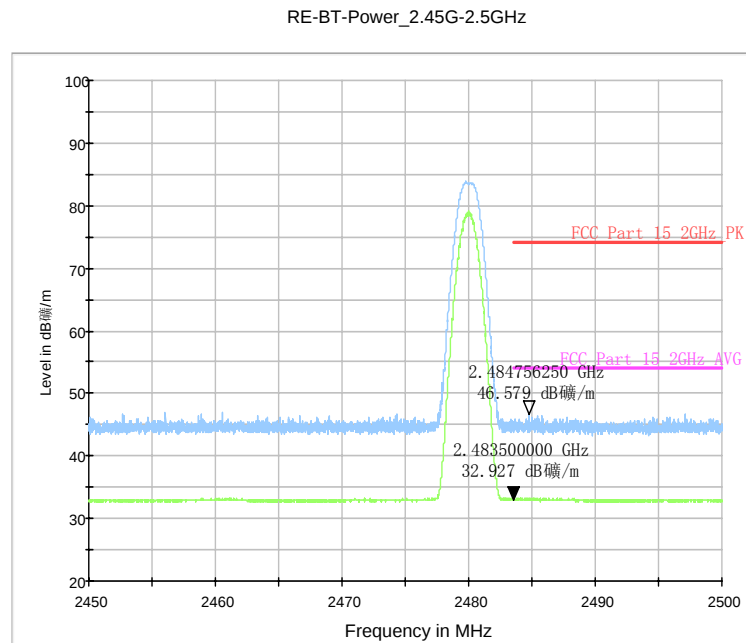
Fig.26. Radiated emission (Power): GFSK high channel
