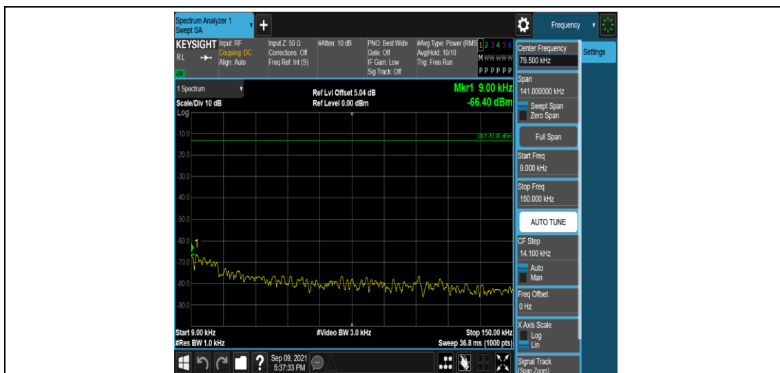
Band25-20MHz-16QAM-26590-1RB#0-Range1:0.009~0.15MHz
