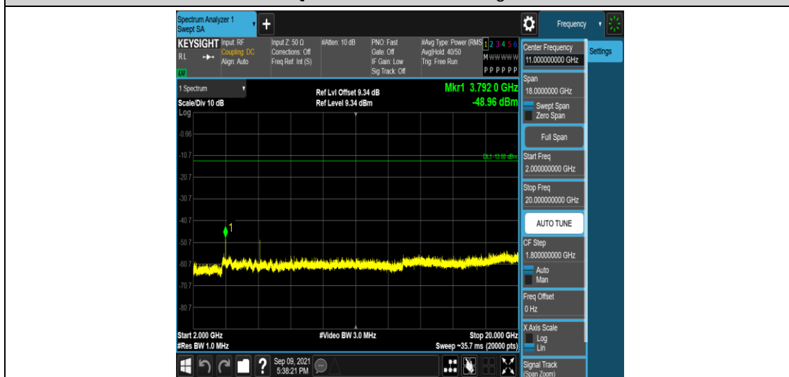
Band25-20MHz-16QAM-26590-1RB#0-Range5:2000~20000MHz
