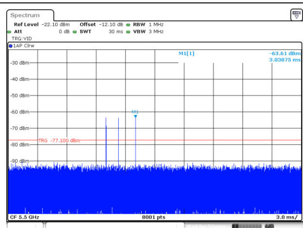
Radar #5 DFS detection threshold level
