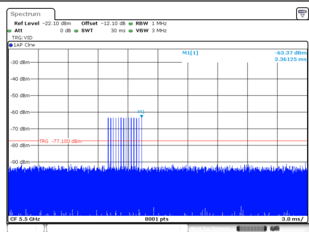
Radar #4 DFS detection threshold level
