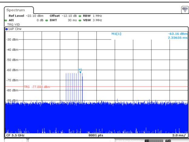
Radar #6 DFS detection threshold level
