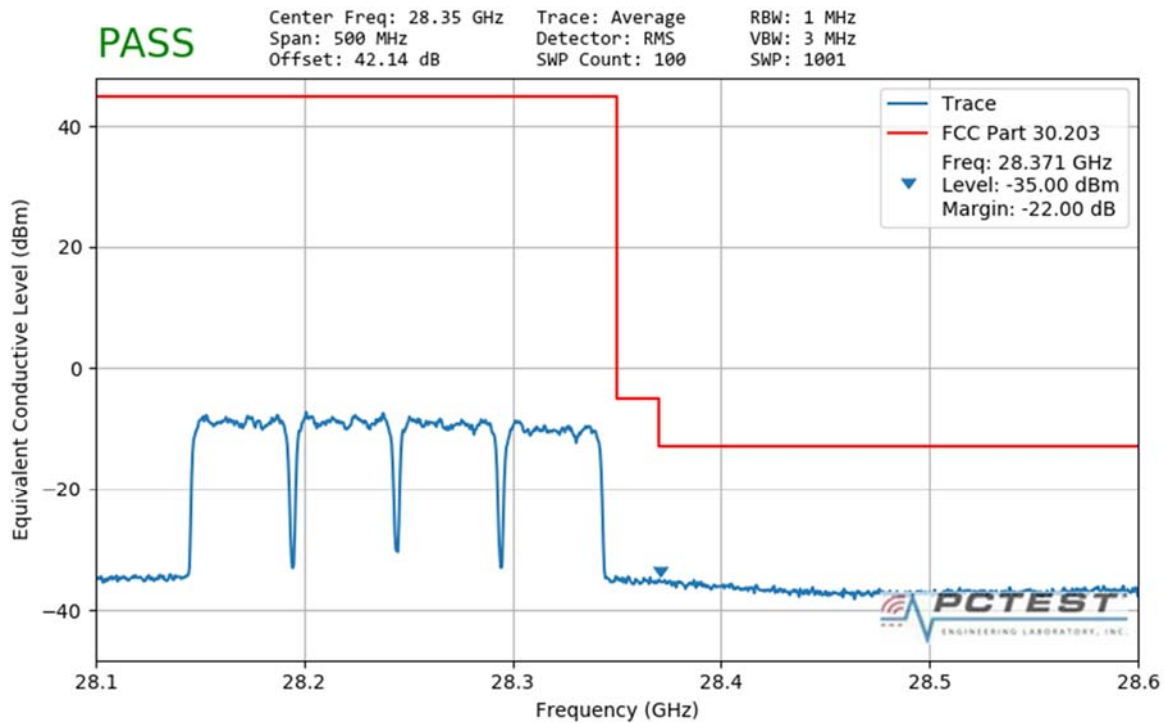
Plot 7-156. Ant3 Upper Band Edge (50MHz-4CC – QPSK Full RB)
