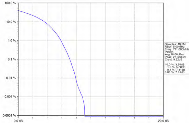
Band12_10MHz_64QAM_HCH_711MHz_RB_50_0_NTNV
