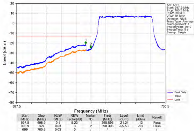
Band12_1.4MHz_16QAM_LCH_699.7MHz_RB_6_0_NTNV
