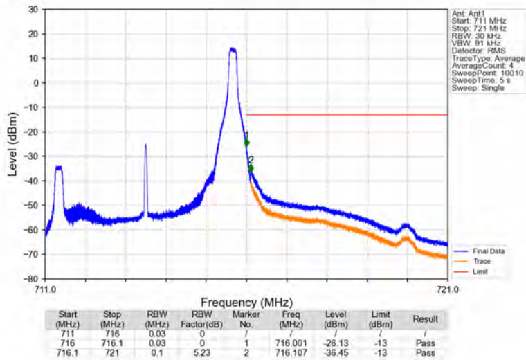
Band12_5MHz_64QAM_HCH_713.5MHz_RB_1_24_NTNV
