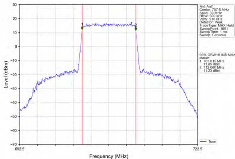
Band12_10MHz_16QAM_MCH_707.5MHz_RB_50_0_NTNV
