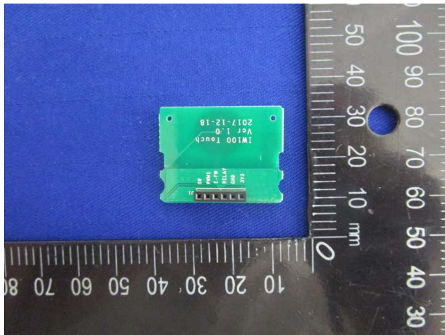
EUT –Touch Control Board Bottom View
