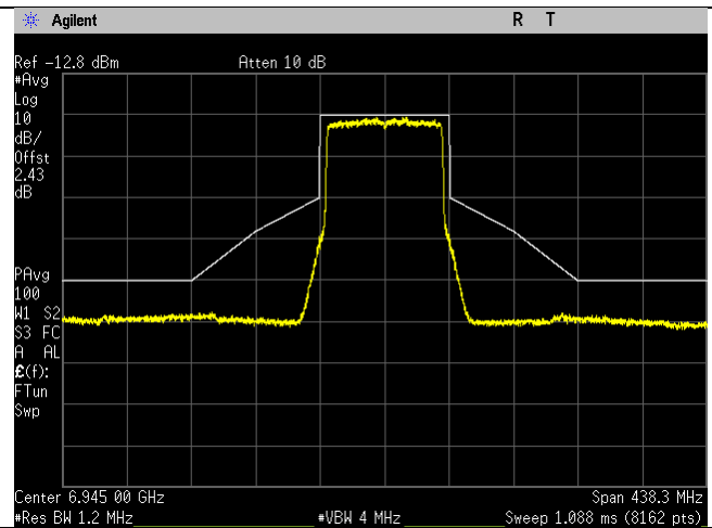
6945MHz_199_80MHz BW_be-mode_Chain 3
