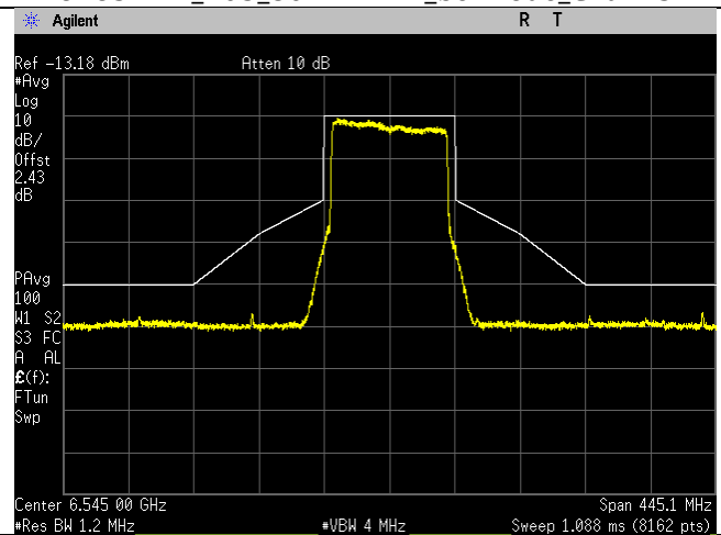
6545MHz_119_80MHz BW_be-mode_Chain 1
