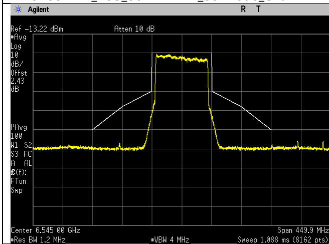
6545MHz_119_80MHz BW_be-mode_Chain 0
