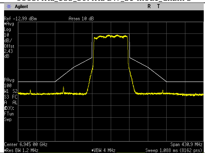
6945MHz_199_80MHz BW_be-mode_Chain 1
