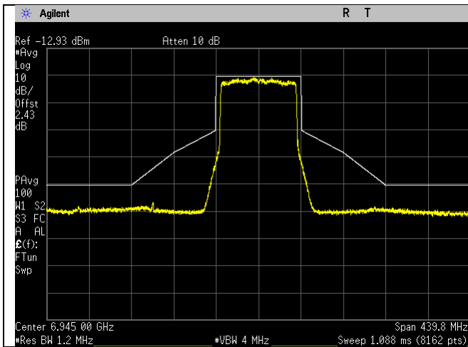
6945MHz_199_80MHz BW_be-mode_Chain 2
