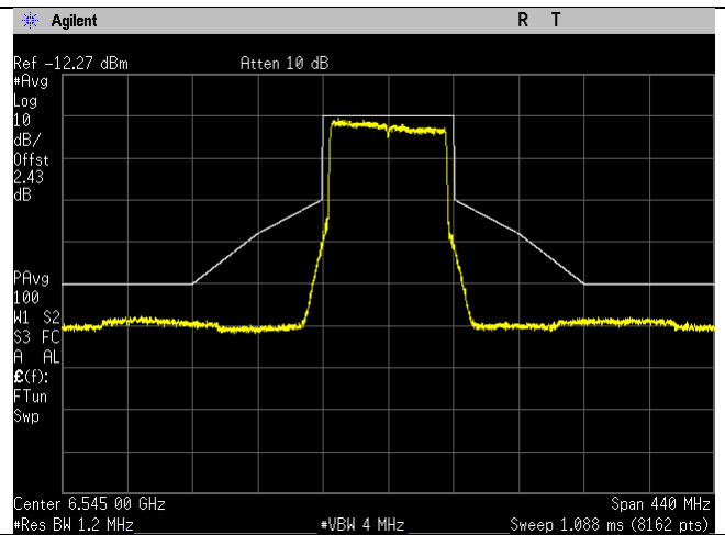
6545MHz_119_80MHz BW_be-mode_Chain 3
