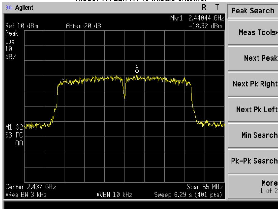
Mode: TX 11n HT40 middle channel
