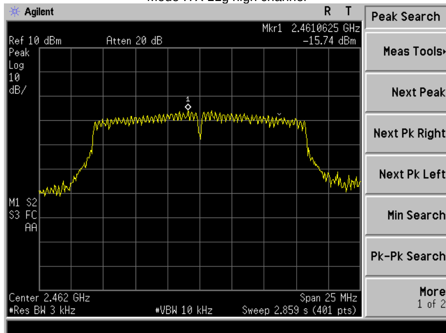
Mode :TX 11g high channel
