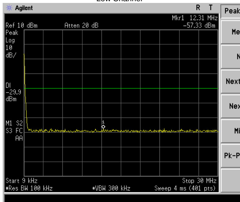
802.11n40 Low Channel
