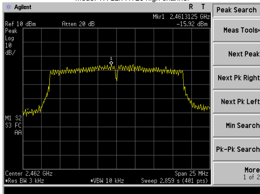
Mode: TX 11n HT20 high channel
