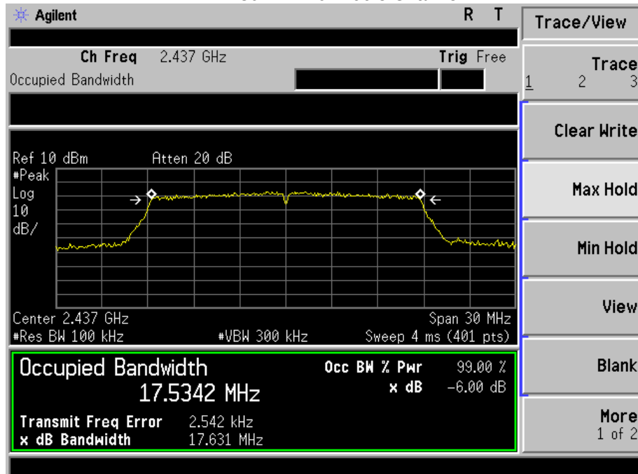
802.11n20 Middle Channel
