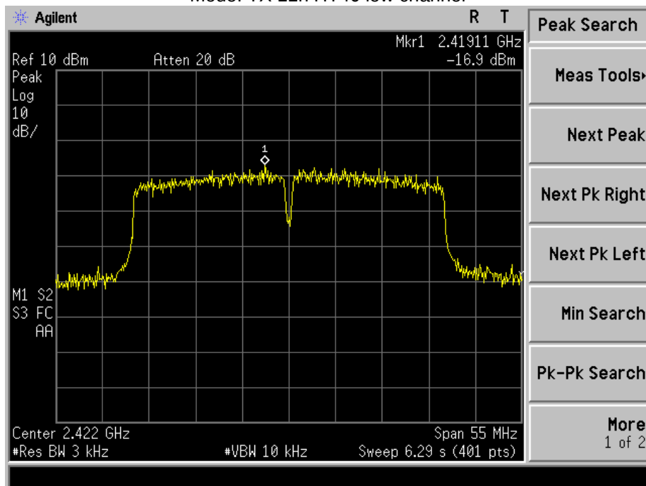
Mode: TX 11n HT40 low channel
