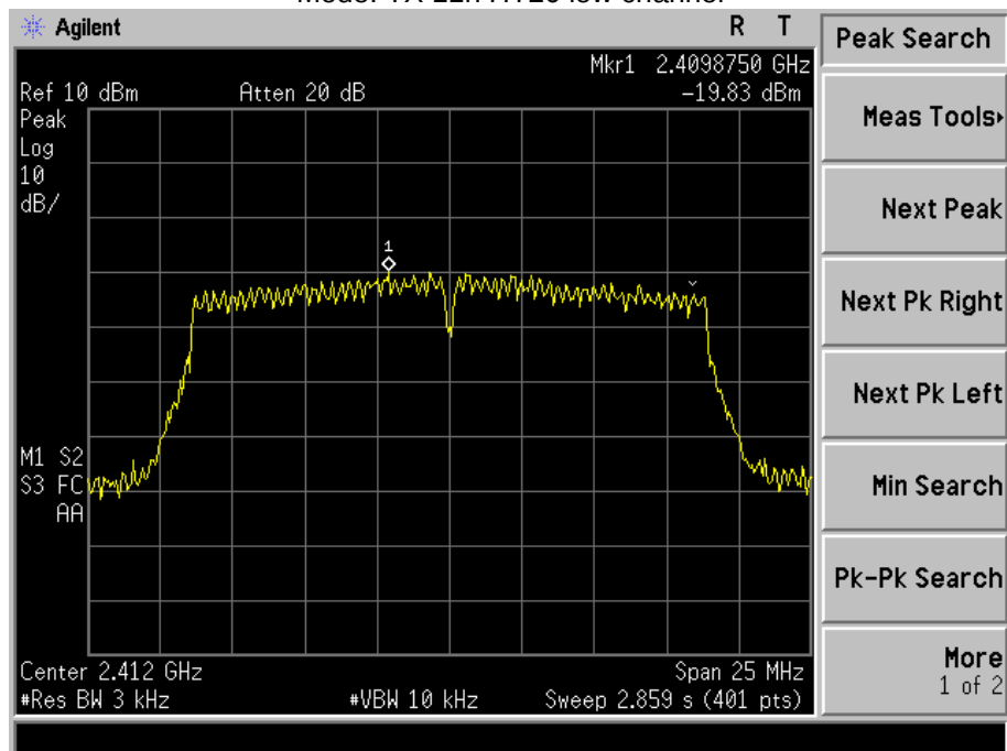
Mode: TX 11n HT20 low channel
