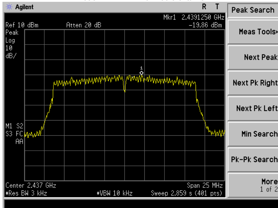
Mode: TX 11n HT20 middle channel
