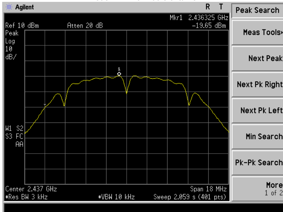
Mode: TX 11b middle channel
