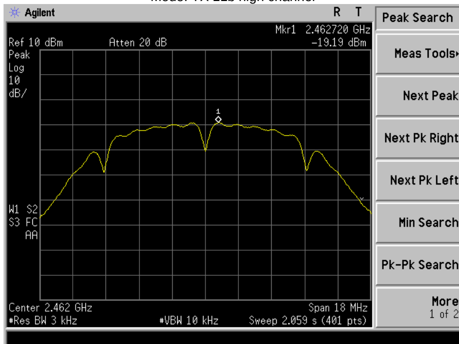
Mode: TX 11b high channel
