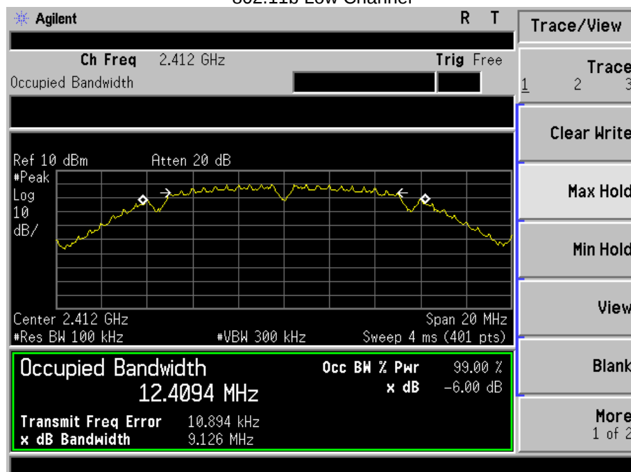
Test plots 802.11b Low Channel
