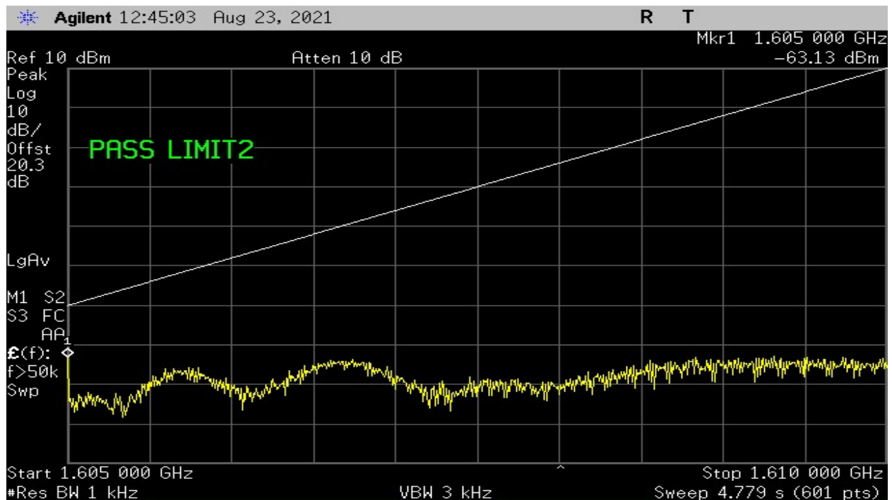
Plot 22-High Channel – Test Limit 25.216 (f)(g) – Discrete Emissions
