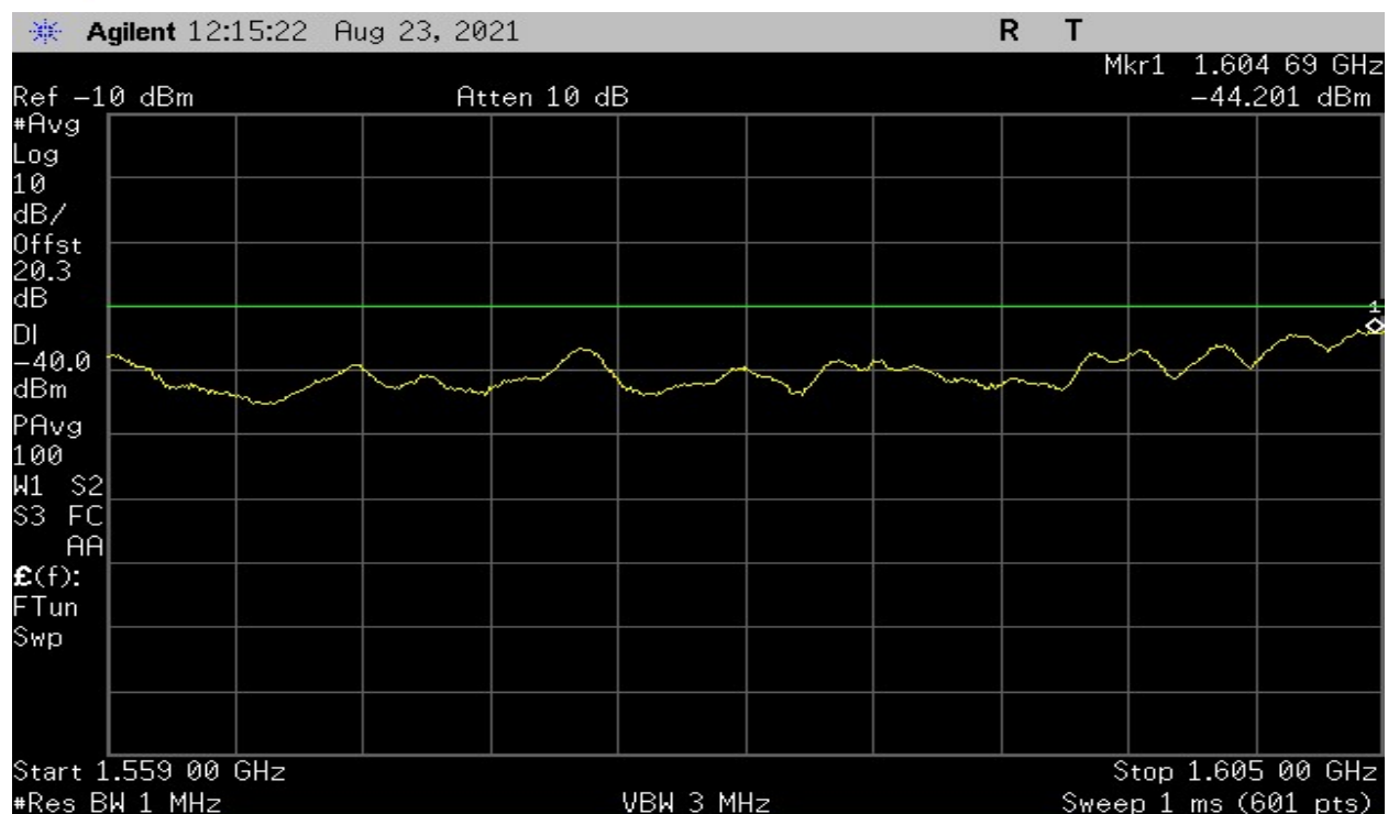
Plot 19 – Low Channel – Test Limit 25.216 (c)
