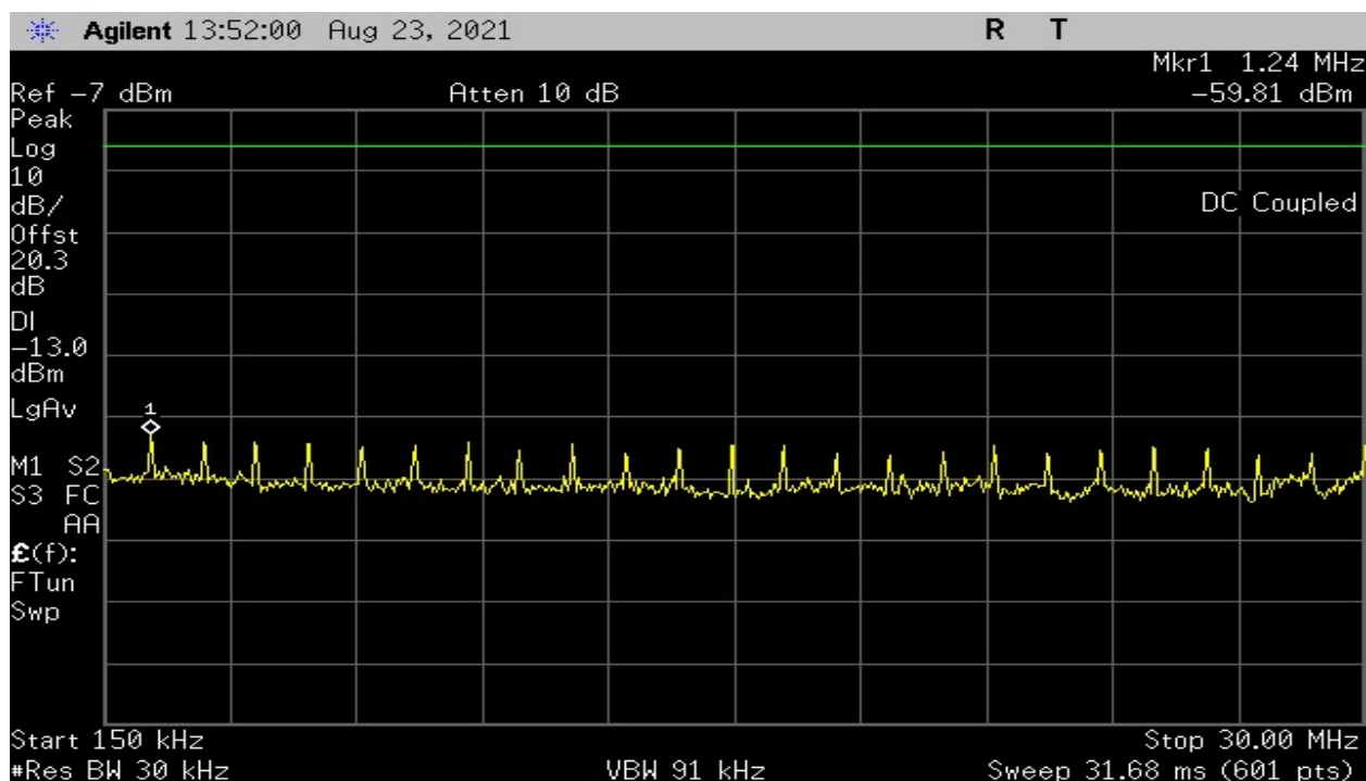
Plot 12 – Highest Channel – 150kHz to 30MHz
