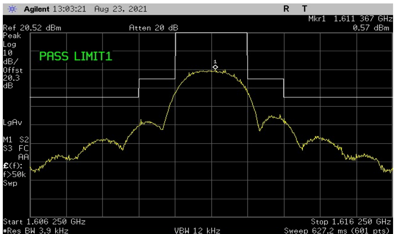
Plot 5 – Emission Mask – Low Channel
