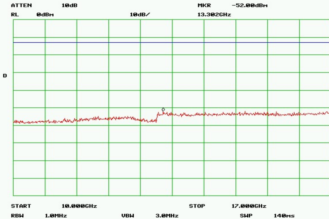
Plot 11 – Lowest Channel - 10GHz to 17GHz
