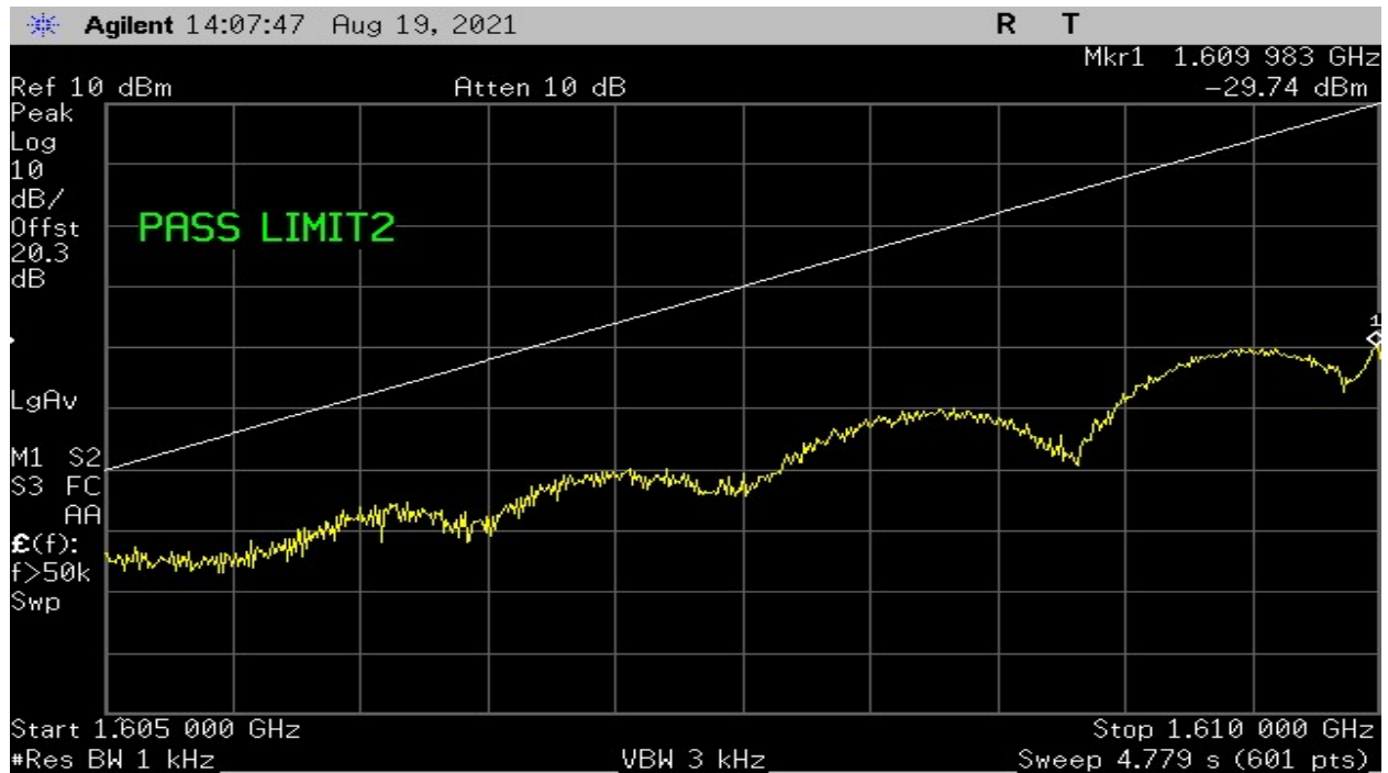
Plot 21- Low Channel – Test Limit 25.216 (f)(g) – Discrete Emissions
