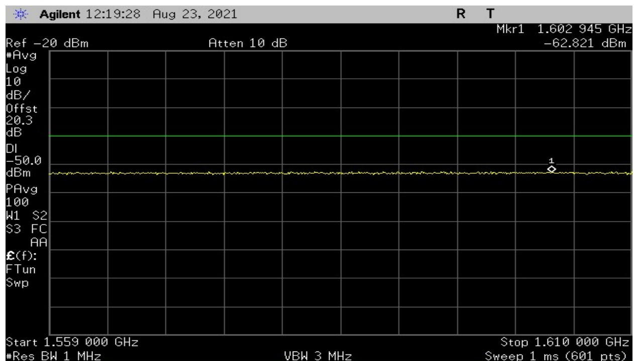
Plot 25- Low Channel - Carrier Off
