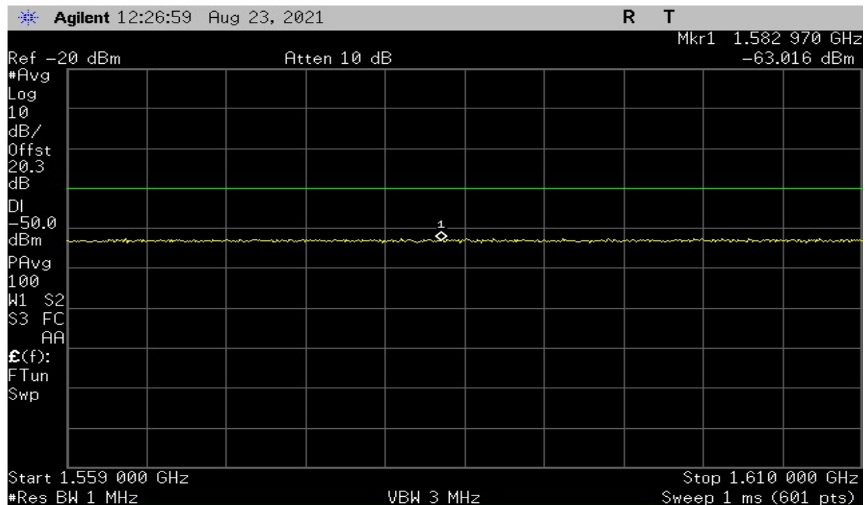
Plot 26 – High Channel – Carrier Off
