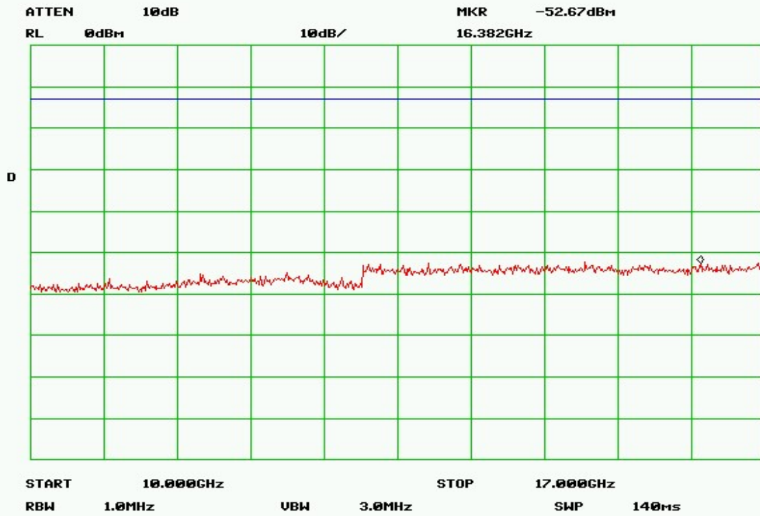
Plot 16 Highest Channel - 10GHz to 17GHz
