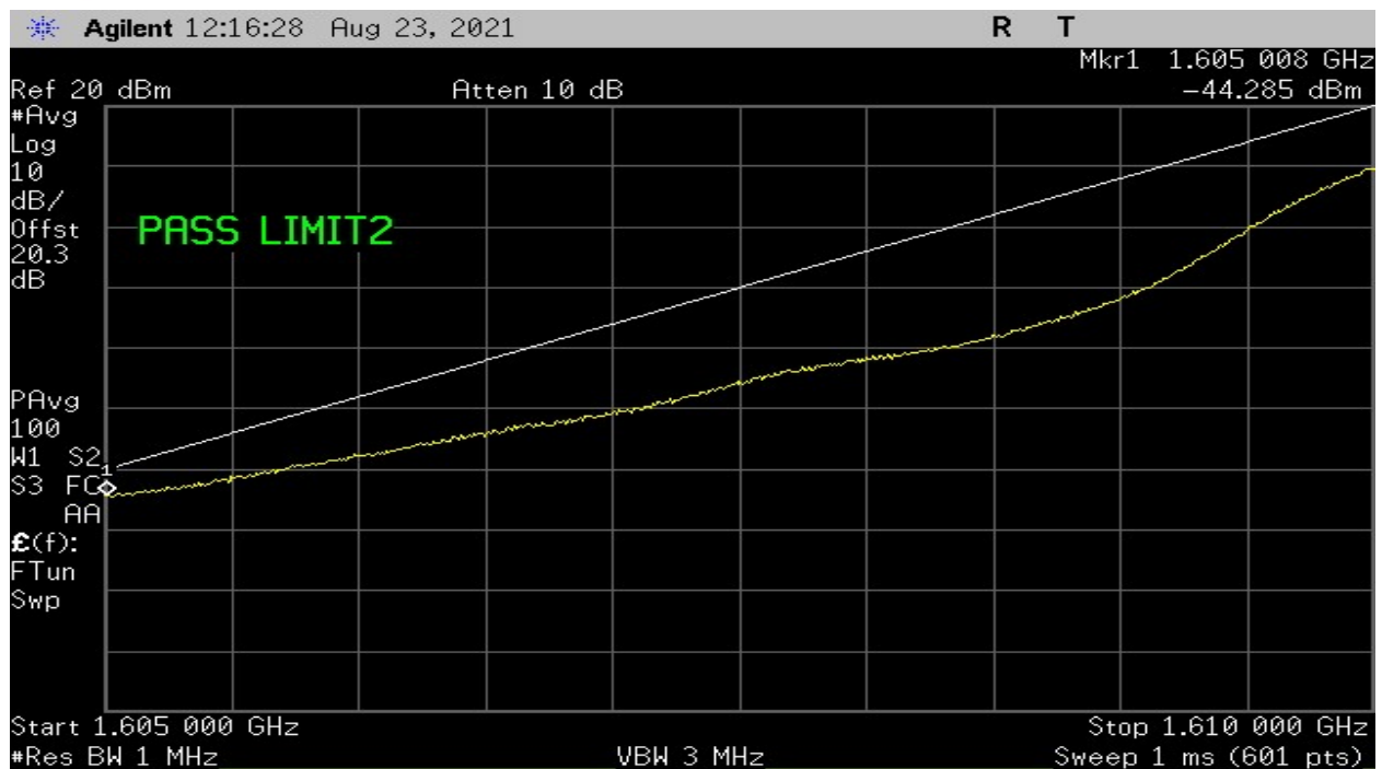
Plot 23- Low Channel – Test Limit 25.216 (f)(g)
