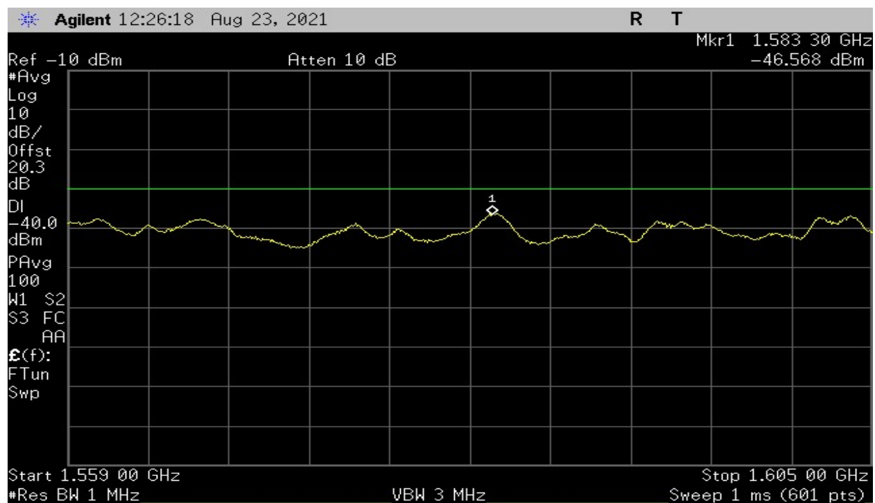
Plot 20 – High Channel – Test Limit 25.216 (c)
