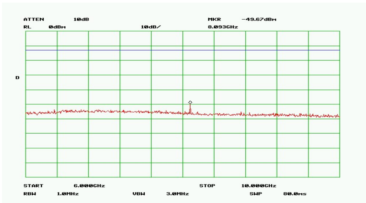
Plot 15 Highest Channel - 6GHz to 10GHz
