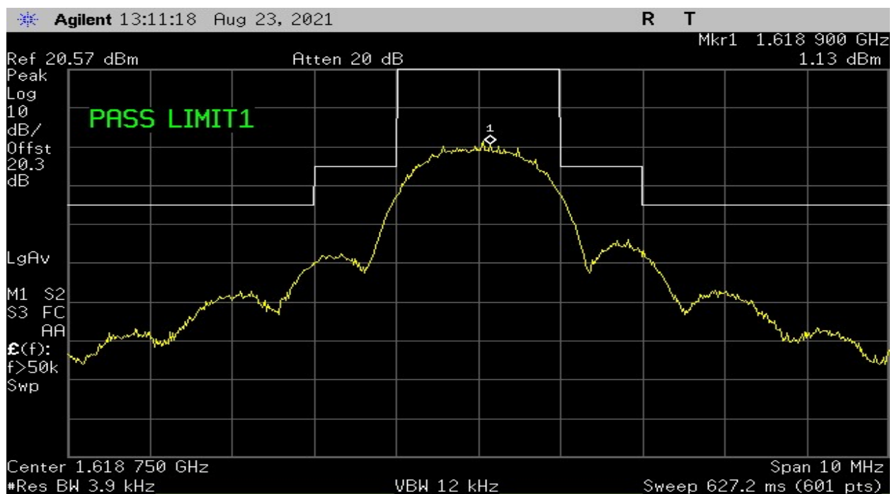
Plot 6 – Emission Mask - High Channel
