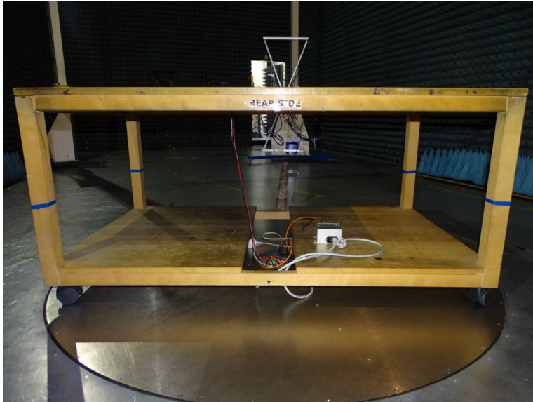
Photo 3: Test setup for radiated measurements
