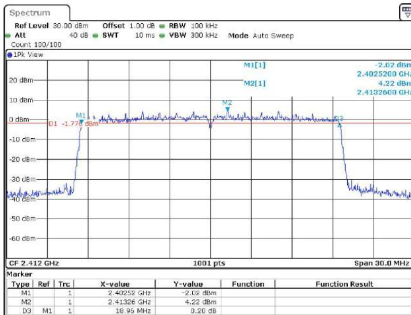
11AX20SISO-242T_Ant1_2412
