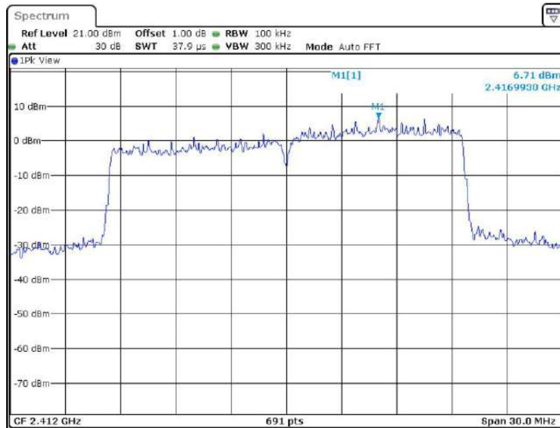
11AX20SISO-242T_Ant1_2412_0~Reference
