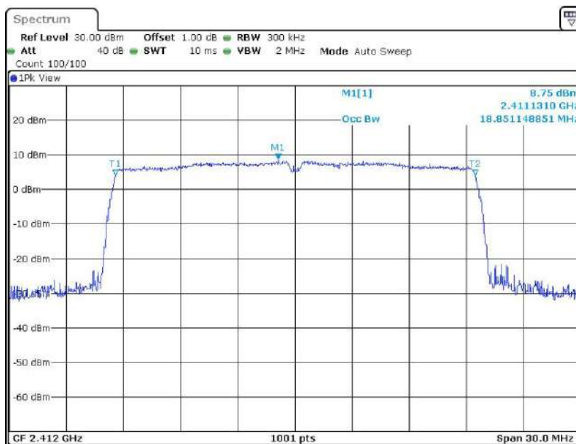
11AX20SISO-242T_Ant1_2412
