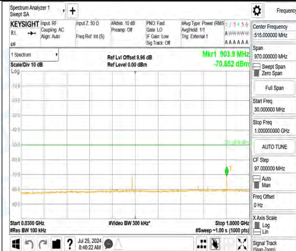
Band40_5MHz_QPSK_38775_1RB#0_3000~26500_3000~26500
