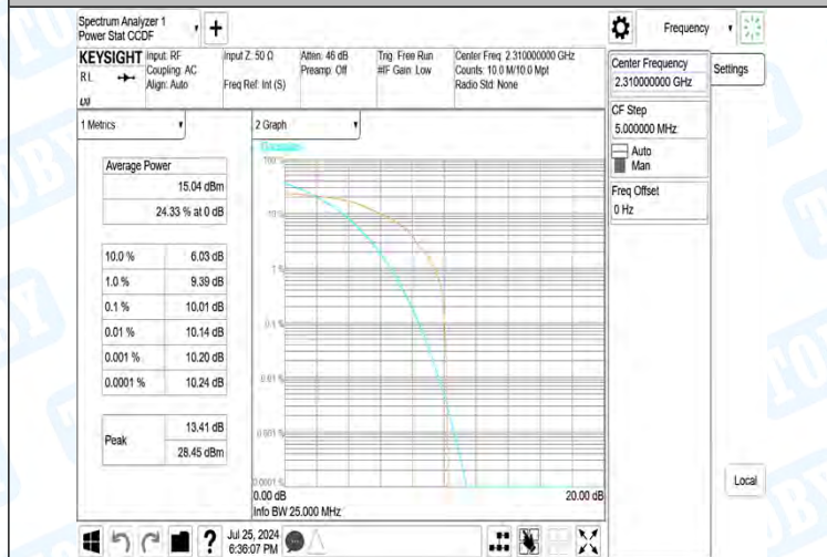
40(2305-2315)-5MHz-16QAM-38775-1RB#0-PASS
