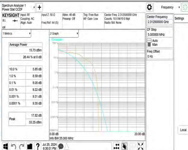
40(2305-2315)-5MHz-16QAM-38725-1RB#0-PASS
