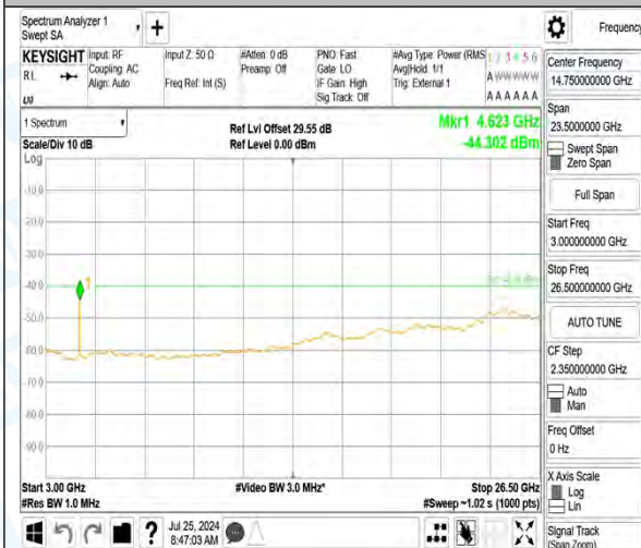
Band40_5MHz_16QAM_38725_1RB#0_0.15~30_0.15~30
