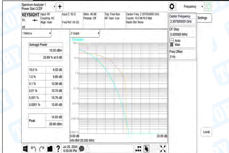
40(2305-2315)-5MHz-16QAM-38750-1RB#0-PASS
