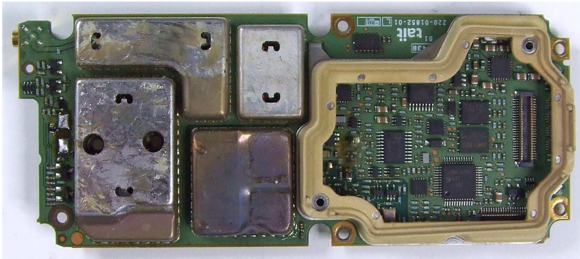
Photograph 02: Rx-Tx PCB - top (with shields)
