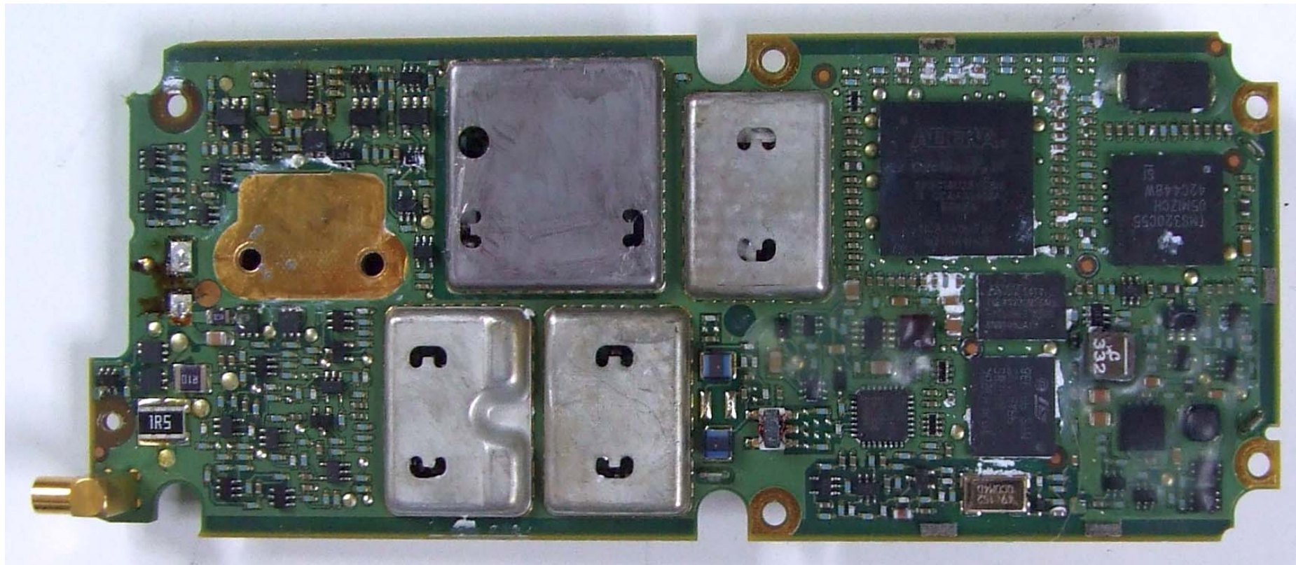
Photograph 04: Rx-Tx PCB - bottom (with shields)
