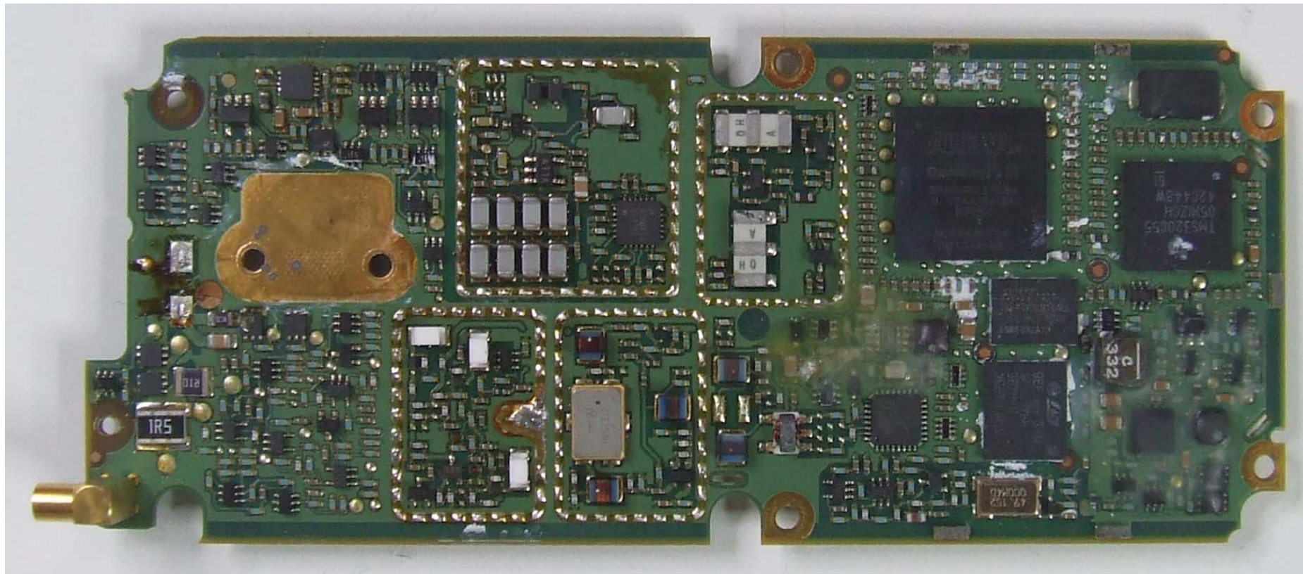
Photograph 05: Rx-Tx PCB - bottom (without shields)
