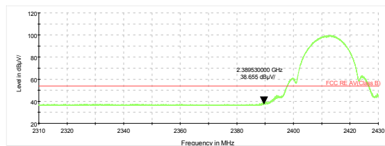
802.11b-Channel 1 Average
