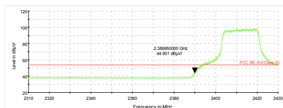
802.11g-Channel 1 Average
