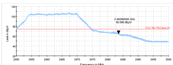
802.11g-Channel 11 Peak
