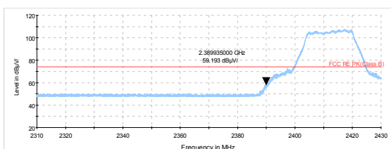
802.11g-Channel 1 Peak
