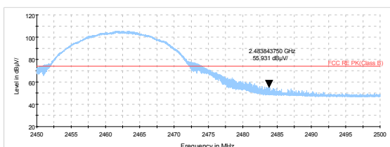
802.11b-Channel 11 Peak
