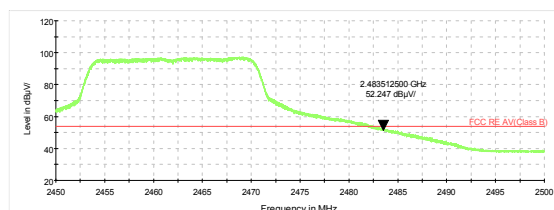
802.11g-Channel 11 Average
