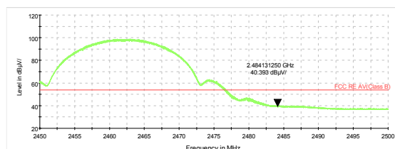
802.11b-Channel 11 Average
