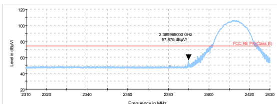
802.11b-Channel 1 Peak
