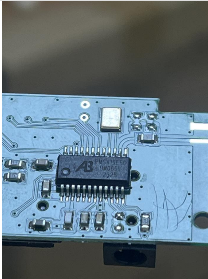
RF IC:PMSA15E5C
