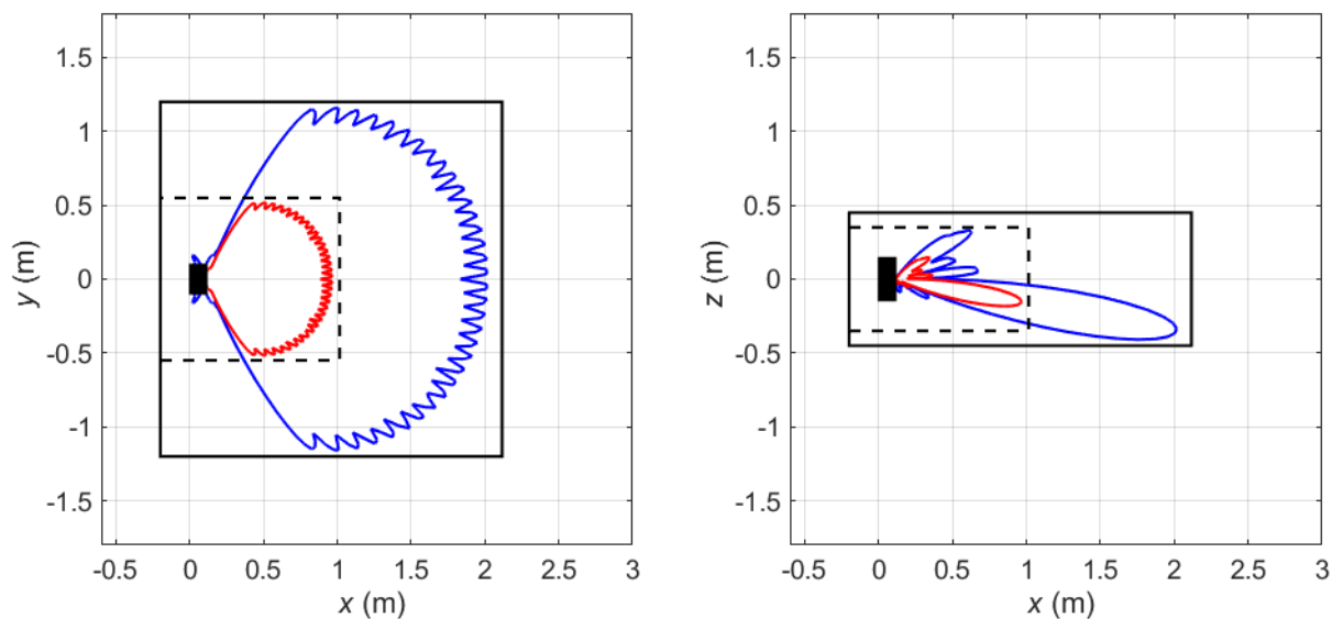
Figure 13 Compliance boundaries for general public (black solid line) and occupational (black dashed line) exposure for markets where the FCC exposure limits apply for Macro11 (tilt 7.5^\circ ) sector shape (Configuration Mode 2). The blue solid lines correspond to compliance distance results for general public exposure obtained using the spherical models. The solid red lines indicate the corresponding compliance distance results for occupational exposure. The EUT is shown from above (left) and from the side (right) with its backplane located at x = 0 m. Mode: B258 (26 GHz) (NR). Total EIRP of the radio: 57.2 dBm.
