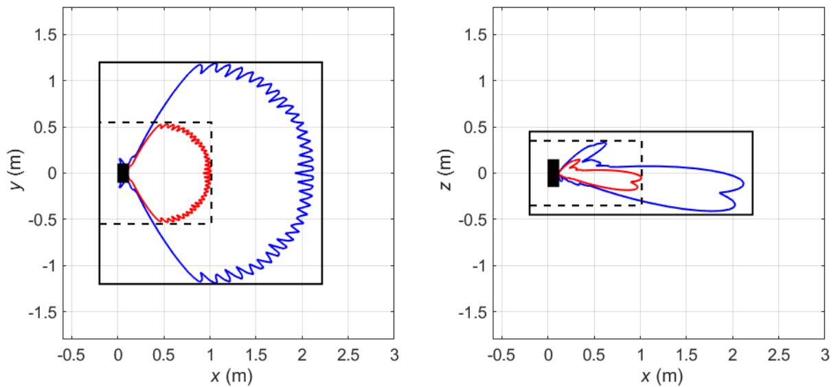
Figure 11 Compliance boundaries for general public (black solid line) and occupational (black dashed line) exposure for markets where the FCC exposure limits apply for Macro10 sector shape (Configuration Mode 2). The blue solid lines correspond to compliance distance results for general public exposure obtained using the spherical models. The solid red lines indicate the corresponding compliance distance results for occupational exposure. The EUT is shown from above (left) and from the side (right) with its backplane located at x = 0 m. Mode: B258 (26 GHz) (NR). Total EIRP of the radio: 57.2 dBm.
