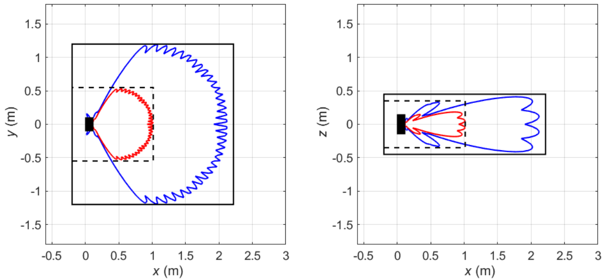
Figure 6 Compliance boundaries for general public (black solid line) and occupational (black dashed line) exposure for markets where the FCC exposure limits apply for Hotspot2 sector shape (Configuration Mode 2). The blue solid lines correspond to compliance distance results for general public exposure obtained using the spherical models. The solid red lines indicate the corresponding compliance distance results for occupational exposure. The EUT is shown from above (left) and from the side (right) with its backplane located at x = 0 m. Mode: B258 (26 GHz) (NR). Total EIRP of the radio: 57.2 dBm.
