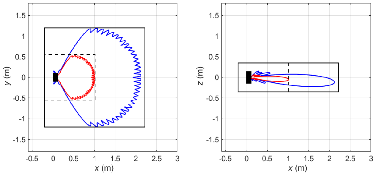
Figure 9 Compliance boundaries for general public (black solid line) and occupational (black dashed line) exposure for markets where the FCC exposure limits apply for Macro9 sector shape (Configuration Mode 2). The blue solid lines correspond to compliance distance results for general public exposure obtained using the spherical models. The solid red lines indicate the corresponding compliance distance results for occupational exposure. The EUT is shown from above (left) and from the side (right) with its backplane located at x = 0 m. Mode: B258 (26 GHz) (NR). Total EIRP of the radio: 57.2 dBm.
