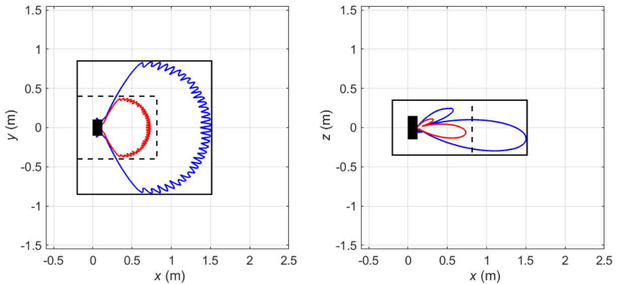
Figure 4 Compliance boundaries for general public (black solid line) and occupational (black dashed line) exposure for markets where the FCC exposure limits apply for Macro3 sector shape (Configuration Mode 1). The blue solid lines correspond to compliance distance results for general public exposure obtained using the spherical models. The solid red lines indicate the corresponding compliance distance results for occupational exposure. The EUT is shown from above (left) and from the side (right) with its backplane located at x = 0 m. Mode: B258 (26 GHz) (NR). Total EIRP of the radio: 54.2 dBm.
