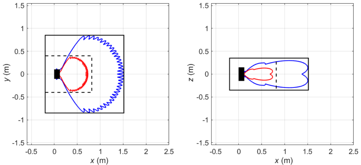
Figure 3 Compliance boundaries for general public (black solid line) and occupational (black dashed line) exposure for markets where the FCC exposure limits apply for Hotspot5 sector shape (Configuration Mode 1). The blue solid lines correspond to compliance distance results for general public exposure obtained using the spherical models. The solid red lines indicate the corresponding compliance distance results for occupational exposure. The EUT is shown from above (left) and from the side (right) with its backplane located at x = 0 m. Mode: B258 (26 GHz) (NR). Total EIRP of the radio: 54.2 dBm.
