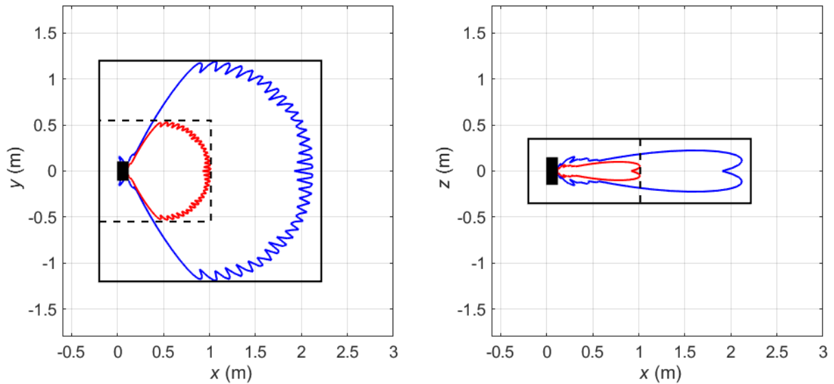
Figure 7 Compliance boundaries for general public (black solid line) and occupational (black dashed line) exposure for markets where the FCC exposure limits apply for Macro3 sector shape (Configuration Mode 2). The blue solid lines correspond to compliance distance results for general public exposure obtained using the spherical models. The solid red lines indicate the corresponding compliance distance results for occupational exposure. The EUT is shown from above (left) and from the side (right) with its backplane located at x = 0 m. Mode: B258 (26 GHz) (NR). Total EIRP of the radio: 57.2 dBm.
