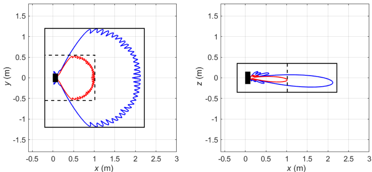
Figure 12 Compliance boundaries for general public (black solid line) and occupational (black dashed line) exposure for markets where the FCC exposure limits apply for Macro11 sector shape (Configuration Mode 2). The blue solid lines correspond to compliance distance results for general public exposure obtained using the spherical models. The solid red lines indicate the corresponding compliance distance results for occupational exposure. The EUT is shown from above (left) and from the side (right) with its backplane located at x = 0 m. Mode: B258 (26 GHz) (NR). Total EIRP of the radio: 57.2 dBm.
