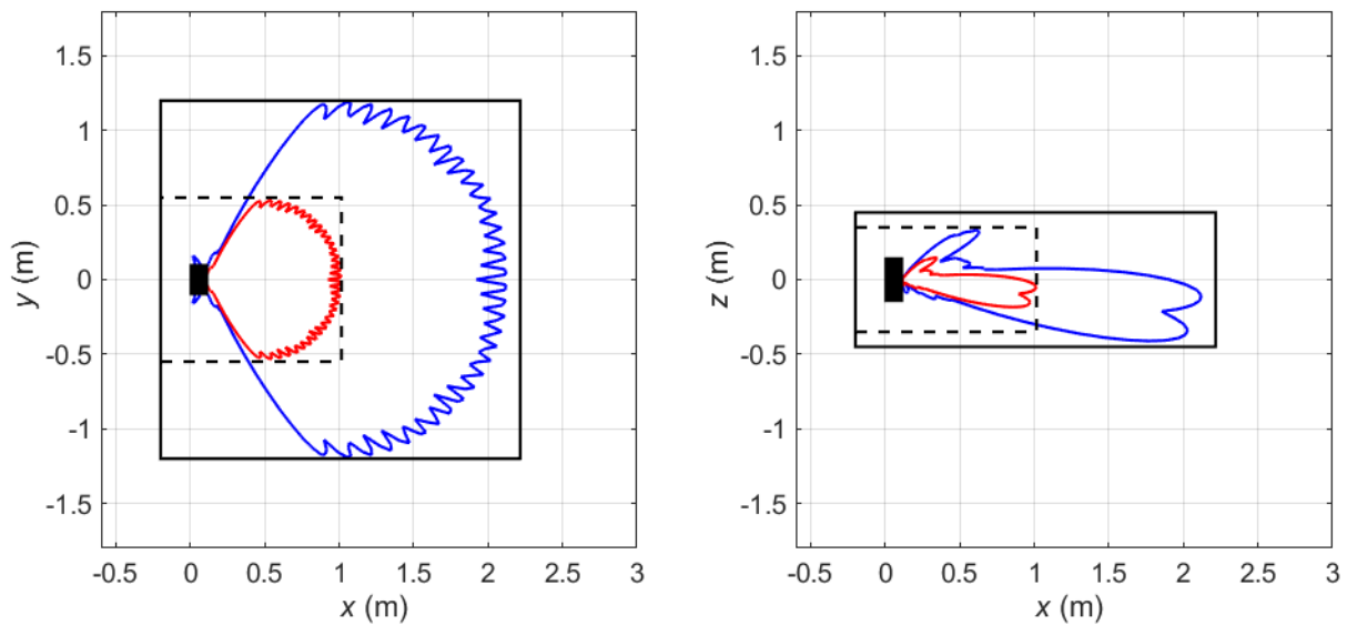
Figure 8 Compliance boundaries for general public (black solid line) and occupational (black dashed line) exposure for markets where the FCC exposure limits apply for Macro3 (tilt 7.5°) sector shape (Configuration Mode 2). The blue solid lines correspond to compliance distance results for general public exposure obtained using the spherical models. The solid red lines indicate the corresponding compliance distance results for occupational exposure. The EUT is shown from above (left) and from the side (right) with its backplane located at x = 0 m. Mode: B258 (26 GHz) (NR). Total EIRP of the radio: 57.2 dBm.
