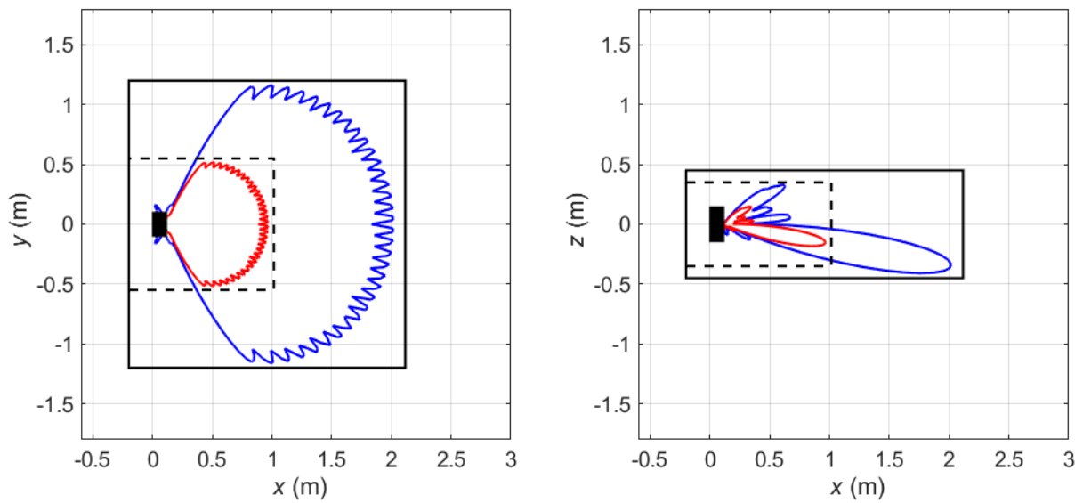
Figure 10 Compliance boundaries for general public (black solid line) and occupational (black dashed line) exposure for markets where the FCC exposure limits apply for Macro9 (tilt 7.5°) sector shape (Configuration Mode 2). The blue solid lines correspond to compliance distance results for general public exposure obtained using the spherical models. The solid red lines indicate the corresponding compliance distance results for occupational exposure. The EUT is shown from above (left) and from the side (right) with its backplane located at x = 0 m. Mode: B258 (26 GHz) (NR). Total EIRP of the radio: 57.2 dBm.
