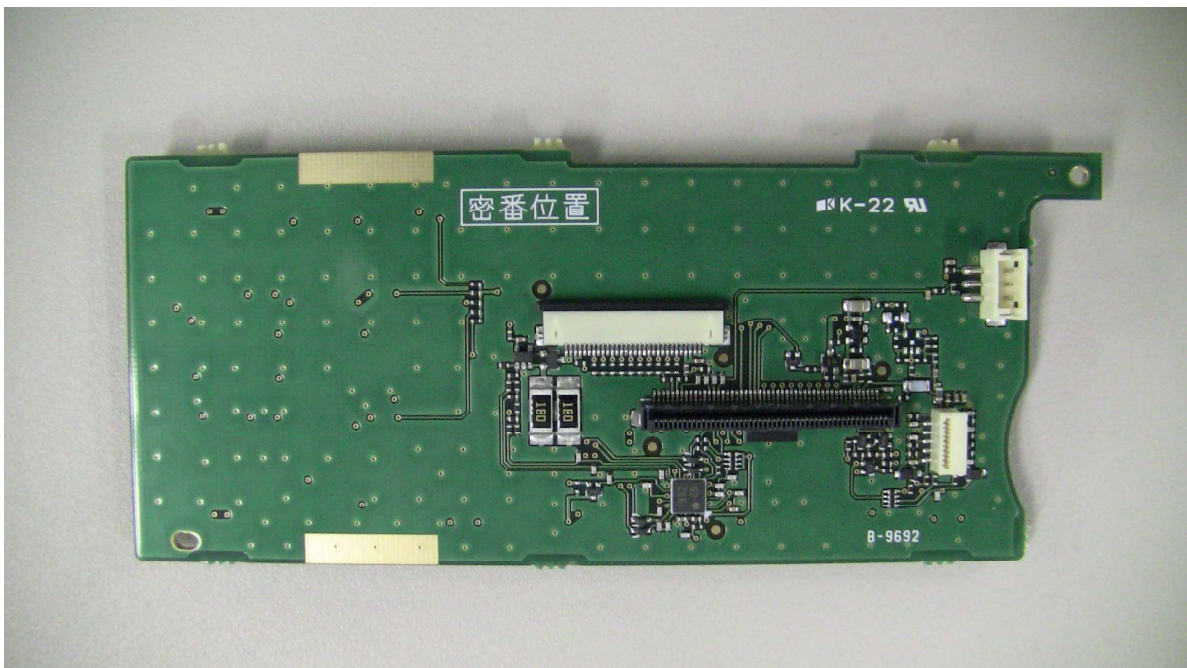
IC-F7520 FRONT-A UNIT B SIDE
