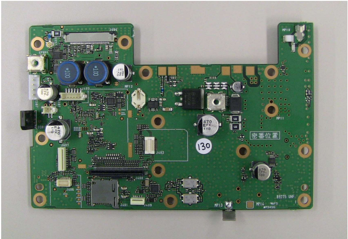
IC-F7520 MAIN-D UNIT A SIDE
