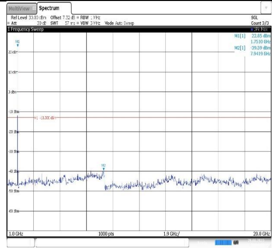
Band4-5MHz-16QAM-19975-1RB#0- Range2:1000~20000MHz
