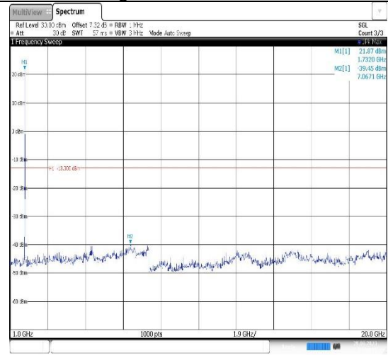
Band4-15MHz-QPSK-20175-1RB#0- Range2:1000~20000MHz
