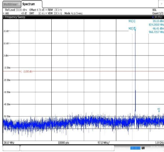
Band5-1.4MHz-16QAM-20407-1RB#0- Range1:30~1000MHz
