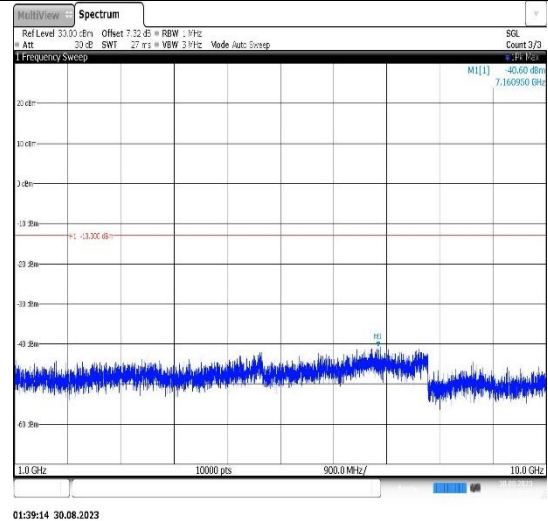
Band5-5MHz-QPSK-20625-1RB#0- Range2:1000~10000MHz
