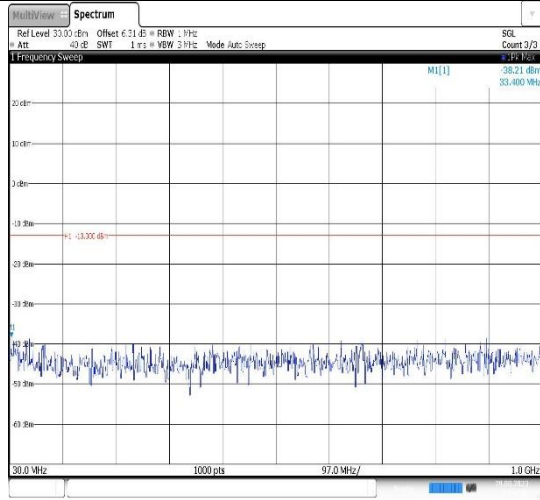
Band4-20MHz-QPSK-20175-1RB#0- Range1:30~1000MHz
