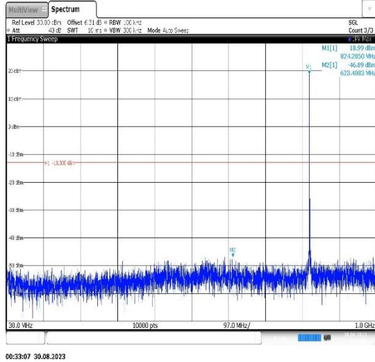
Band5-1.4MHz-QPSK-20525-1RB#0- Range1:30~1000MHz
