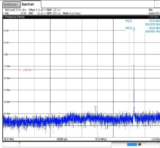
Band5-1.4MHz-16QAM-20525-1RB#0- Range1:30~1000MHz
