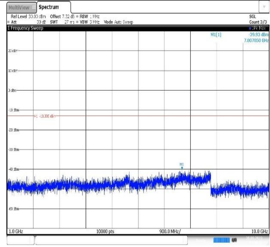
Band5-3MHz-16QAM-20635-1RB#0- Range2:1000~10000MHz
