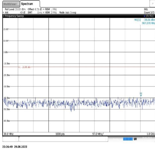
Band4-10MHz-QPSK-20175-1RB#0- Range1:30~1000MHz
