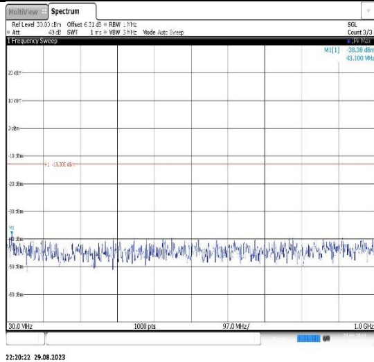
Band4-3MHz-16QAM-19965-1RB#0- Range1:30~1000MHz
