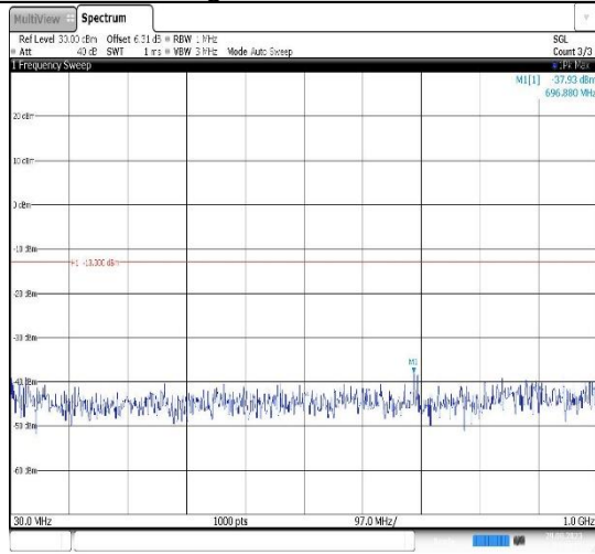
Band4-15MHz-16QAM-20175-1RB#0- Range1:30~1000MHz
