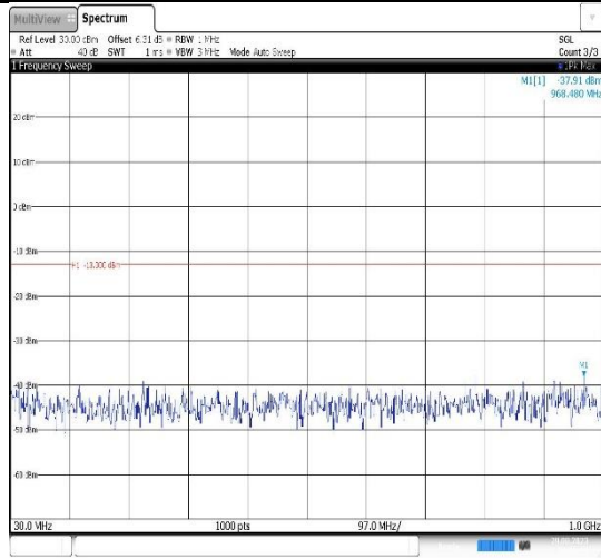
Band4-5MHz-16QAM-19975-1RB#0- Range1:30~1000MHz
