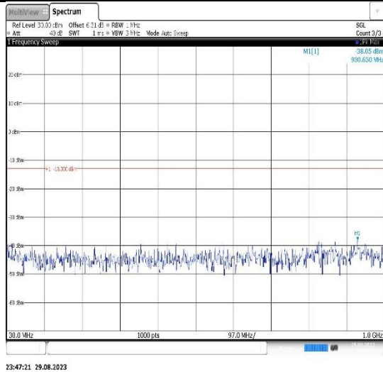
Band5-1.4MHz-QPSK-20407-1RB#0- Range1:30~1000MHz
