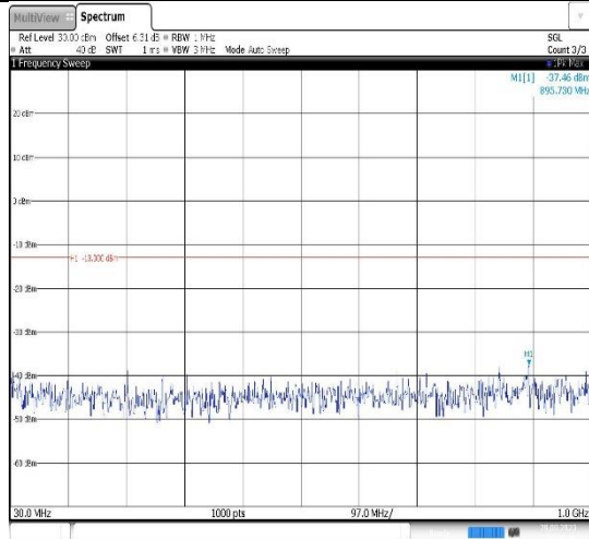
Band4-1.4MHz-16QAM-19957-1RB#0- Range1:30~1000MHz
