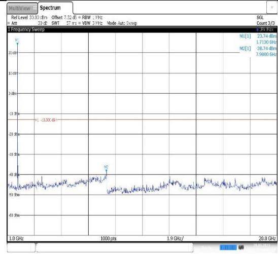
Band4-15MHz-16QAM-20025-1RB#0- Range2:1000~20000MHz
