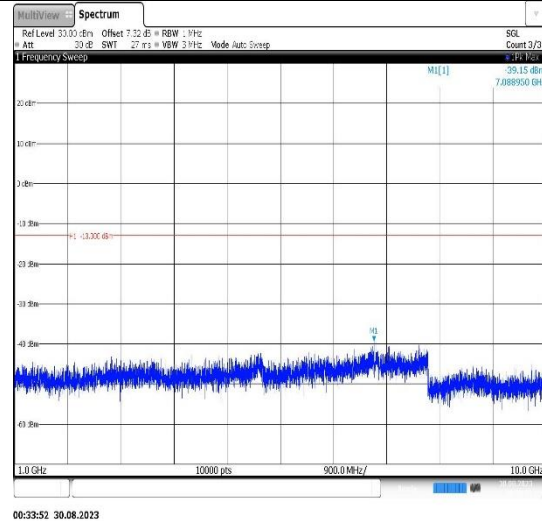
Band5-1.4MHz-QPSK-20643-1RB#0- Range2:1000~10000MHz
