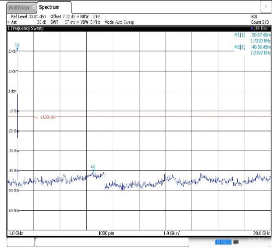
Band4-10MHz-16QAM-20175-1RB#0- Range2:1000~20000MHz
