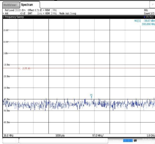
Band4-15MHz-QPSK-20175-1RB#0- Range1:30~1000MHz
