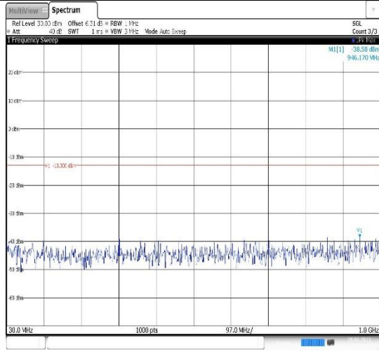
Band4-10MHz-16QAM-20175-1RB#0- Range1:30~1000MHz
