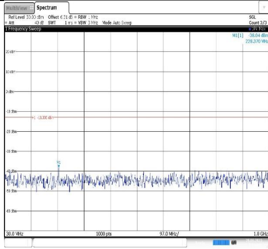
Band4-15MHz-16QAM-20025-1RB#0- Range1:30~1000MHz
