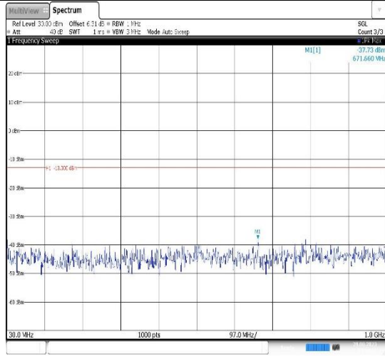
Band4-20MHz-16QAM-20175-1RB#0- Range1:30~1000MHz
