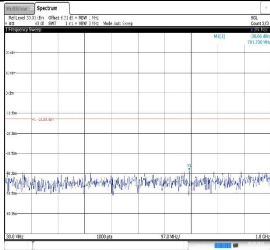
Band4-1.4MHz-16QAM-19957-1RB#0- Range1:30~1000MHz
