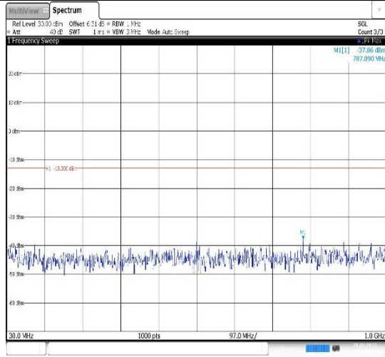
Band4-1.4MHz-QPSK-20175-1RB#0- Range1:30~1000MHz
