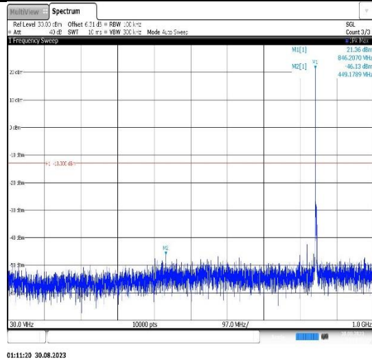
Band5-5MHz-QPSK-20425-1RB#0- Range1:30~1000MHz
