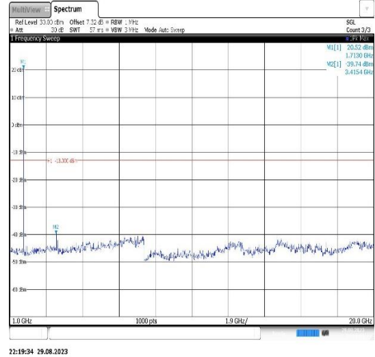
Band4-3MHz-16QAM-20175-1RB#0- Range2:1000~20000MHz
