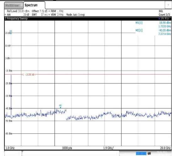
Band4-1.4MHz-16QAM-20175-1RB#0- Range2:1000~20000MHz
