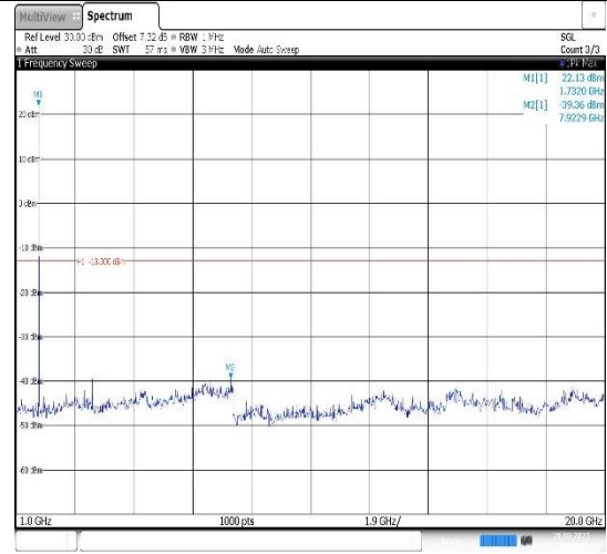
Band4-5MHz-16QAM-20175-1RB#0- Range2:1000~20000MHz
