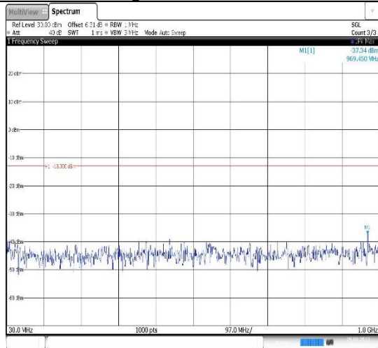
Band4-1.4MHz-16QAM-20175-1RB#0- Range1:30~1000MHz
