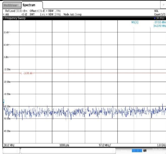
Band4-20MHz-16QAM-20050-1RB#0- Range1:30~1000MHz
