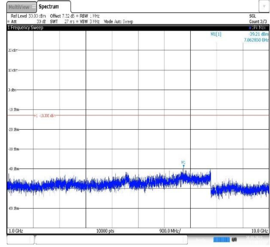
Band5-3MHz-16QAM-20525-1RB#0- Range2:1000~10000MHz
