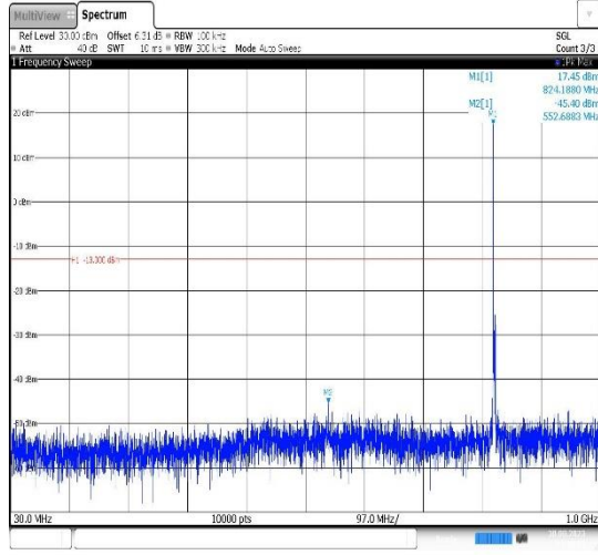
Band5-3MHz-16QAM-20525-1RB#0- Range1:30~1000MHz
