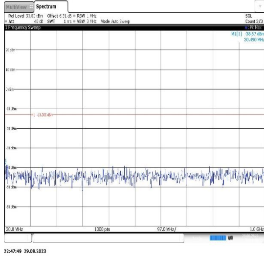
Band4-5MHz-QPSK-20175-1RB#0- Range1:30~1000MHz
