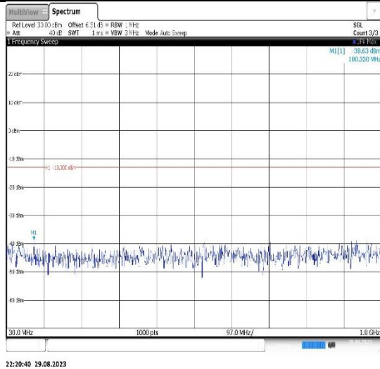
Band4-5MHz-QPSK-19975-1RB#0- Range1:30~1000MHz
