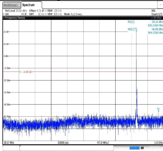
Band5-3MHz-QPSK-20525-1RB#0- Range1:30~1000MHz
