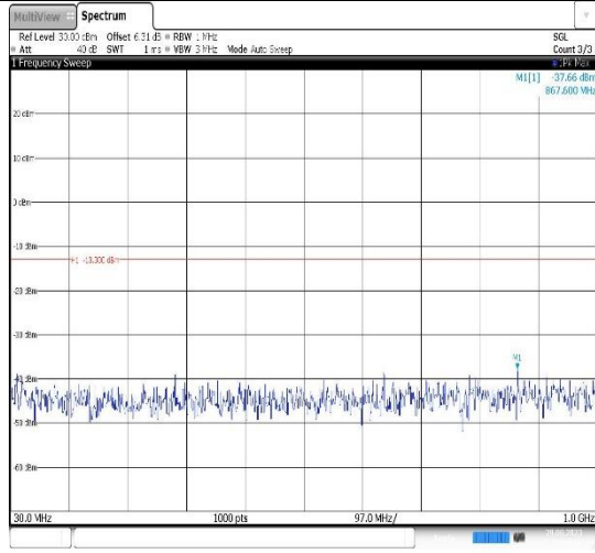
Band4-3MHz-QPSK-20385-1RB#0- Range1:30~1000MHz
