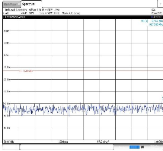
Band4-10MHz-16QAM-20000-1RB#0- Range1:30~1000MHz
