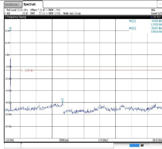
Band4-20MHz-16QAM-20175-1RB#0- Range2:1000~20000MHz
