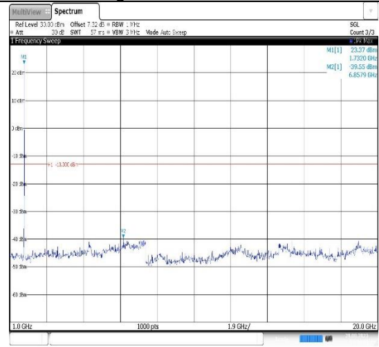
Band4-15MHz-16QAM-20175-1RB#0- Range2:1000~20000MHz
