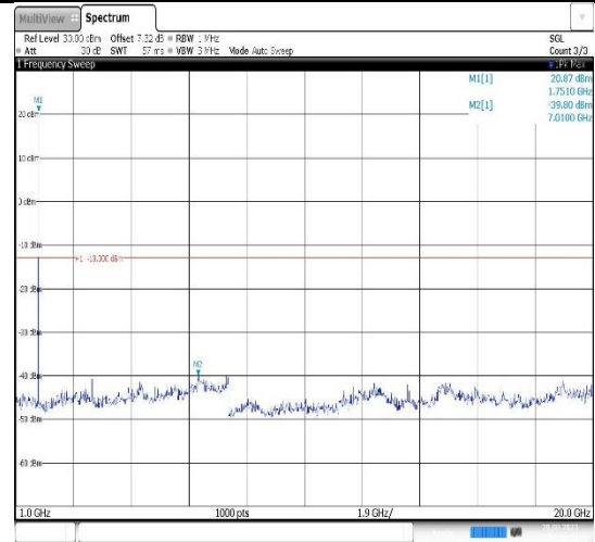
Band4-1.4MHz-16QAM-19957-1RB#0- Range2:1000~20000MHz
