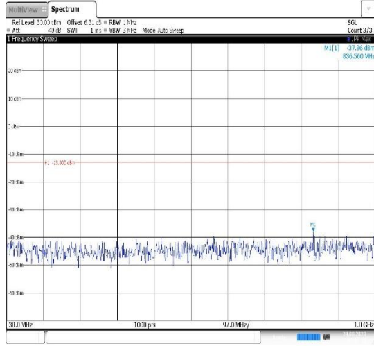
Band4-1.4MHz-QPSK-19957-1RB#0- Range1:30~1000MHz
