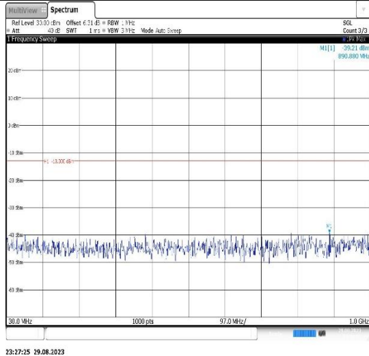
Band4-10MHz-QPSK-20350-1RB#0- Range1:30~1000MHz
