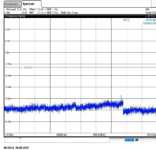
Band5-1.4MHz-QPSK-20525-1RB#0- Range2:1000~10000MHz
