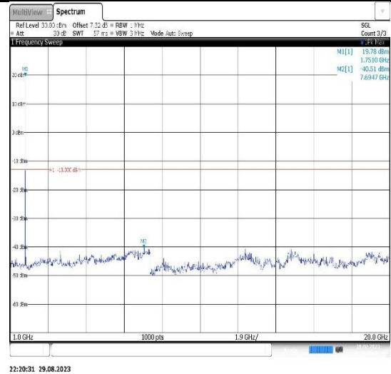
Band4-3MHz-16QAM-19965-1RB#0- Range2:1000~20000MHz
