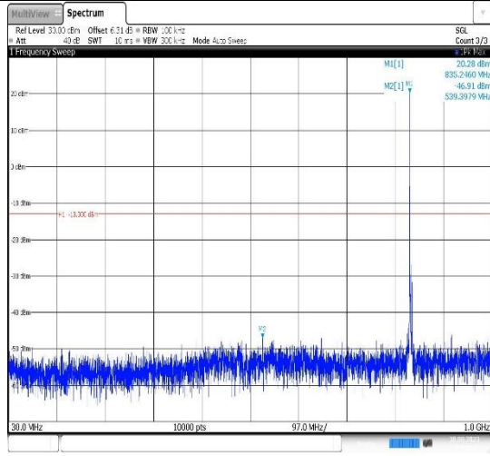
Band5-3MHz-16QAM-20635-1RB#0- Range1:30~1000MHz
