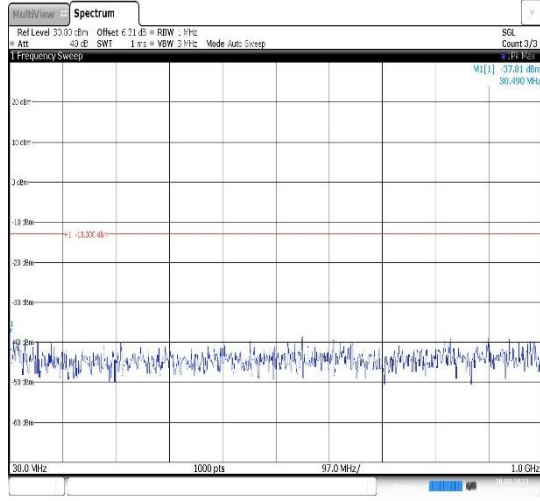
Band4-3MHz-QPSK-20175-1RB#0- Range1:30~1000MHz
