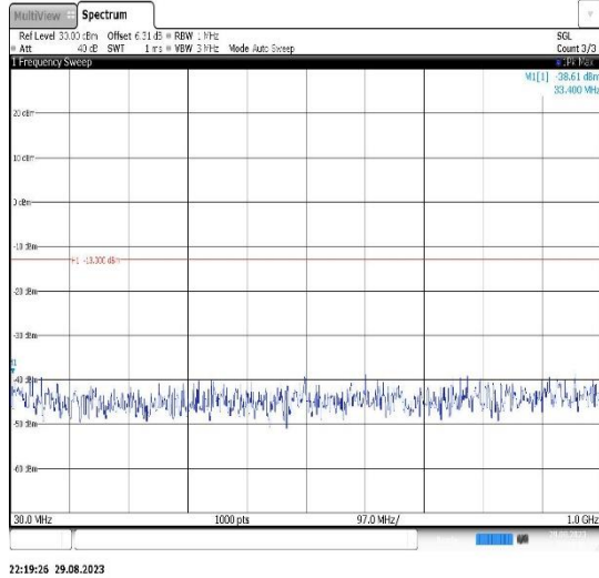
Band4-3MHz-16QAM-20175-1RB#0- Range1:30~1000MHz
