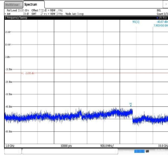
Band5-1.4MHz-16QAM-20525-1RB#0- Range2:1000~10000MHz
