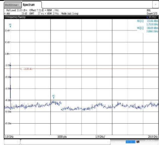
Band4-10MHz-16QAM-20000-1RB#0- Range2:1000~20000MHz
