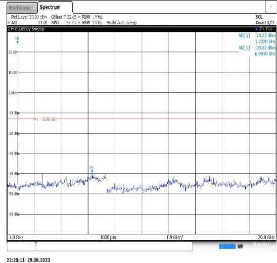
Band4-3MHz-16QAM-20385-1RB#0- Range2:1000~20000MHz
