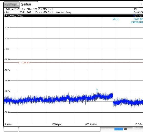
Band5-1.4MHz-16QAM-20407-1RB#0- Range2:1000~10000MHz
