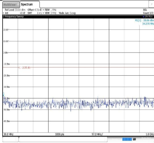
Band4-15MHz-QPSK-20025-1RB#0- Range1:30~1000MHz
