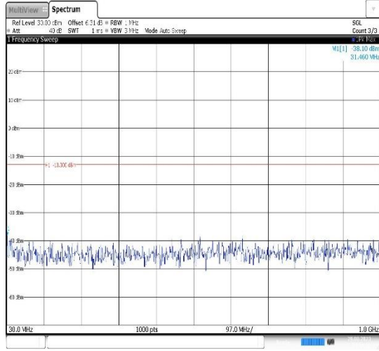
Band4-20MHz-QPSK-20050-1RB#0- Range1:30~1000MHz
