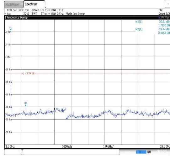
Band4-20MHz-16QAM-20050-1RB#0- Range2:1000~20000MHz
