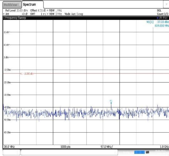
Band4-5MHz-16QAM-20175-1RB#0- Range1:30~1000MHz
